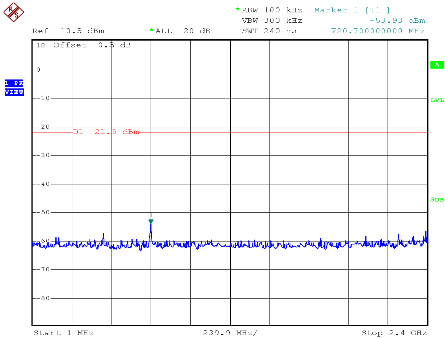
802.11g, Highest Channel, Plot A
