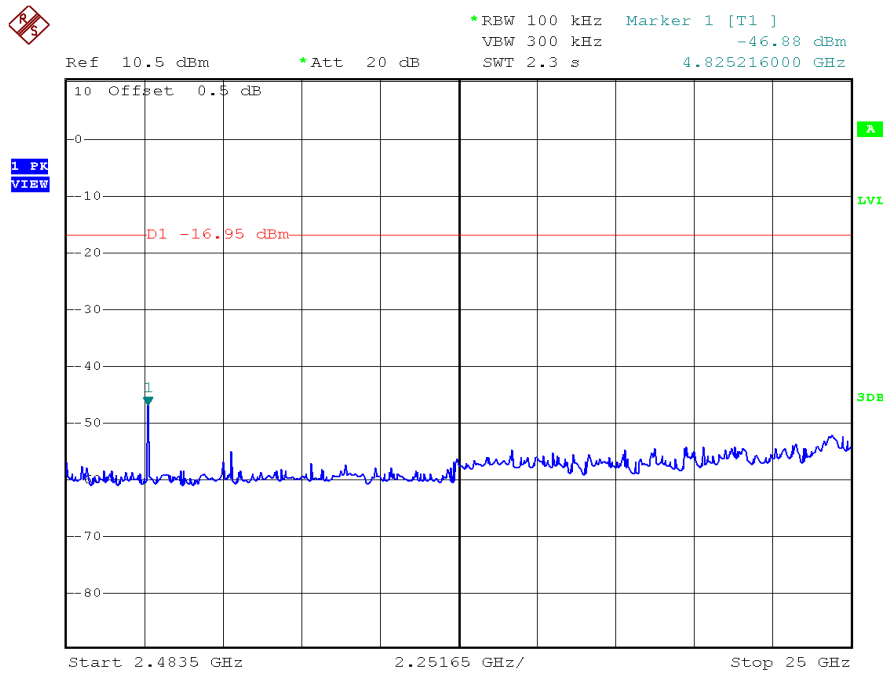
802.11b, Lowest Channel, Plot B
