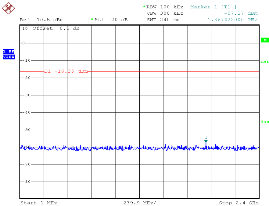
802.11b, Middle Channel, Plot A
