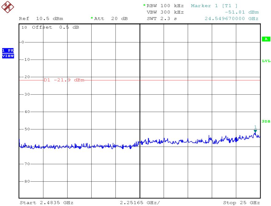
802.11g, Highest Channel, Plot B
