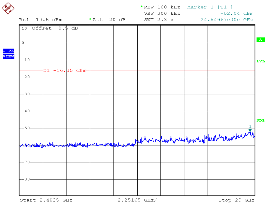
802.11b, Middle Channel, Plot B
