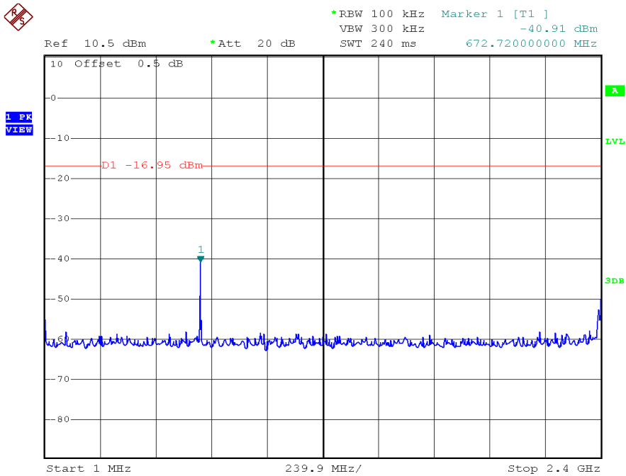
802.11b, Lowest Channel, Plot A
