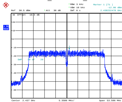
n40_2437MHz_Chain 0
