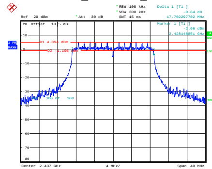
n20_2437MHz_Chain 0
