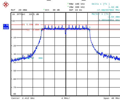
n20_2412MHz_Chain 0
