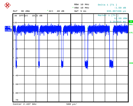
n40_2437MHz_Chain 0
