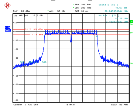
n40_2422MHz_Chain 0
