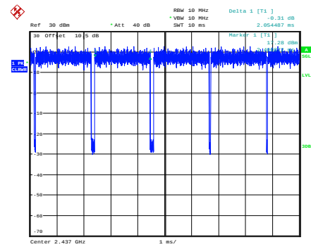
g_2437MHz_Chain 0
