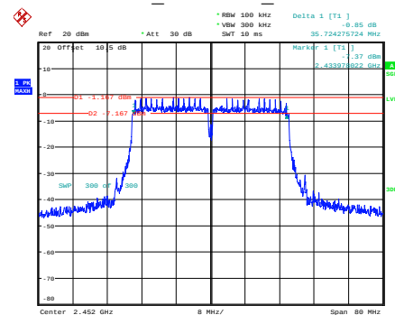
n40_2452MHz_Chain 0
