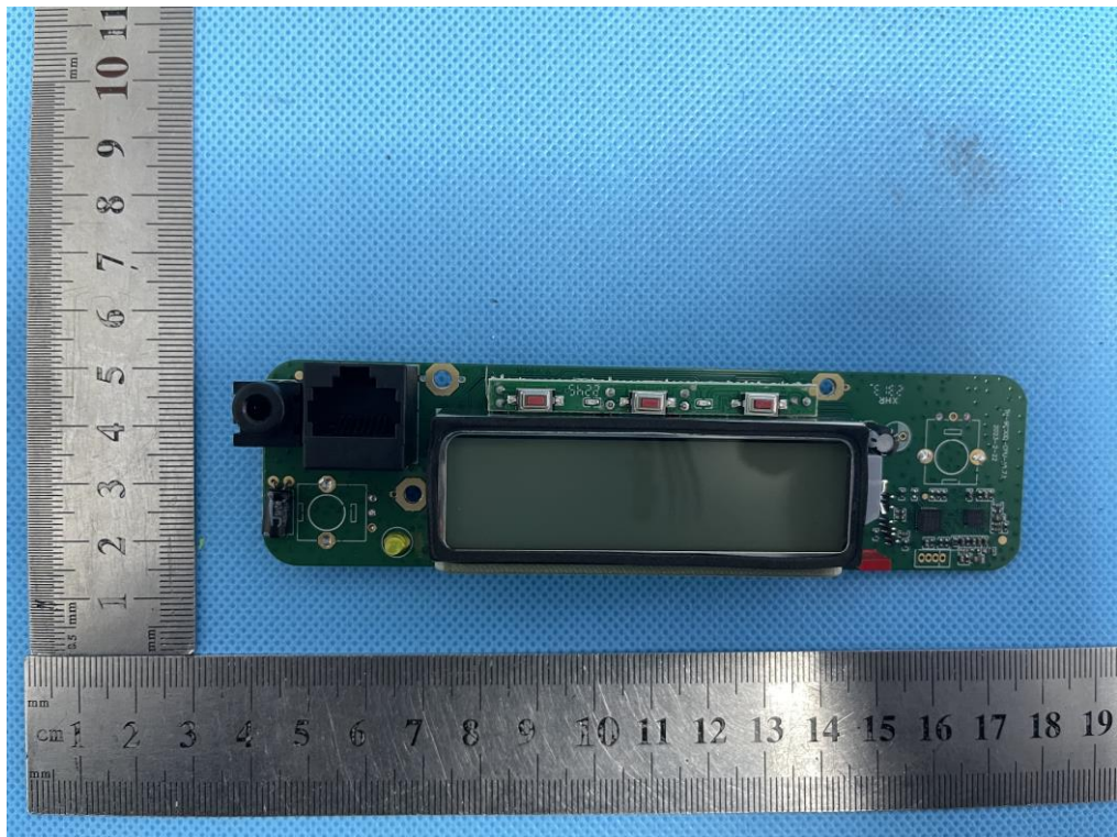
INTERNAL VIEW OF INTERNAL TRANSMITTER (FIGURE 3)
