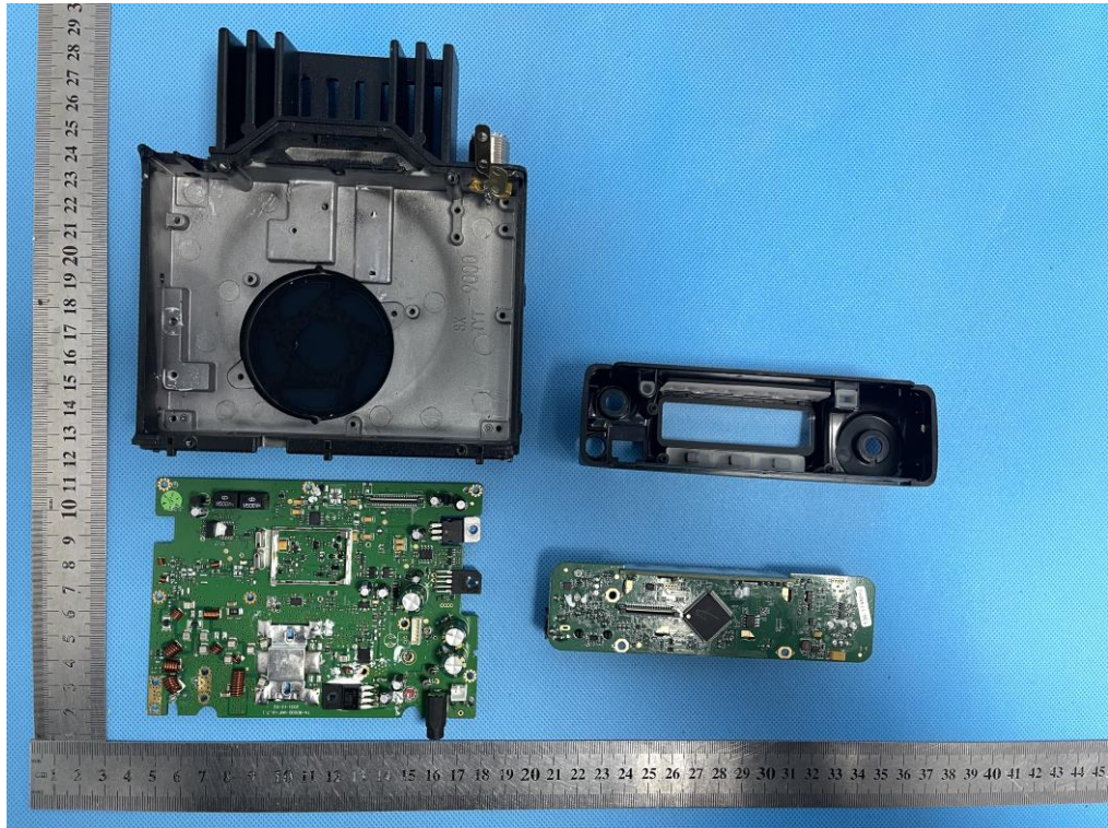
INTERNAL VIEW OF INTERNAL TRANSMITTER (FIGURE 1)
