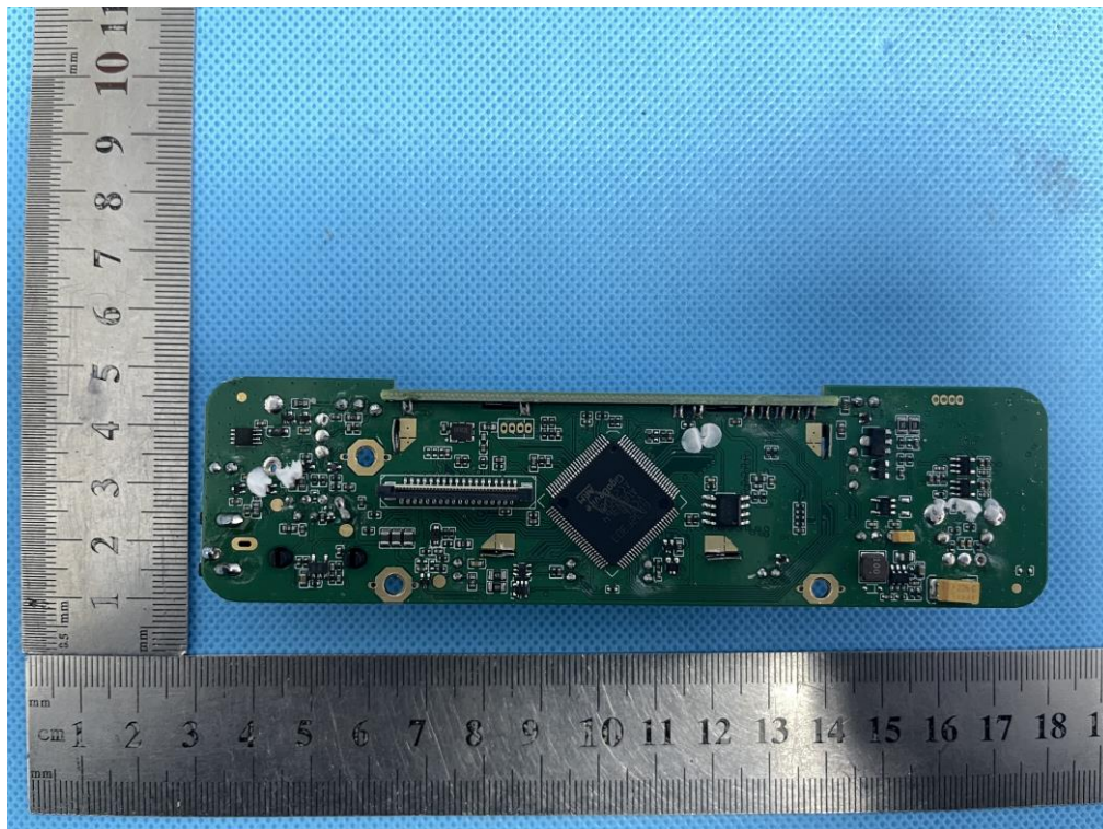
INTERNAL VIEW OF INTERNAL RECEIVER (FIGURE 2)
