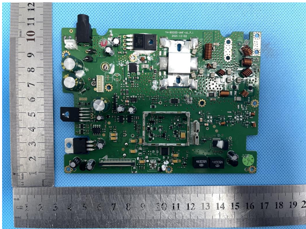
INTERNAL VIEW OF INTERNAL TRANSMITTER (FIGURE 5)
