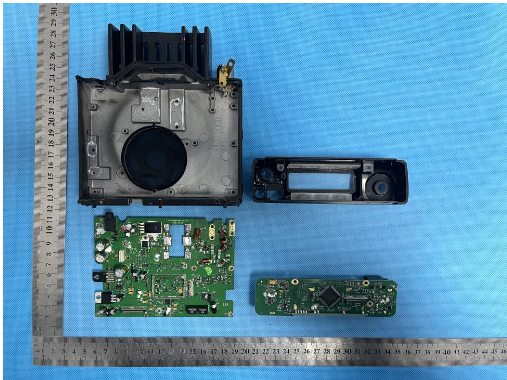
OPEN VIEW OF INTERNAL RECEIVER (FIGURE 2)
