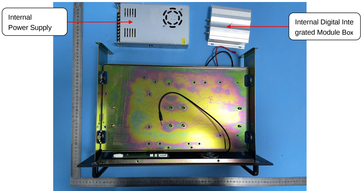
OPEN VIEW OF EUT (FIGURE 4)
