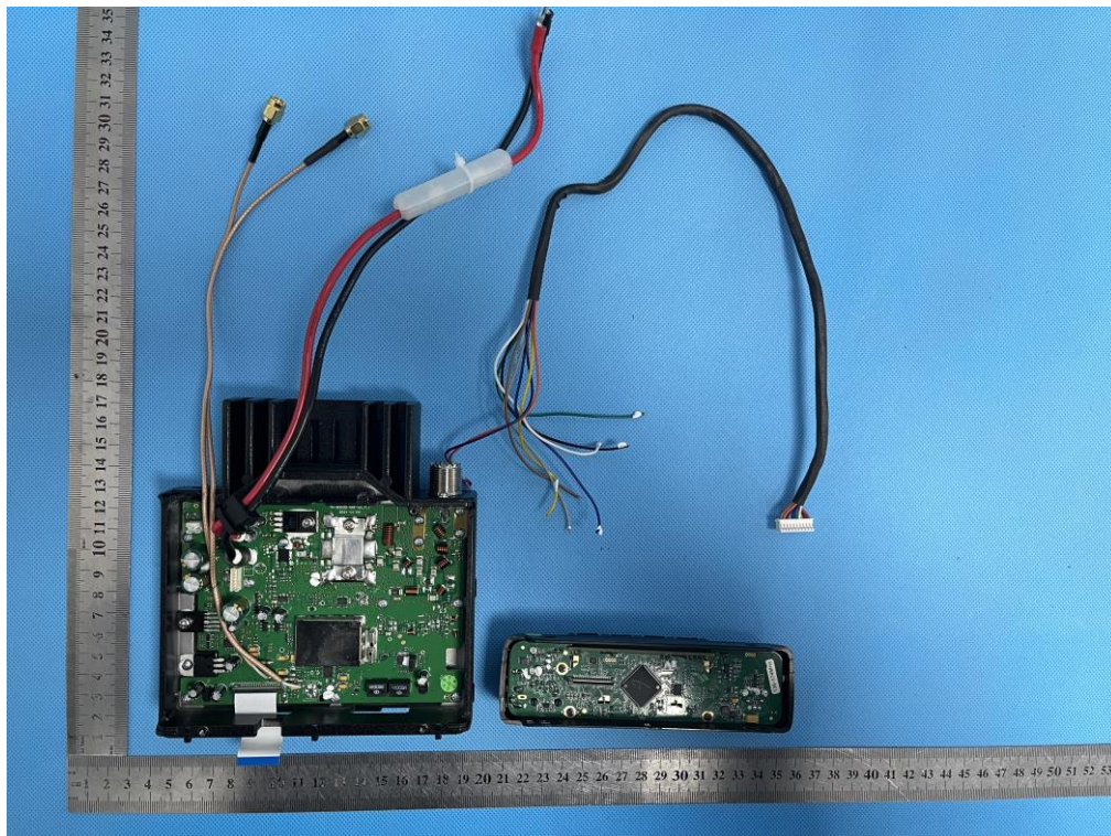
OPEN VIEW OF INTERNAL TRANSMITTER (FIGURE 2)
