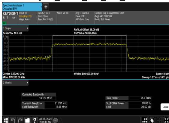
B66_N41(20M)_CP-OFDM_16 QAM_Outer_Full_Mid_CH
