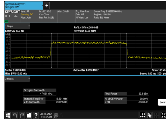
B66_N41(50M)_CP-OFDM_256 QAM_Outer_Full_Mid_CH
