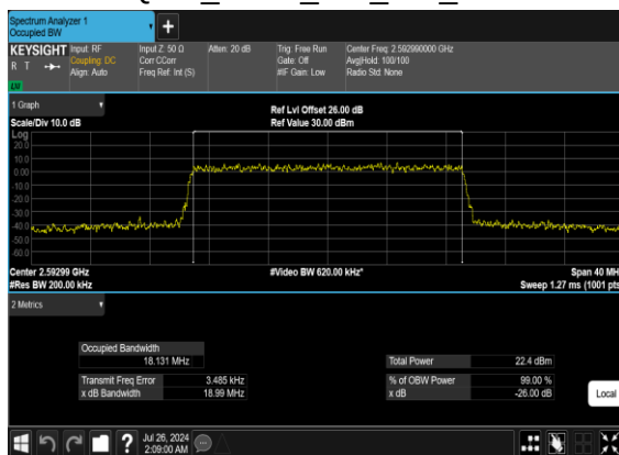
B66_N41(20M)_CP-OFDM_256 QAM_Outer_Full_Mid_CH
