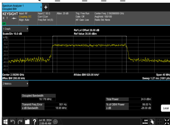
B66_N41(20M)_CP-OFDM_64 QAM_Outer_Full_Mid_CH
