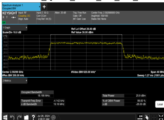
B66_N41(20M)_CP- OFDM_QPSK_Outer_Full_Mid_CH
