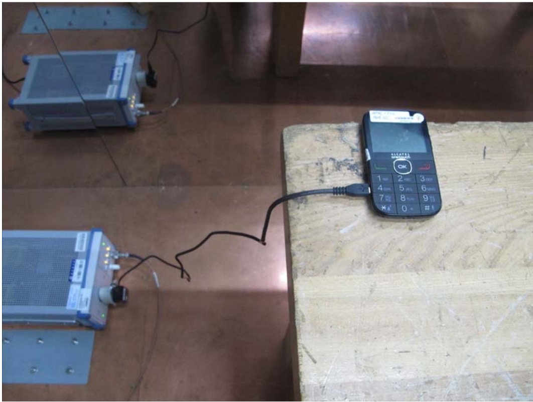
Conducted emission
