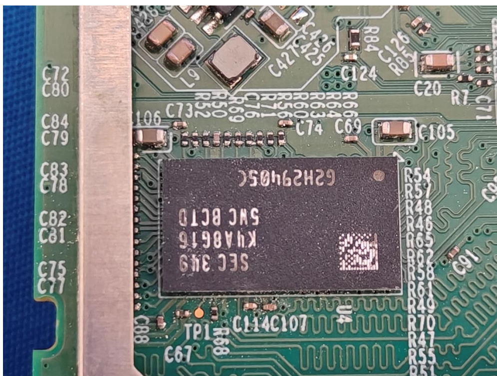
(26) EUT Photo
