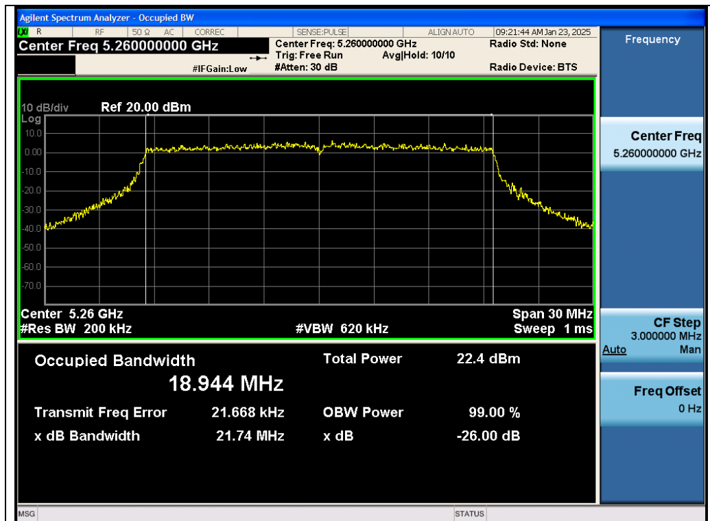
Test_Graph_802.11ax20_Chain B_5260_MCS0_OBW
