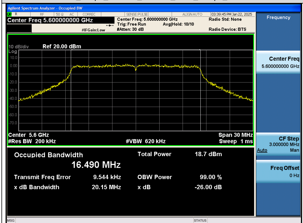
Test_Graph_802.11a_Chain A_5600_6Mbps_OBW
