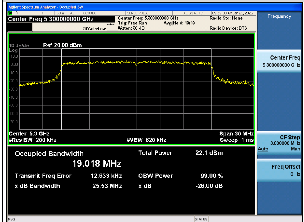
Test_Graph_802.11ax20_Chain B_5300_MCS0_OBW
