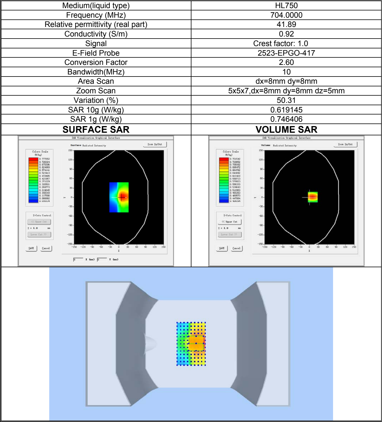
Plot 5: LTE BAND 12, Low channel (Body-worn, Front Side) Product Description: UF1 USB WiFi Dongle Test Date: 2024-07-19
