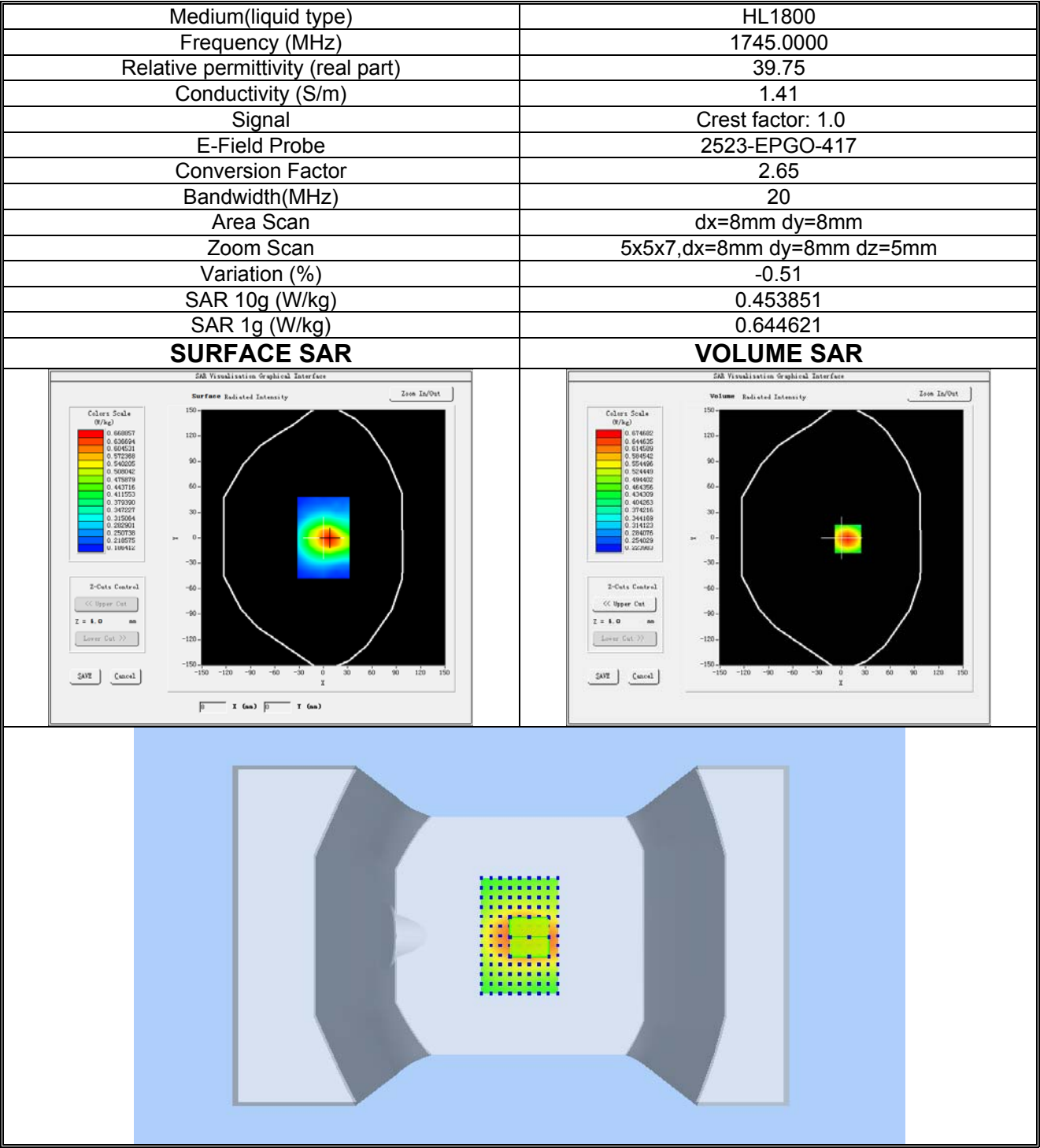
Plot 3: LTE BAND 4, High channel (Body-worn, Back Side) Product Description: UF1 USB WiFi Dongle Test Date: 2024-07-20
