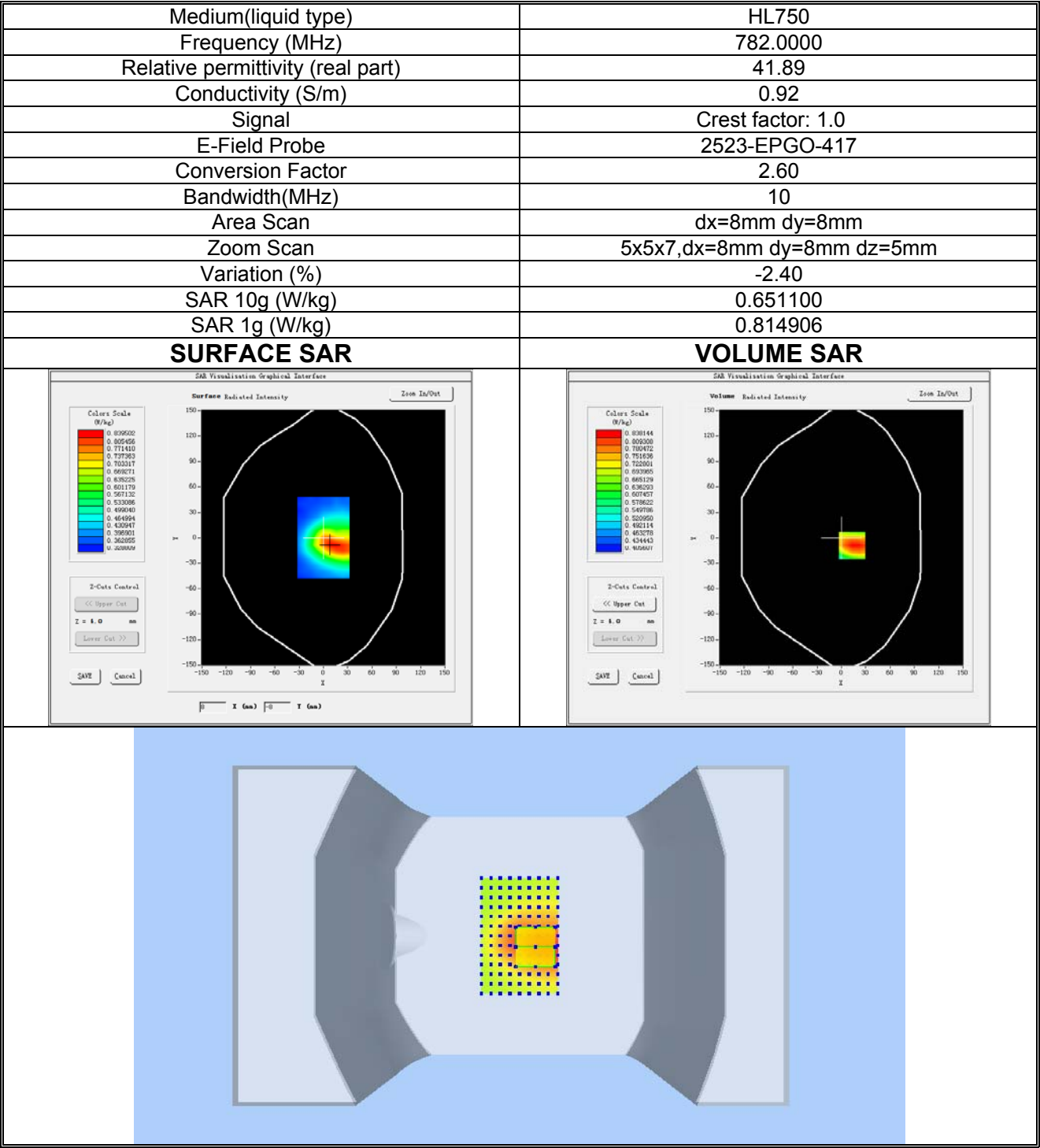
Plot 6: LTE BAND 13, Low channel (Body-worn, Back Side) Product Description: UF1 USB WiFi Dongle Test Date: 2024-07-19
