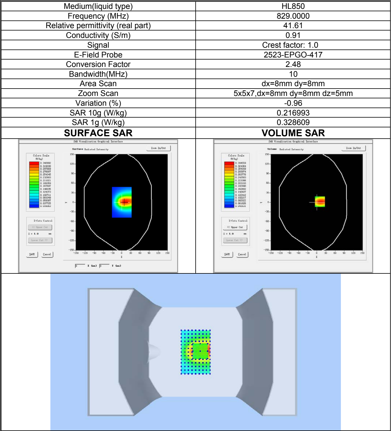
Plot 4: LTE BAND 5, Low channel (Body-worn, Front Side) Product Description: UF1 USB WiFi Dongle Test Date: 2024-07-19
