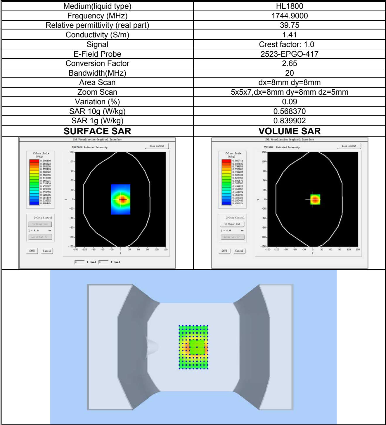
Plot 7: LTE BAND 66, Middle channel (Body-worn, Back Side) Product Description: UF1 USB WiFi Dongle Test Date: 2024-07-20
