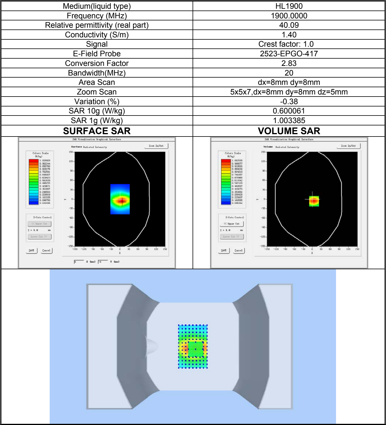
Plot 2: LTE BAND 2, High channel (Body-worn, Front Side) Product Description:UF1 USB WiFi Dongle Test Date: 2024-07-20
