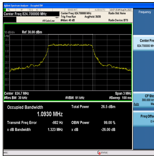
Band26-1.4MHz-QPSK-26797-6RB#0-1.0930
