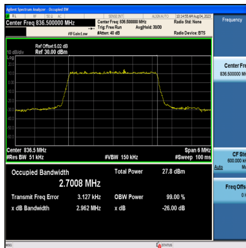
Band26-3MHz-QPSK-26915-15RB#0-2.7008
