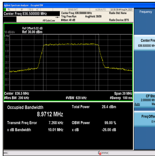
Band26-10MHz-QPSK-26915-50RB#0-8.9712
