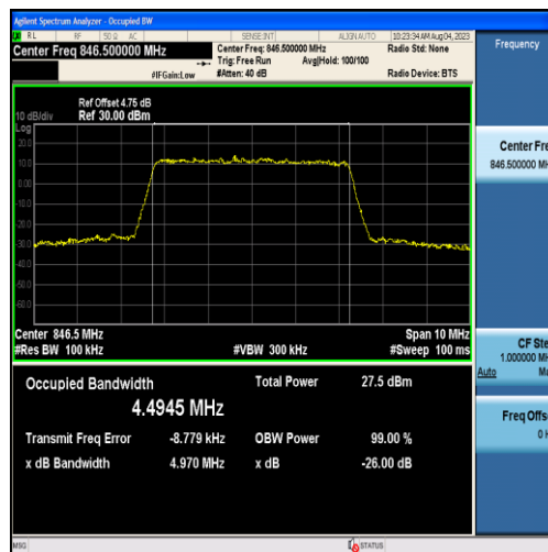
Band26-5MHz-16QAM-27015-25RB#0-4.4945
