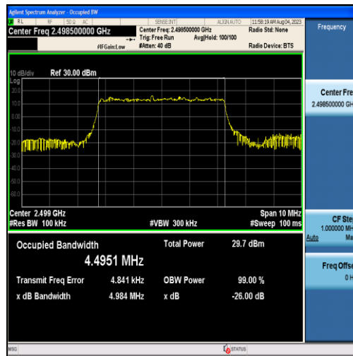
Band41-5MHz-QPSK-39675-25RB#0-4.4951
