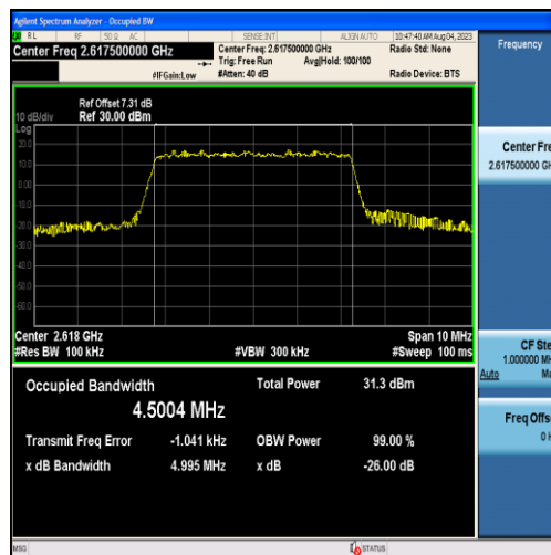
Band38-5MHz-QPSK-38225-25RB#0-4.5004
