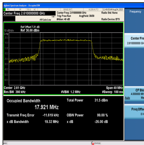
Band38-20MHz-QPSK-38150-100RB#0-17.921
