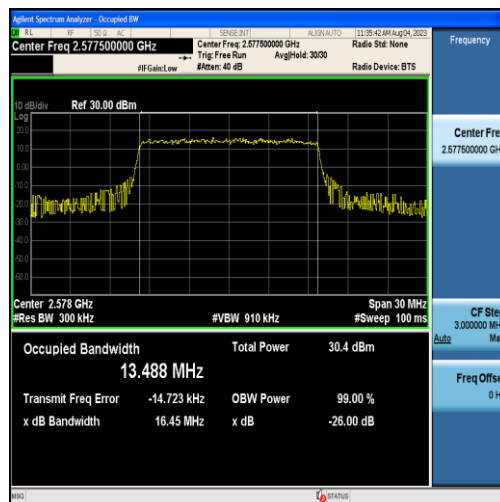
Band38-15MHz-16QAM-37825-75RB#0-13.488
