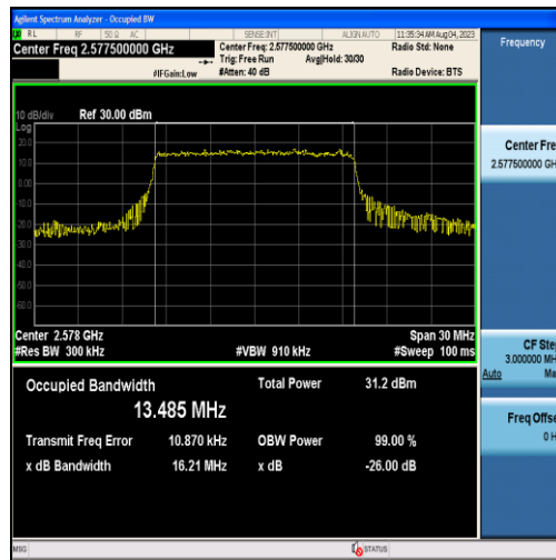
Band38-15MHz-QPSK-37825-75RB#0-13.485
