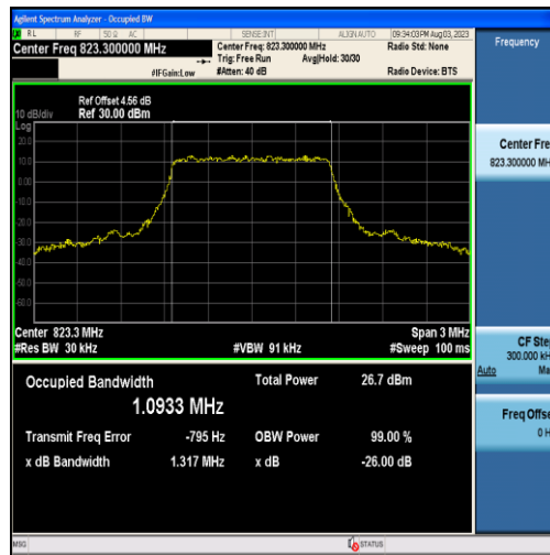
Band26-1.4MHz-QPSK-26783-6RB#0-1.0933
