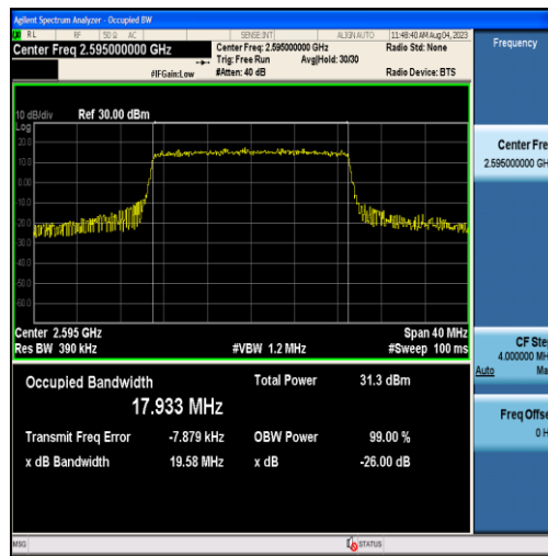
Band38-20MHz-QPSK-38000-100RB#0-17.933
