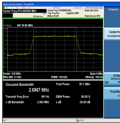
Band26-3MHz-16QAM-26740-15RB#0-2.6967
