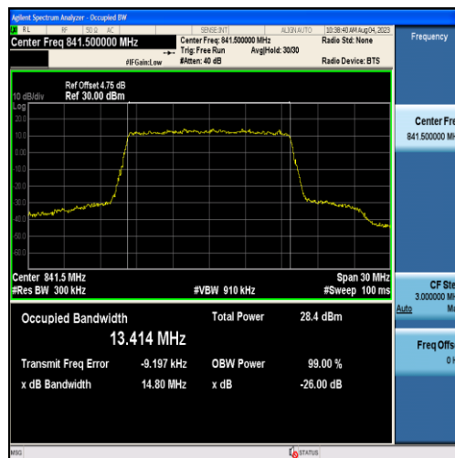
Band26-15MHz-QPSK-26965-75RB#0-13.414
