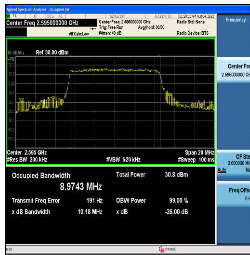
Band38-10MHz-QPSK-38000-50RB#0-8.9743
