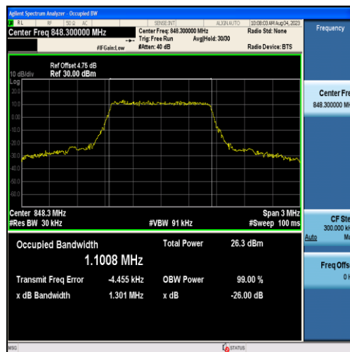
Band26-1.4MHz-16QAM-27033-6RB#0-1.1008
