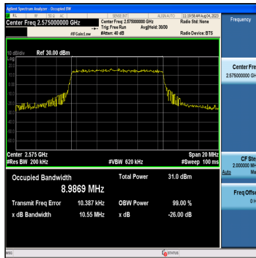
Band38-10MHz-QPSK-37800-50RB#0-8.9869
