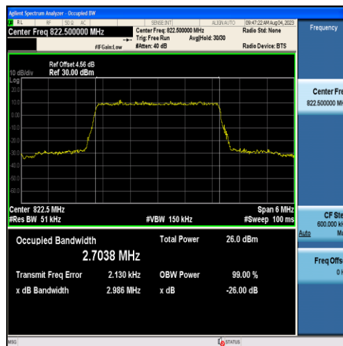
Band26-3MHz-16QAM-26775-15RB#0-2.7038
