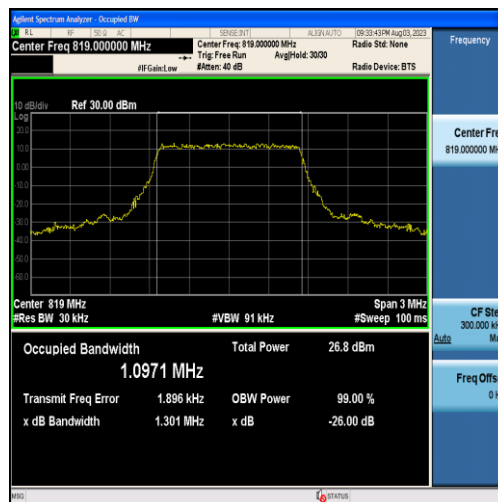
Band26-1.4MHz-QPSK-26740-6RB#0-1.0971
