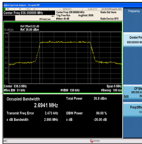
Band26-3MHz-16QAM-26915-15RB#0-2.6941
