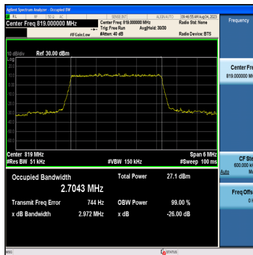
Band26-3MHz-QPSK-26740-15RB#0-2.7043
