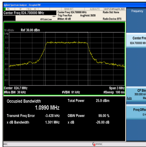
Band26-1.4MHz-16QAM-26797-6RB#0-1.0990
