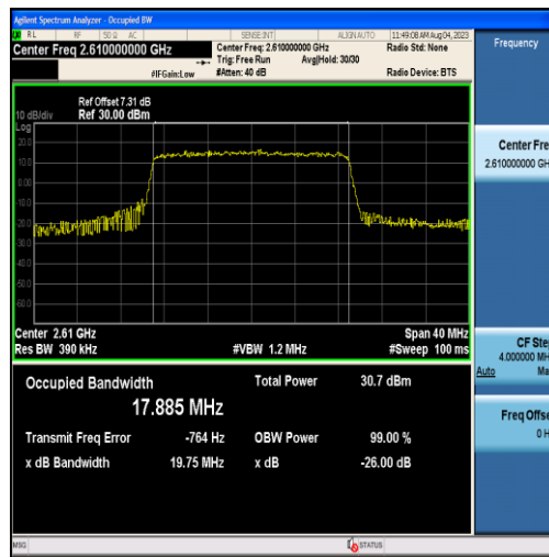
Band38-20MHz-16QAM-38150-100RB#0-17.885
