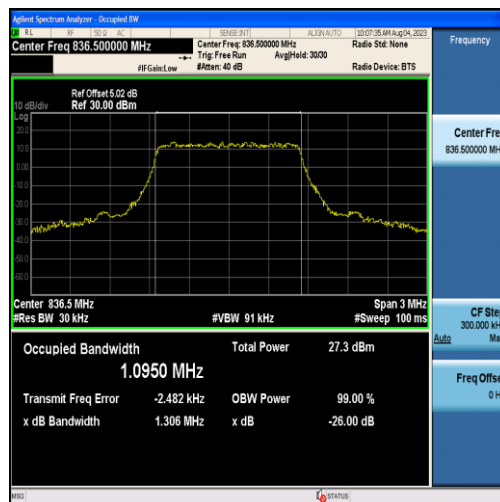
Band26-1.4MHz-QPSK-26915-6RB#0-1.0950
