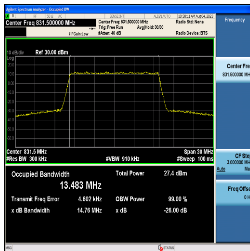
Band26-15MHz-16QAM-26865-75RB#0-13.483
