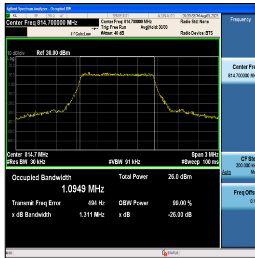
Band26-1.4MHz-16QAM-26697-6RB#0-1.0949
