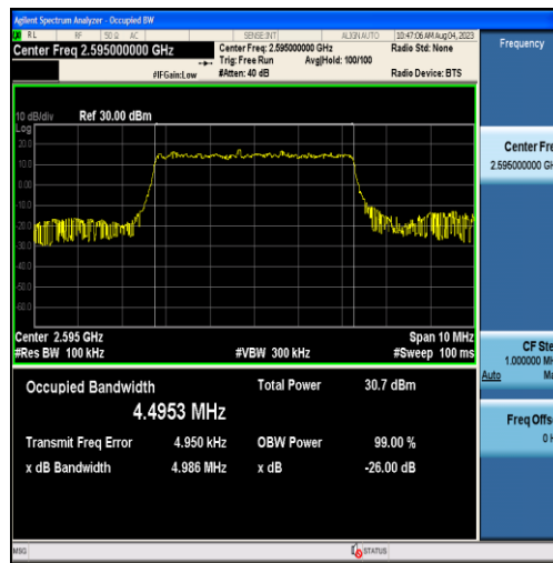
Band38-5MHz-QPSK-38000-25RB#0-4.4953
