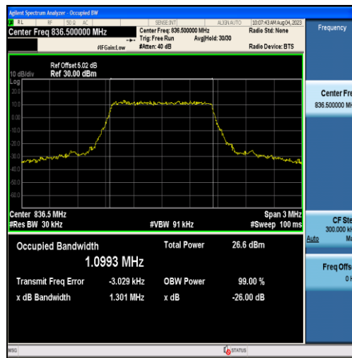
Band26-1.4MHz-16QAM-26915-6RB#0-1.0993
