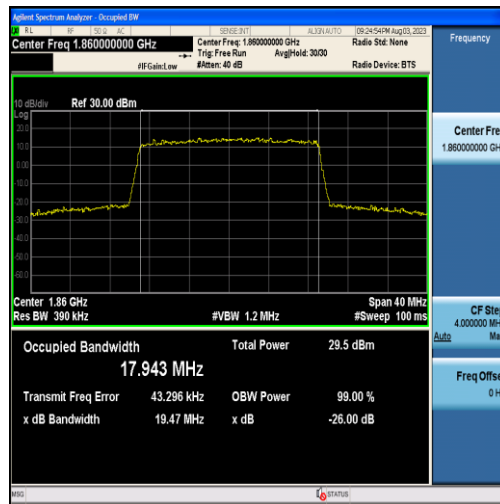
Band25-20MHz-16QAM-26140-100RB#0-17.943
