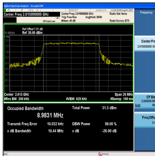
Band38-10MHz-QPSK-38200-50RB#0-8.9831
