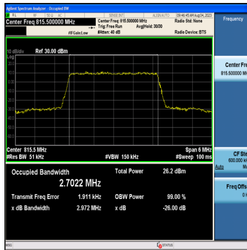
Band26-3MHz-16QAM-26705-15RB#0-2.7022
