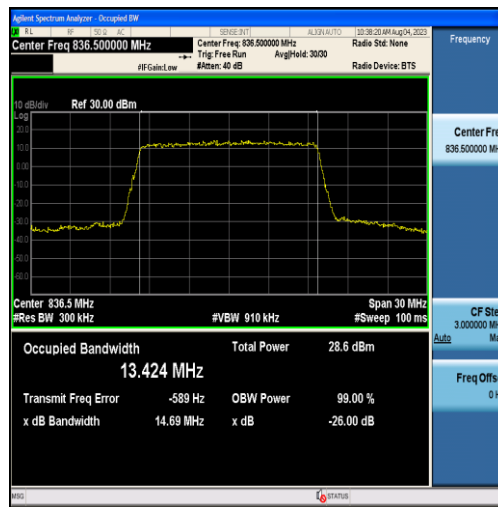
Band26-15MHz-QPSK-26915-75RB#0-13.424
