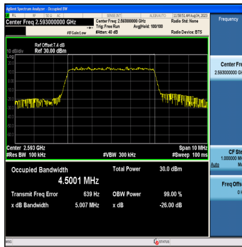
Band41-5MHz-QPSK-40620-25RB#0-4.5001
