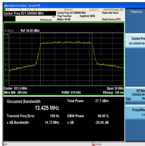
Band26-15MHz-QPSK-26765-75RB#0-13.425
