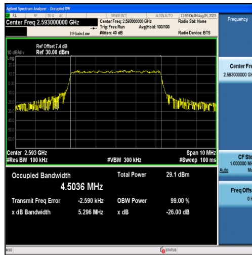
Band41-5MHz-16QAM-40620-25RB#0-4.5036
