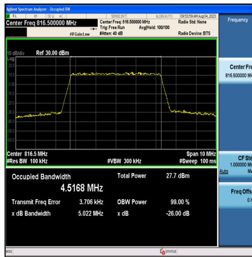
Band26-5MHz-QPSK-26715-25RB#0-4.5168
