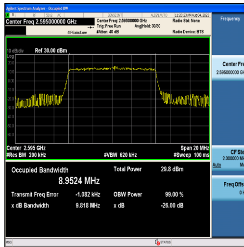
Band38-10MHz-16QAM-38000-50RB#0-8.9524
