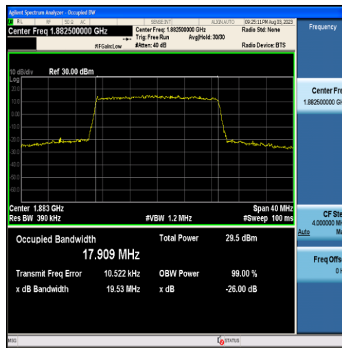
Band25-20MHz-16QAM-26365-100RB#0-17.909
