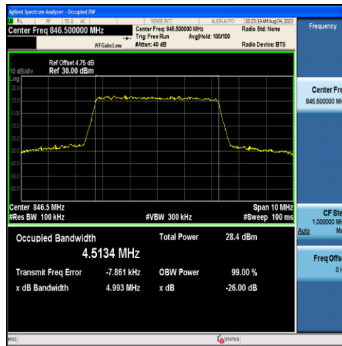
Band26-5MHz-QPSK-27015-25RB#0-4.5134
