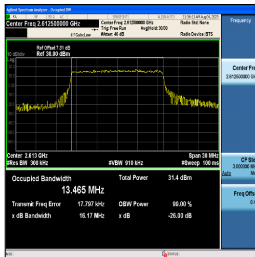
Band38-15MHz-QPSK-38175-75RB#0-13.465
