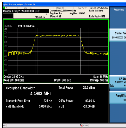
Band38-5MHz-16QAM-38000-25RB#0-4.4983
