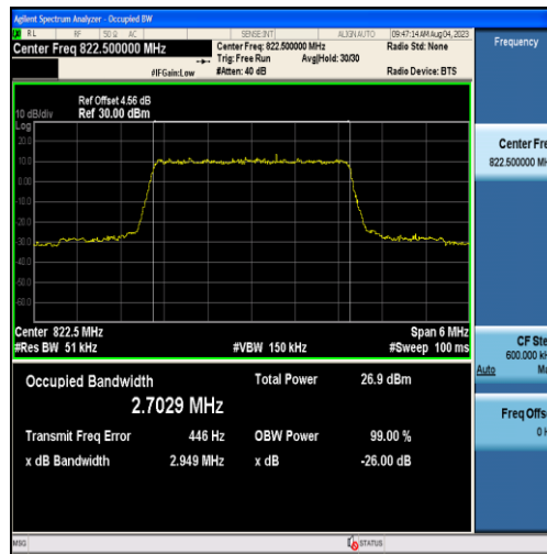
Band26-3MHz-QPSK-26775-15RB#0-2.7029
