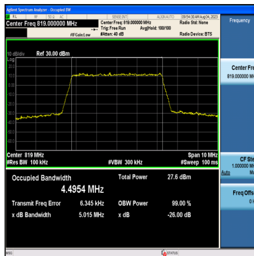
Band26-5MHz-QPSK-26740-25RB#0-4.4954
