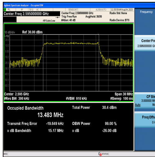
Band38-15MHz-16QAM-38000-75RB#0-13.483
