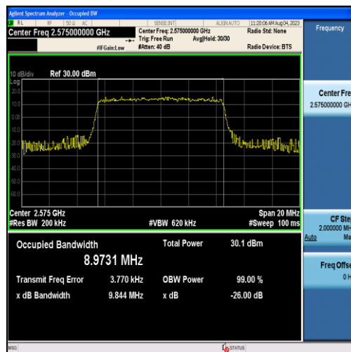
Band38-10MHz-16QAM-37800-50RB#0-8.9731
