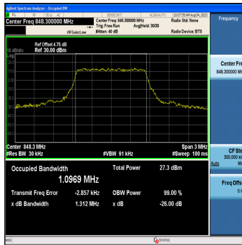
Band26-1.4MHz-QPSK-27033-6RB#0-1.0969
