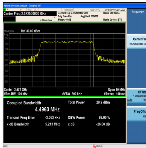
Band38-5MHz-16QAM-37775-25RB#0-4.4960
