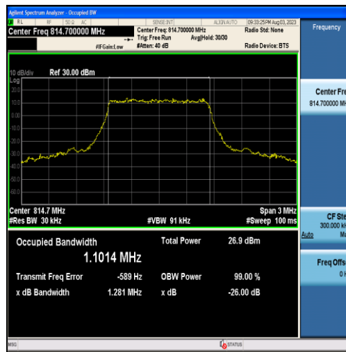
Band26-1.4MHz-QPSK-26697-6RB#0-1.1014
