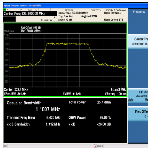
Band26-1.4MHz-16QAM-26783-6RB#0-1.1007
