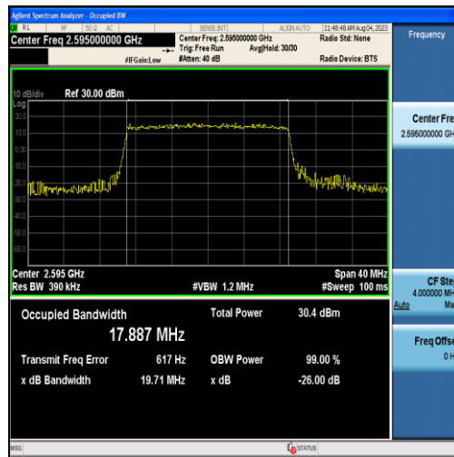
Band38-20MHz-16QAM-38000-100RB#0-17.887
