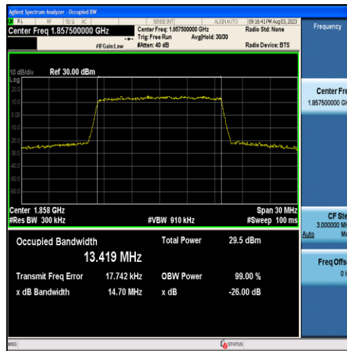
Band25-15MHz-16QAM-26115-75RB#0-13.419
