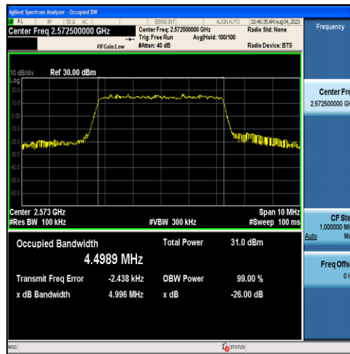
Band38-5MHz-QPSK-37775-25RB#0-4.4989
