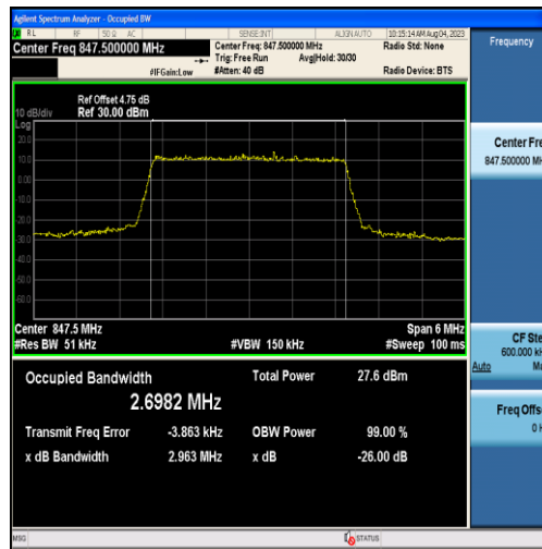
Band26-3MHz-QPSK-27025-15RB#0-2.6982
