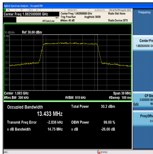
Band25-15MHz-QPSK-26365-75RB#0-13.433
