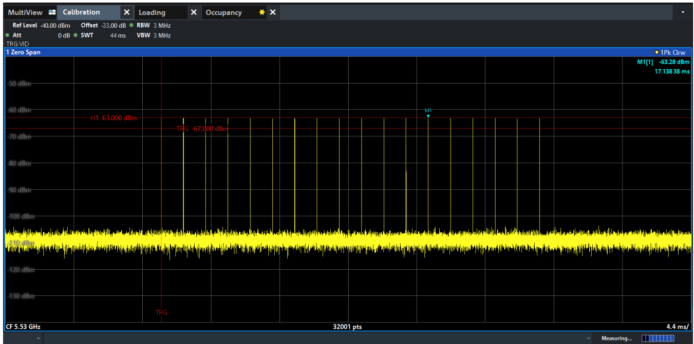
Figure 7-5. 5530MHz – Radar Pulse Type 0 (80MHz)
