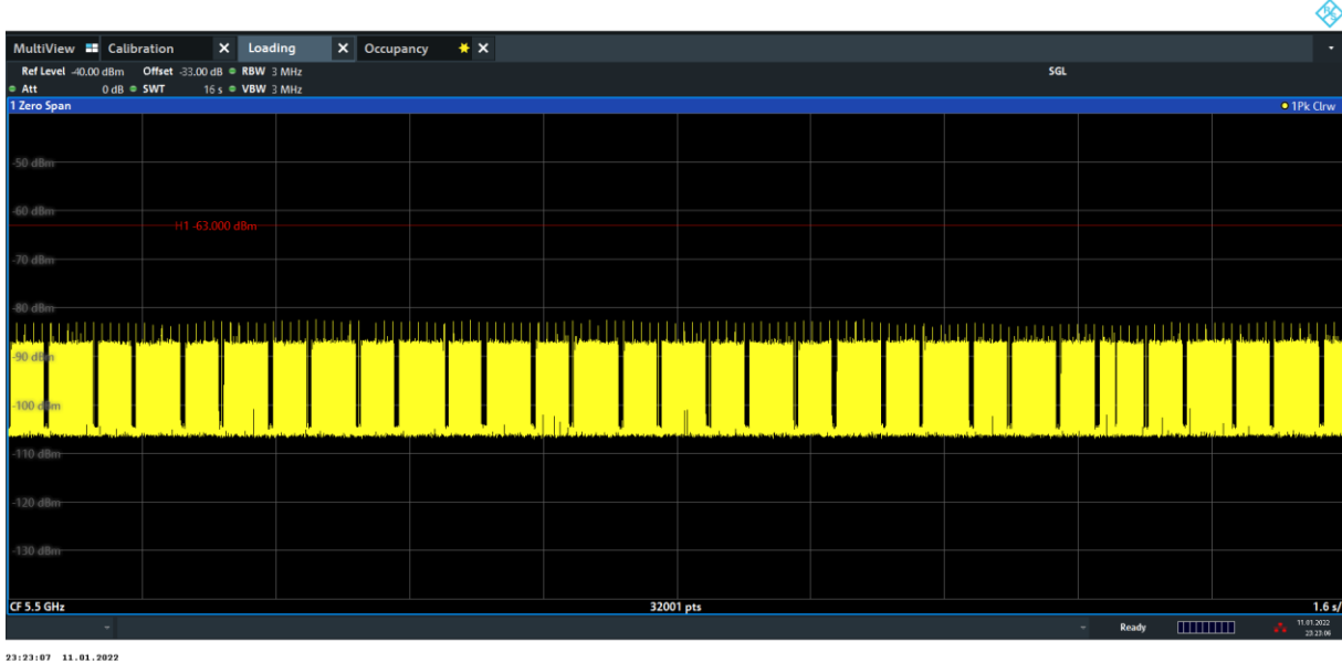
Figure 9-13. 5500MHz - Channel Loading - Mode 3 (20MHz)
