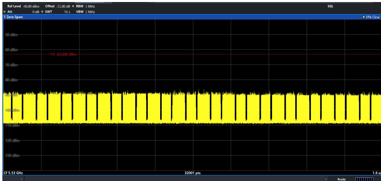
Figure 9-23. 5530MHz - Channel Loading - Mode 4 (80MHz)
