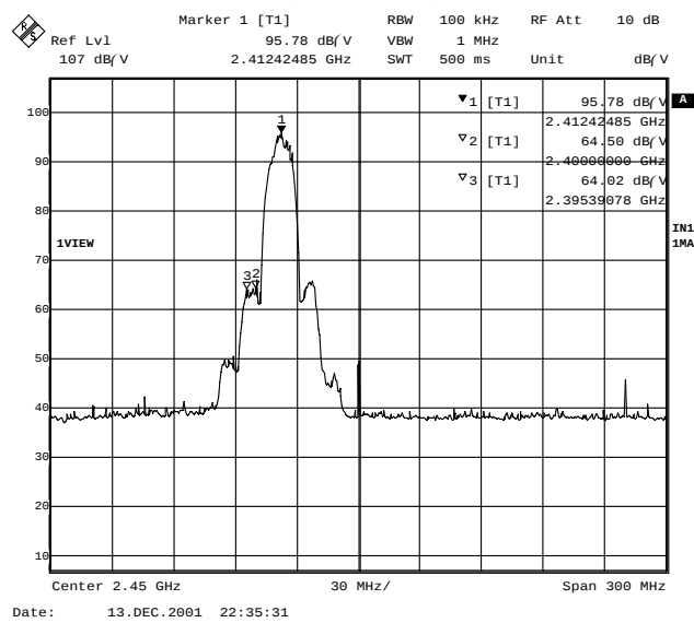
Figure Channel 1: (Vertical)
