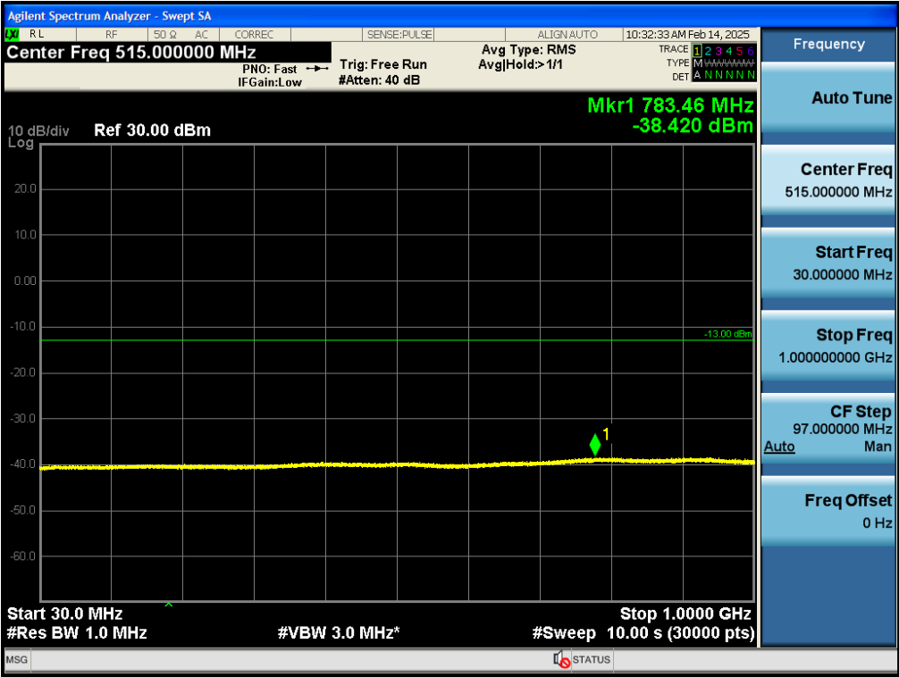
Test_Graph_bandGSM1900_1850.2MHz_Voice_30M_1G_TX
