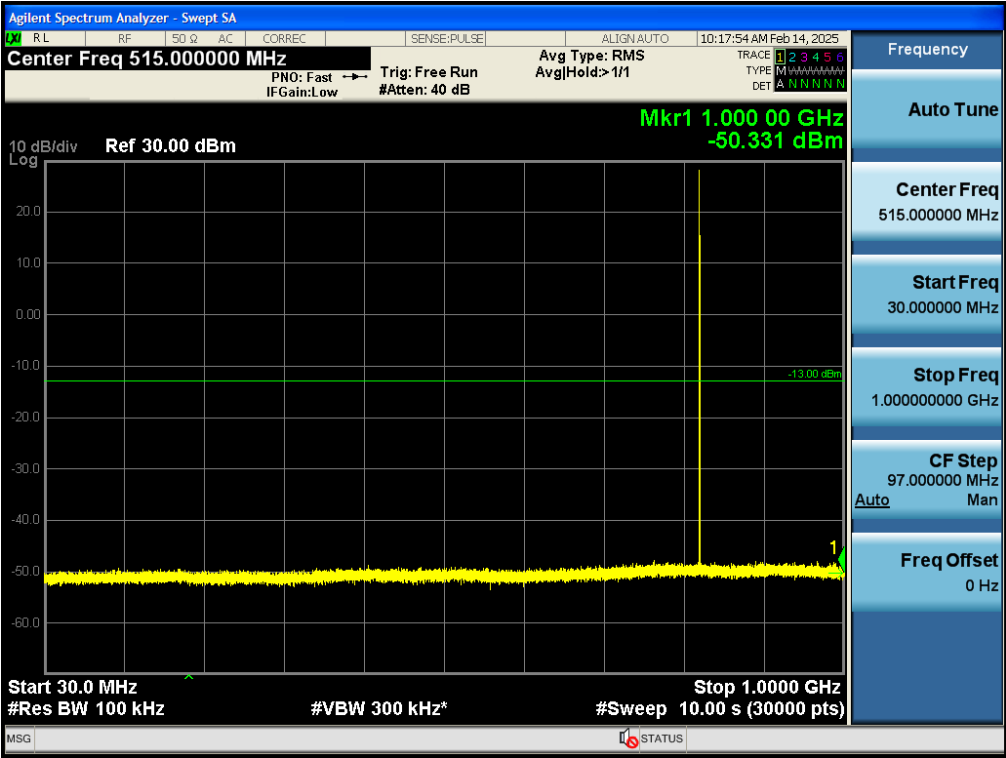
Test_Graph_bandGSM850_824.2MHz_GPRS 1Slot_30M_1G_TX
