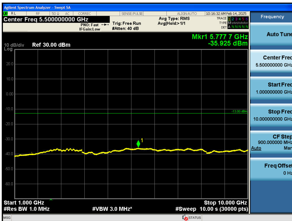
Test_Graph_bandGSM850_836.6MHz_Voice_1G_10G_TX
