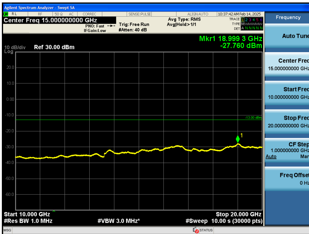
Test_Graph_bandGSM1900_1909.8MHz_Voice_10G_20G_TX
