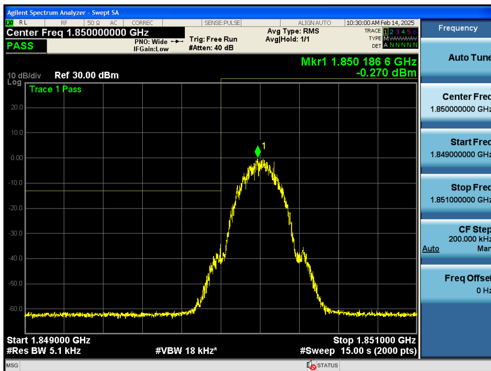
Test_Graph_bandGSM1900_1850.2MHz_Voice_Band edge
