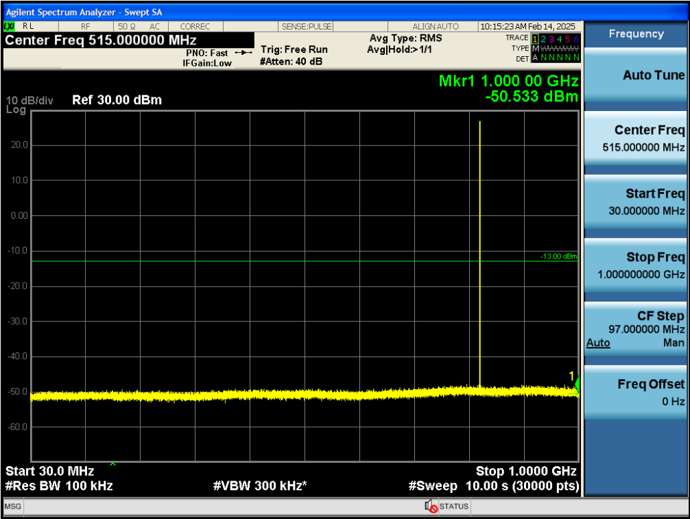
Test_Graph_bandGSM850_824.2MHz_Voice_30M_1G_TX
