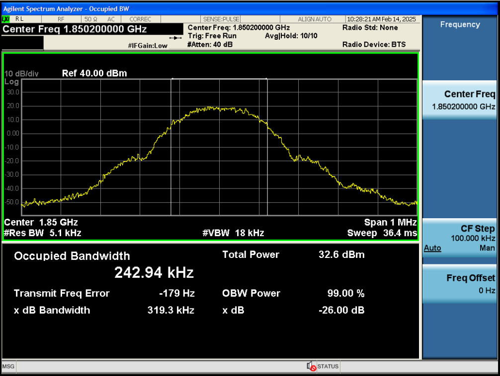
Test_Graph_bandGSM1900_1850.2MHz_GPRS 1Slot_OBW&EBW
