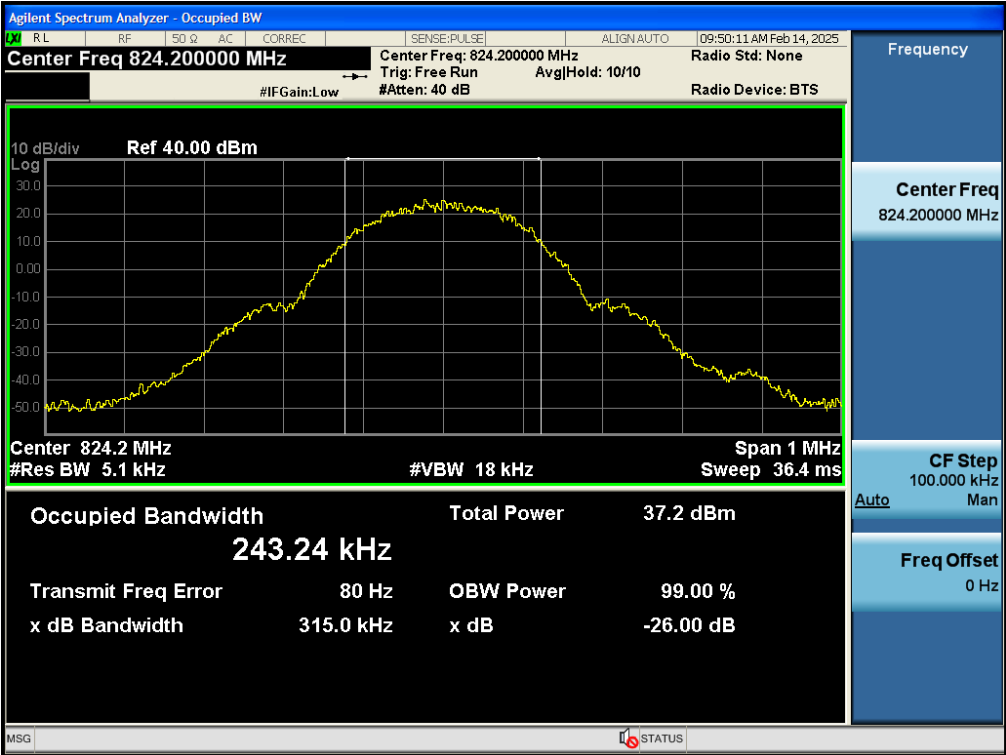
Test_Graph_bandGSM850_824.2MHz_GPRS 1Slot_OBW&EBW
