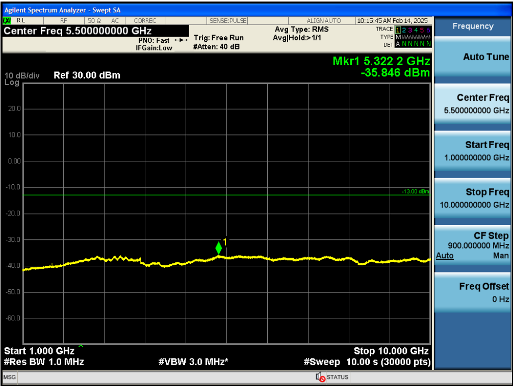
Test_Graph_bandGSM850_824.2MHz_Voice_1G_10G_TX
