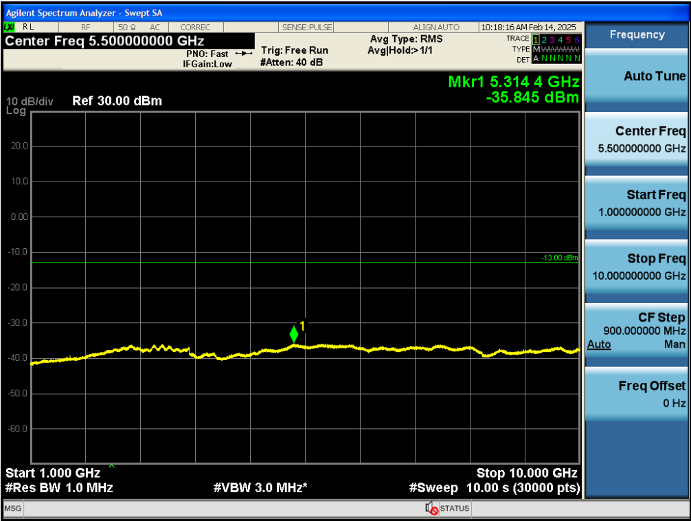
Test_Graph_bandGSM850_824.2MHz_GPRS 1Slot_1G_10G_TX
