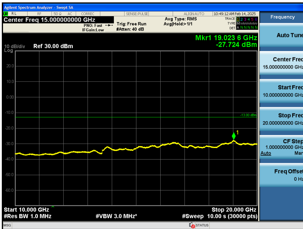
Test_Graph_bandGSM1900_1880MHz_GPRS 1Slot_10G_20G_TX
