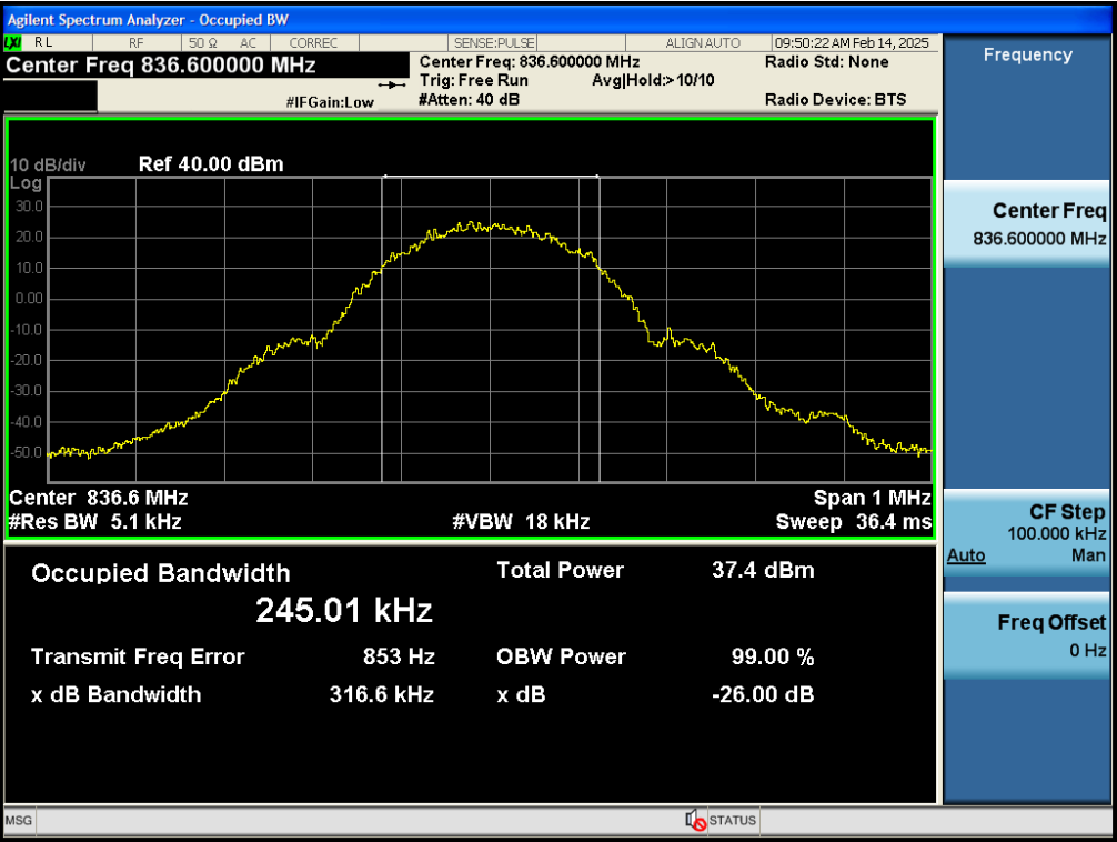
Test_Graph_bandGSM850_836.6MHz_GPRS 1Slot_OBW&EBW
