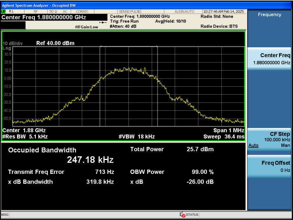
Test_Graph_bandGSM1900_1880MHz_Voice_OBW&EBW
