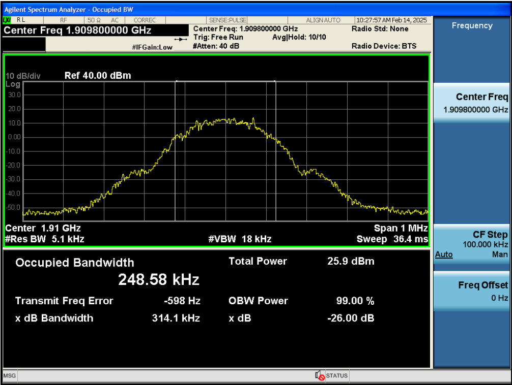
Test_Graph_bandGSM1900_1909.8MHz_Voice_OBW&EBW
