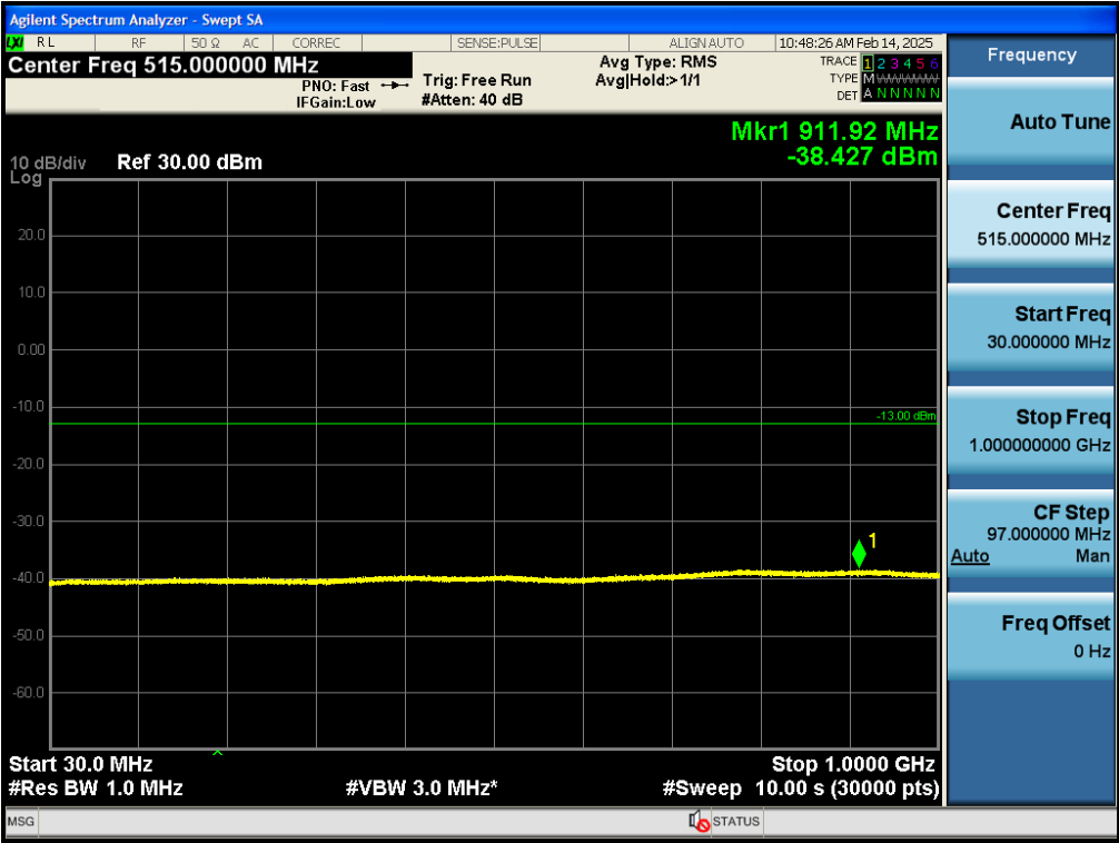
Test_Graph_bandGSM1900_1880MHz_GPRS 1Slot_30M_1G_TX
