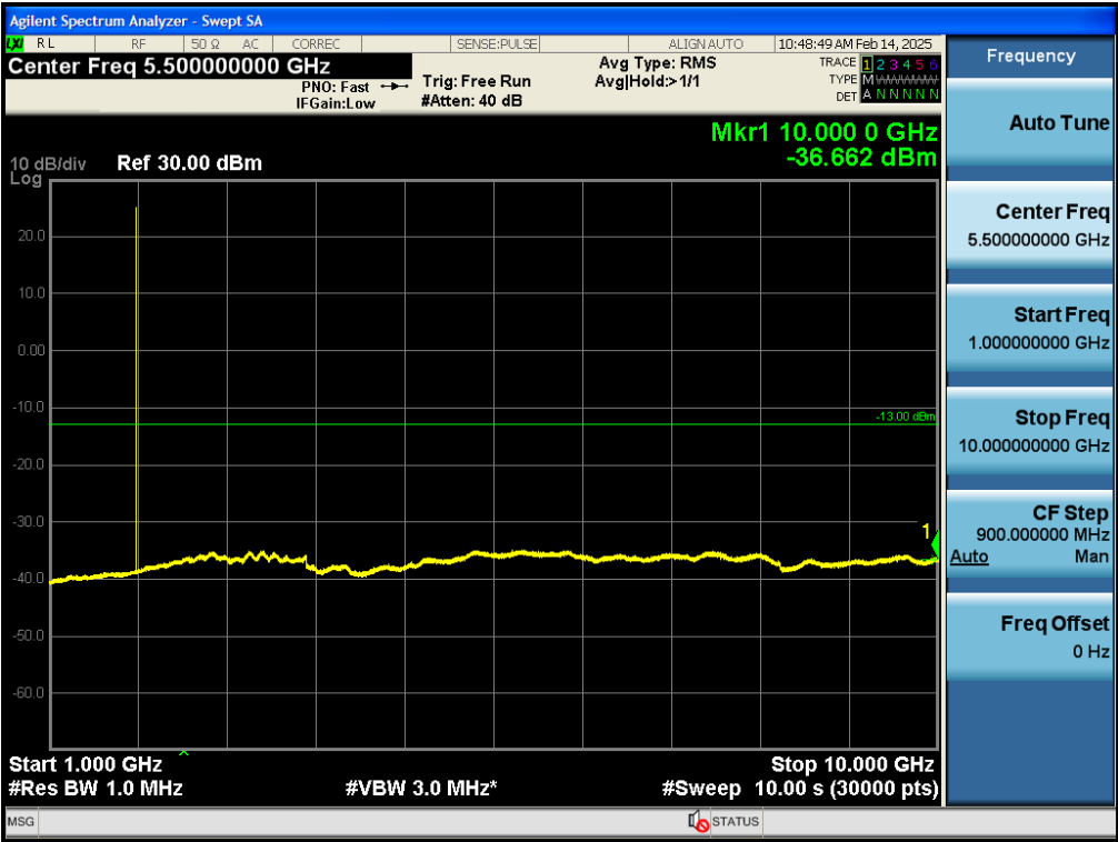
Test_Graph_bandGSM1900_1880MHz_GPRS 1Slot_1G_10G_TX
