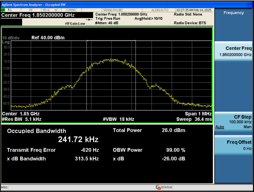
Test_Graph_bandGSM1900_1850.2MHz_Voice_OBW&EBW
