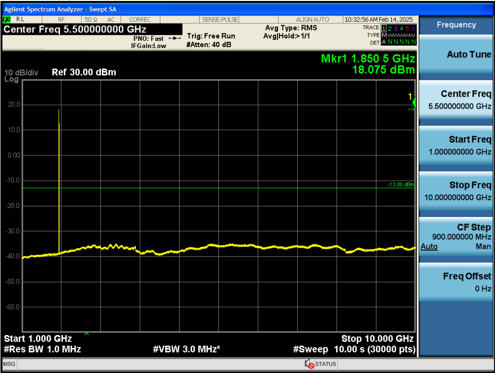
Test_Graph_bandGSM1900_1850.2MHz_Voice_1G_10G_TX
