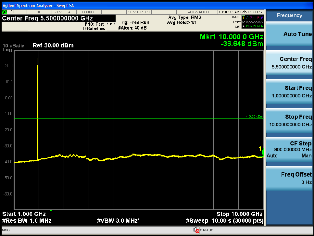
Test_Graph_bandGSM1900_1850.2MHz_GPRS 1Slot_1G_10G_TX
