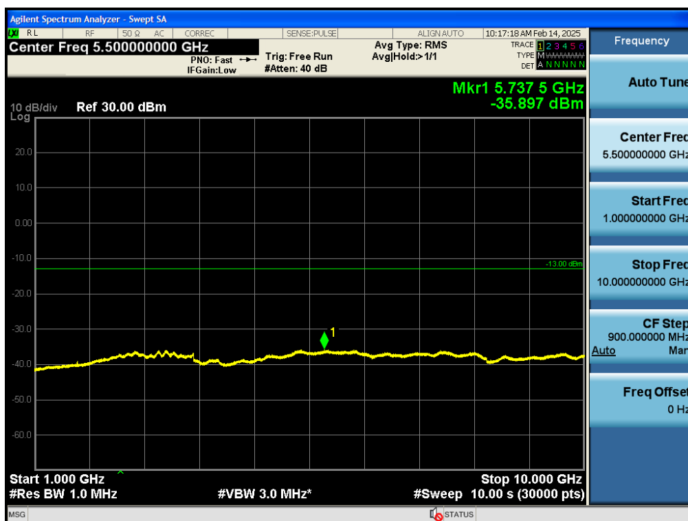
Test_Graph_bandGSM850_848.8MHz_Voice_1G_10G_TX
