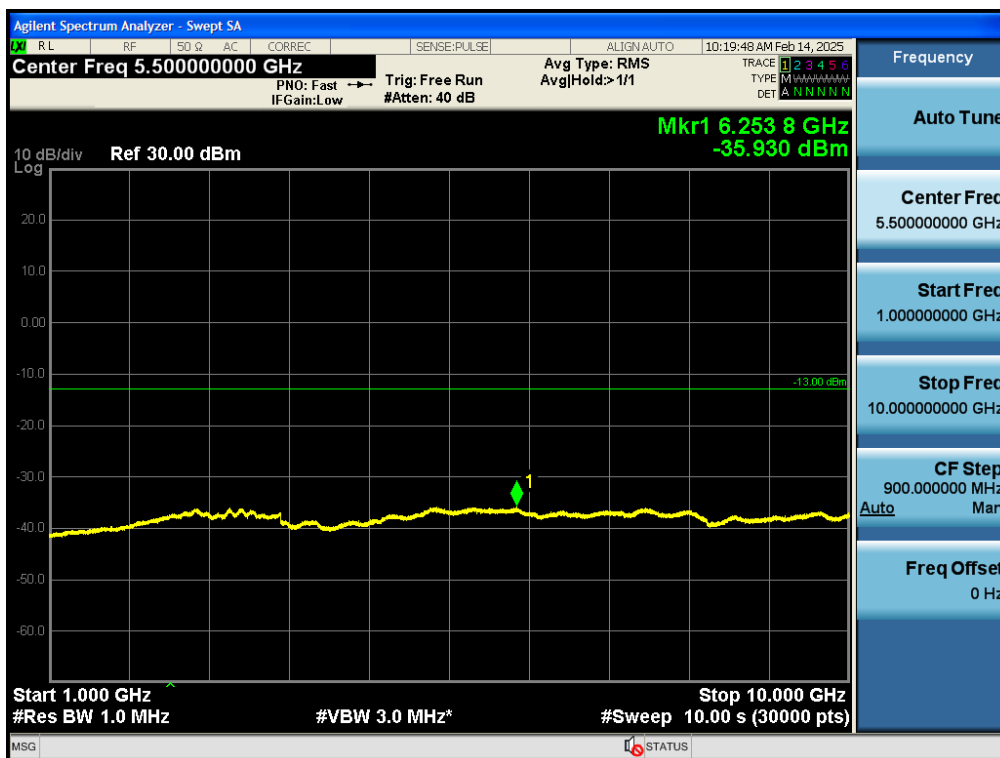
Test_Graph_bandGSM850_848.8MHz_GPRS 1Slot_1G_10G_TX
