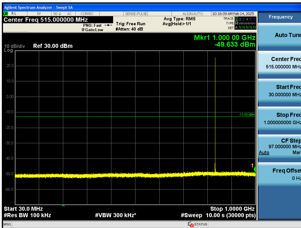
Test_Graph_bandGSM850_836.6MHz_Voice_30M_1G_TX
