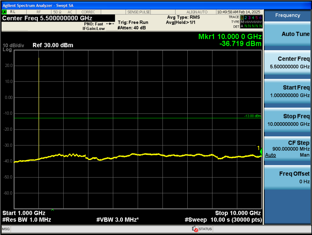
Test_Graph_bandGSM1900_1909.8MHz_GPRS 1Slot_1G_10G_TX
