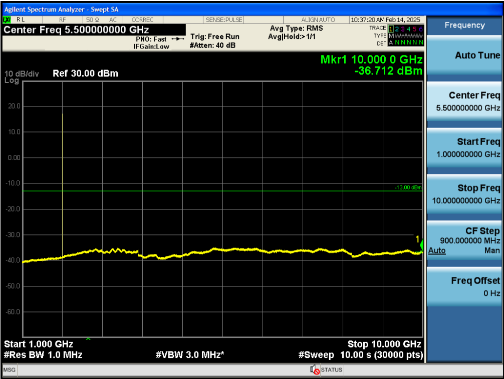
Test_Graph_bandGSM1900_1909.8MHz_Voice_1G_10G_TX
