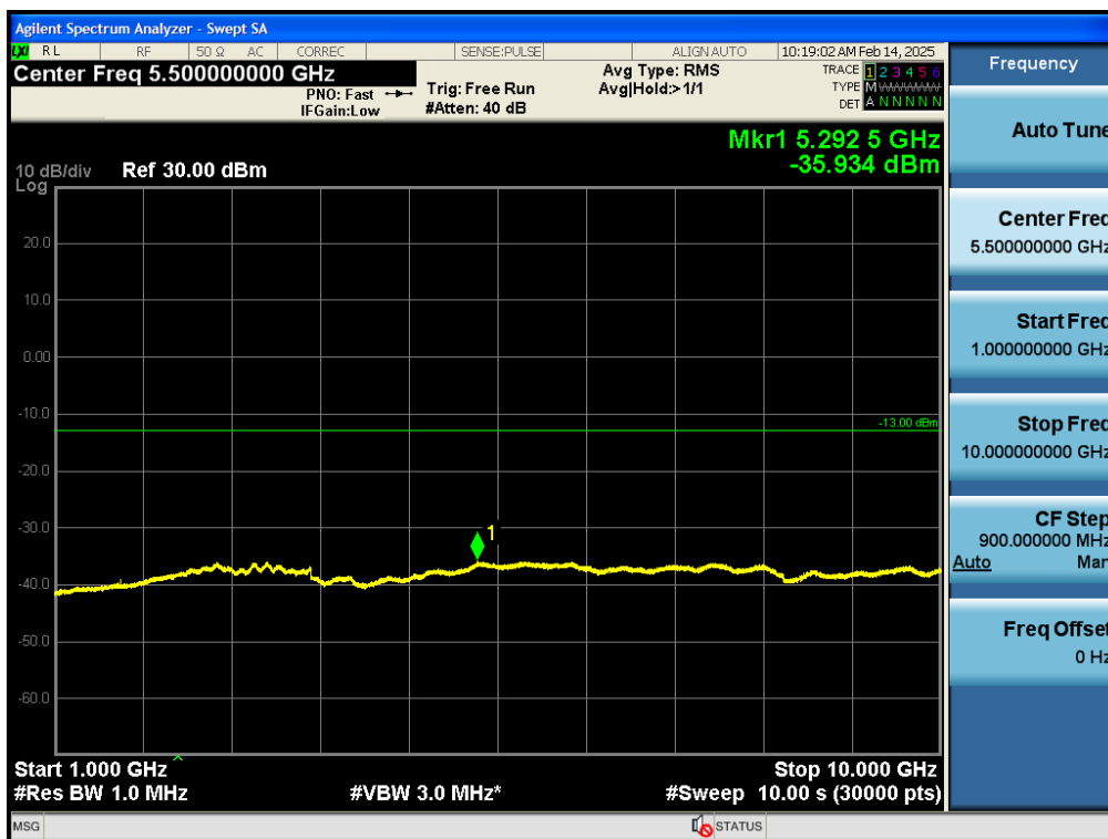
Test_Graph_bandGSM850_836.6MHz_GPRS 1Slot_1G_10G_TX
