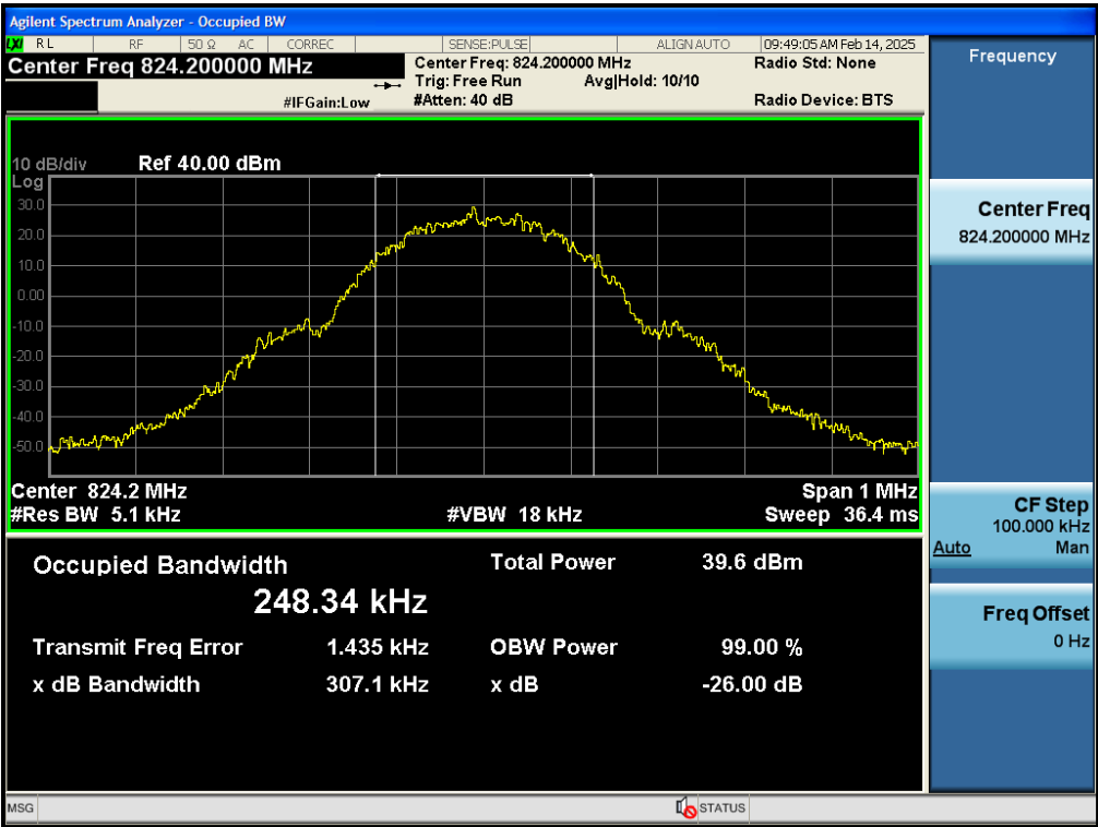
Test_Graph_bandGSM850_824.2MHz_Voice_OBW&EBW
