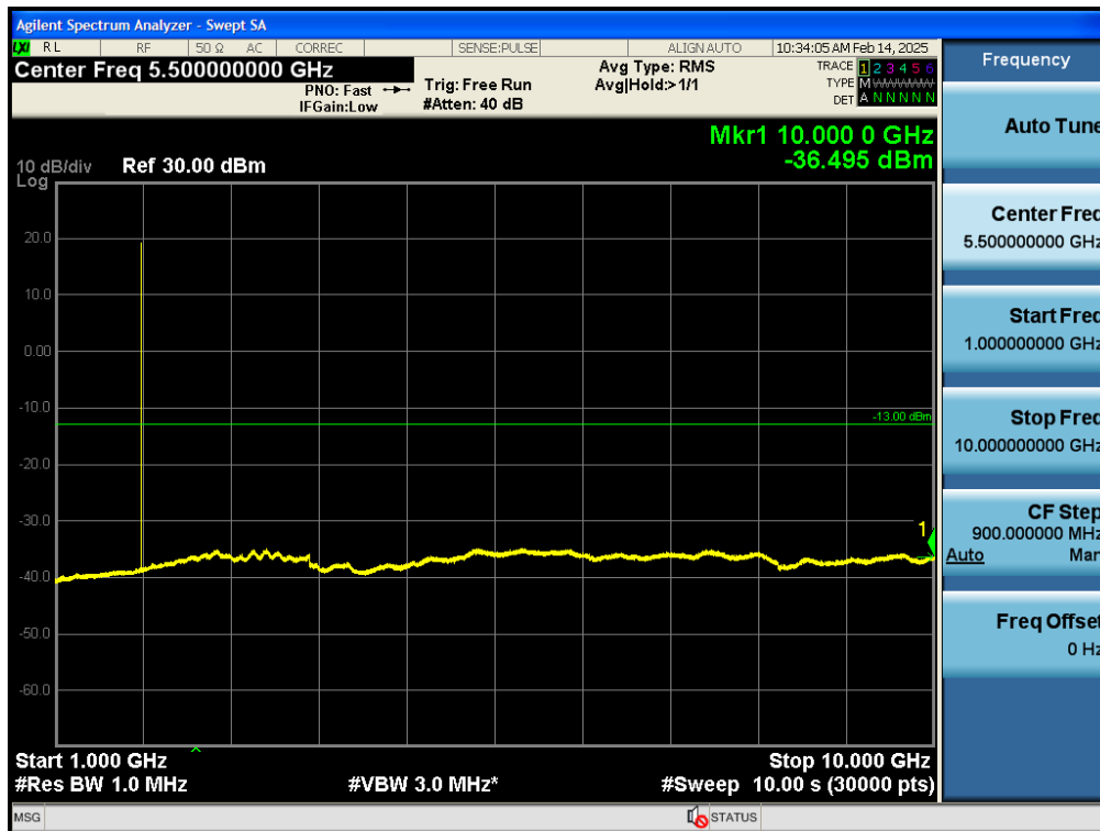
Test_Graph_bandGSM1900_1880MHz_Voice_1G_10G_TX
