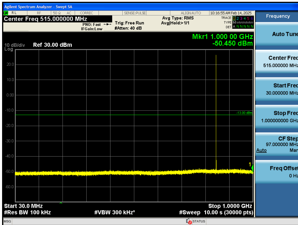
Test_Graph_bandGSM850_848.8MHz_Voice_30M_1G_TX
