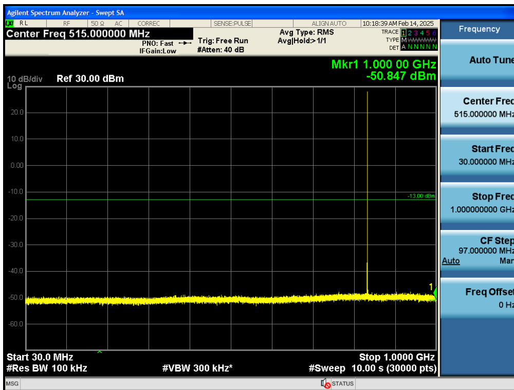
Test_Graph_bandGSM850_836.6MHz_GPRS 1Slot_30M_1G_TX
