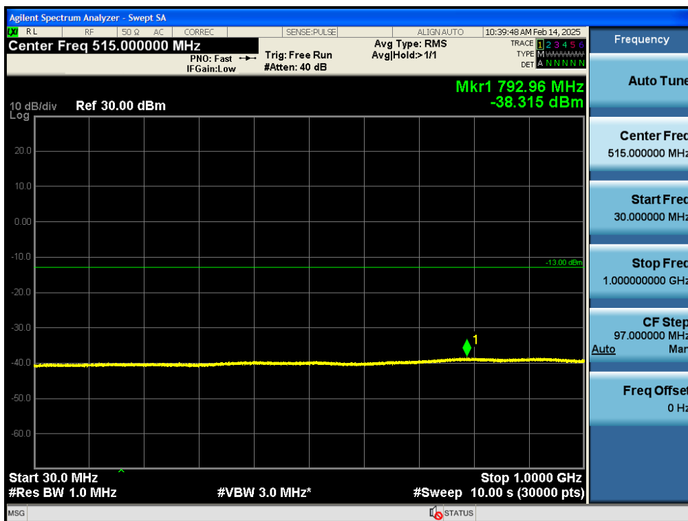
Test_Graph_bandGSM1900_1850.2MHz_GPRS 1Slot_30M_1G_TX
