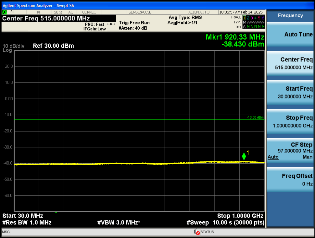
Test_Graph_bandGSM1900_1909.8MHz_Voice_30M_1G_TX
