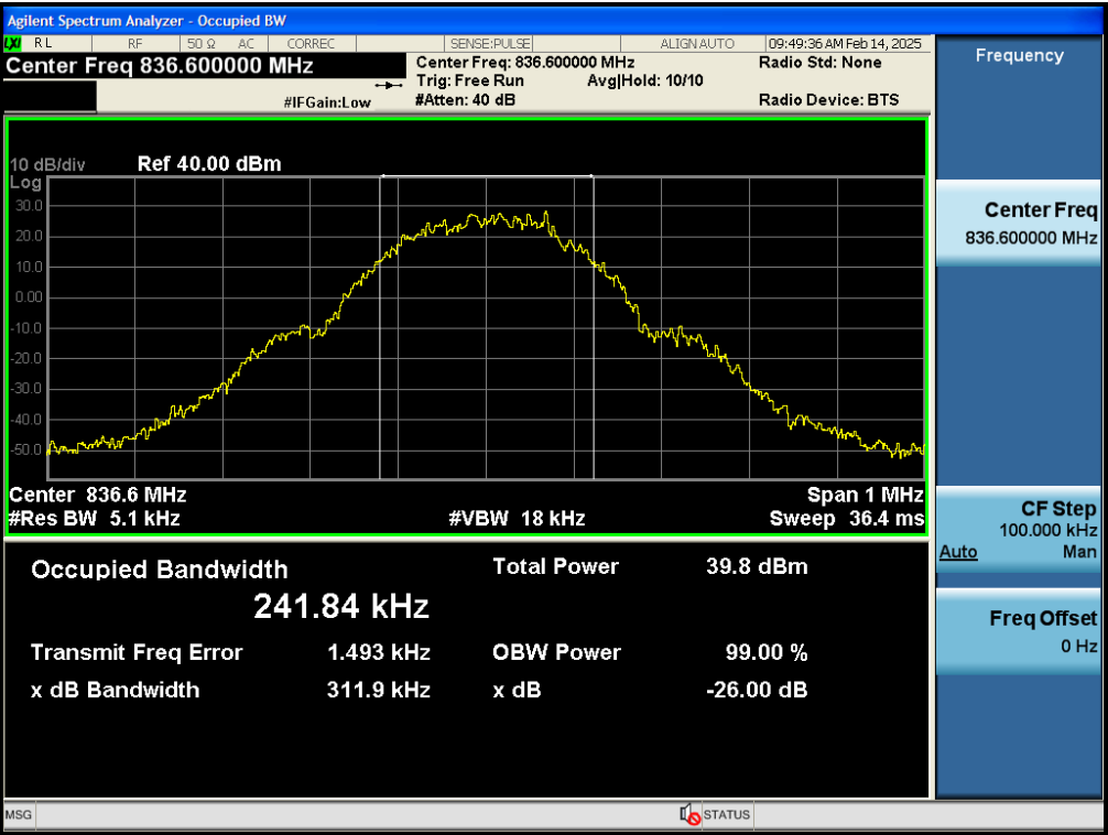
Test_Graph_bandGSM850_836.6MHz_Voice_OBW&EBW
