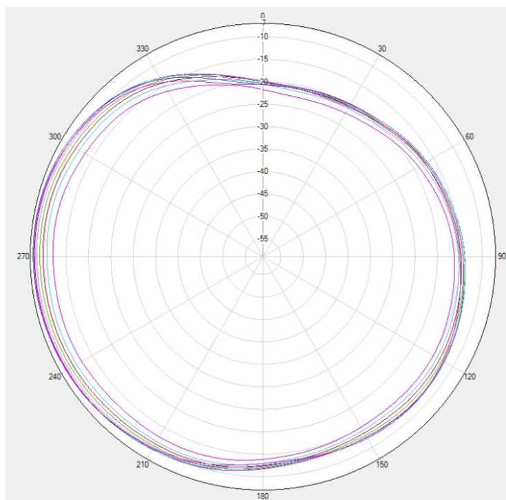
GSM900 / WCDMA B8 / LTE B8 \Theta=90^\circ
