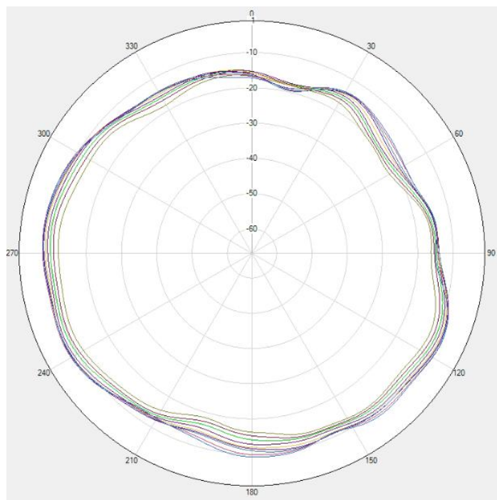
GSM900 / WCDMA B8 / LTE B8 \Phi=90^\circ
