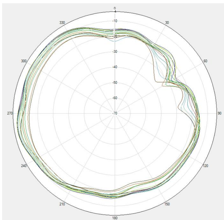
5G WIFI \Theta=90^\circ
