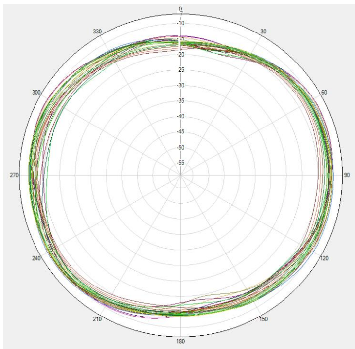
DCS1800/PCS1900/WCDMA B1/B2/B4/ LTE B1/B2/B3/B4/B66 Theta=90deg
