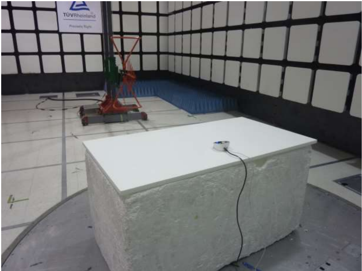
Figure 3: Test Setup for 30 MHz to 1 GHz (View 1)
