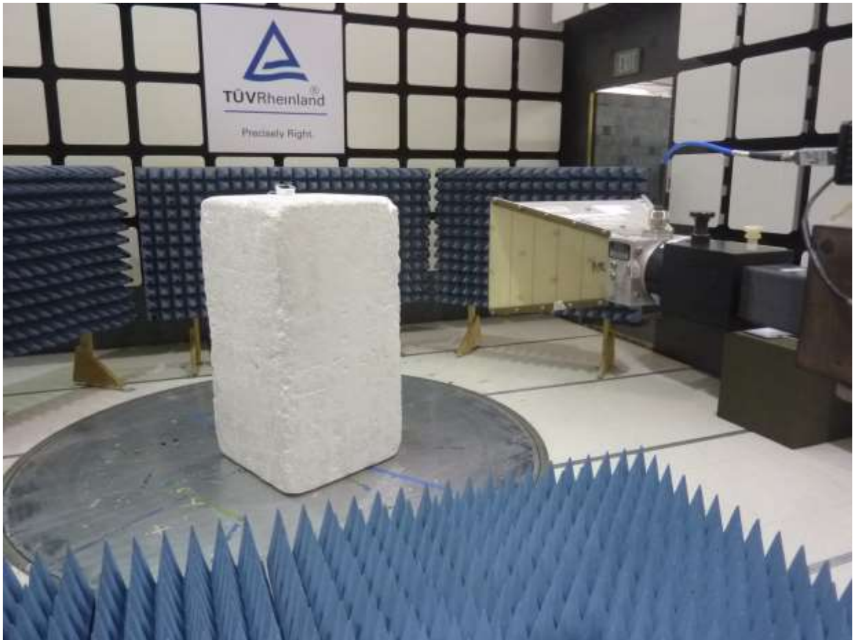
Figure 6: Test Setup for 1 GHz to 18 GHz (View 2)
