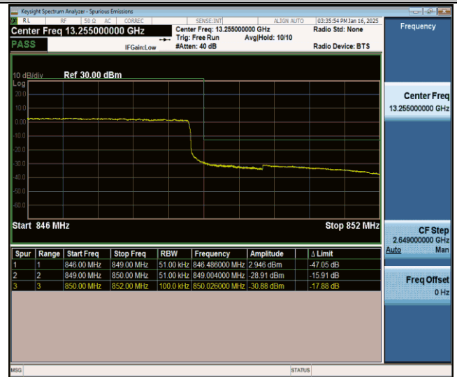
Band26(824-849)-5MHz-QPSK-27015-25RB#0-PASS
