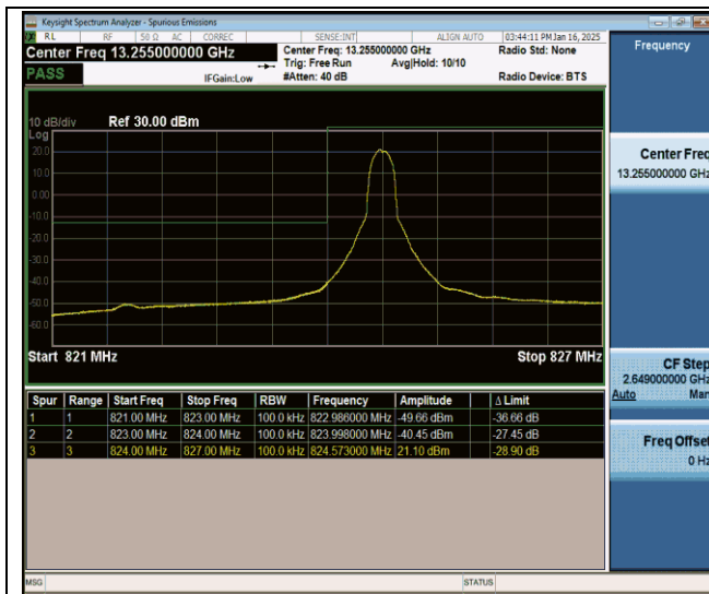
Band26(824-849)-10MHz-QPSK-26840-1RB#0-PASS
