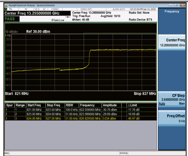
Band26(824-849)-5MHz-QPSK-26815-25RB#0-PASS
