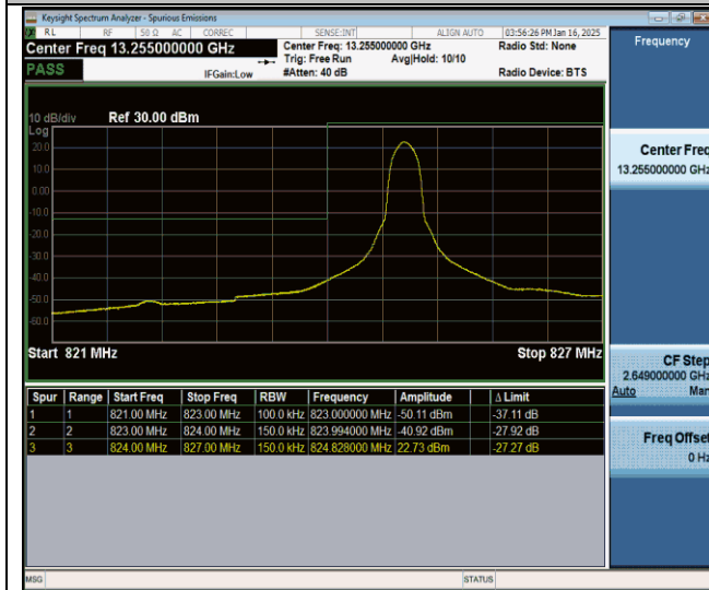
Band26(824-849)-15MHz-QPSK-26865-1RB#0-PASS
