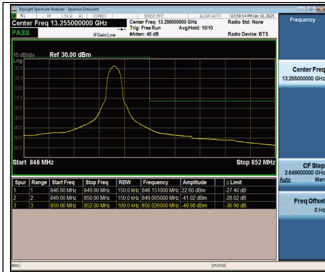
Band26(824-849)-15MHz-QPSK-26965-1RB#74-PASS
