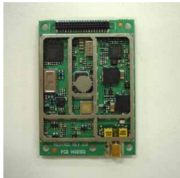
SB555 Module Interior Bottom View
