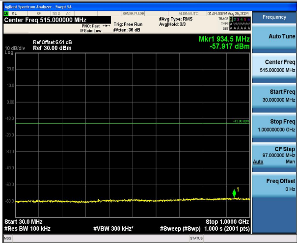
Band4_3MHz_QPSK_20175_1RB#0_30~1000_30~1000
