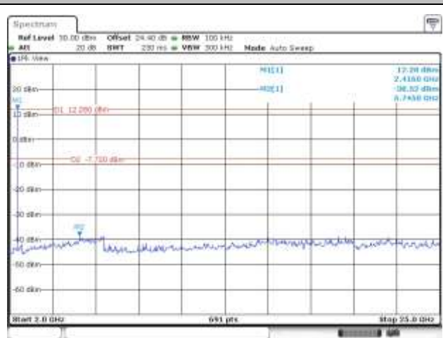
CSE Plot on CH 00 between 2 GHz ~ 25 GHz
