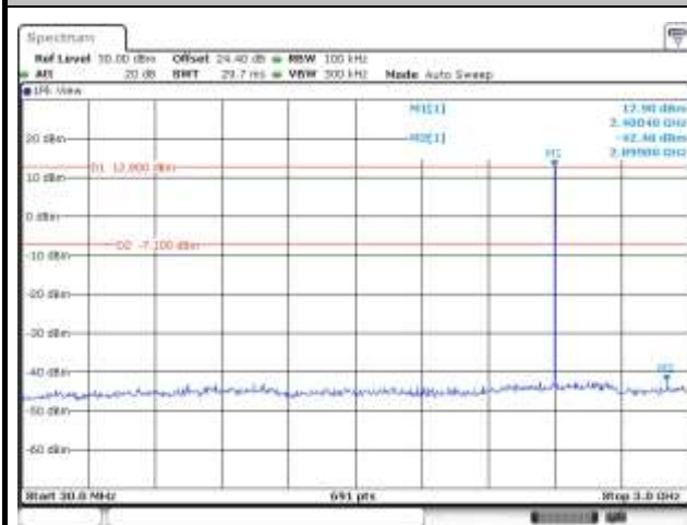
CSE Plot on CH 00 between 30 MHz ~ 3 GHz
