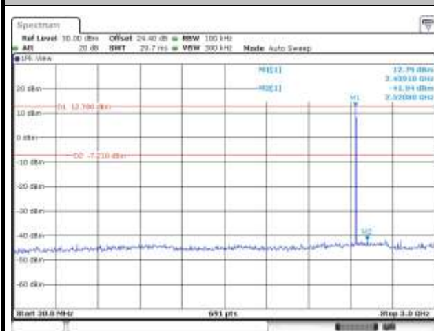
CSE Plot on CH 39 between 30 MHz ~ 3 GHz
