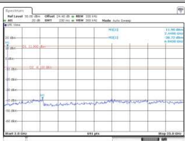
CSE Plot on CH 39 between 2 GHz ~ 25 GHz
