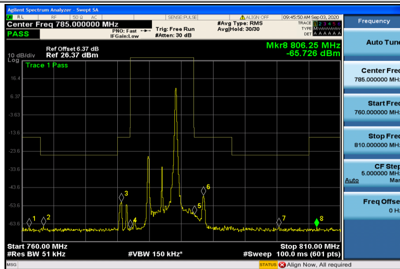
Band13-5MHz-16QAM-23230-1RB#24
