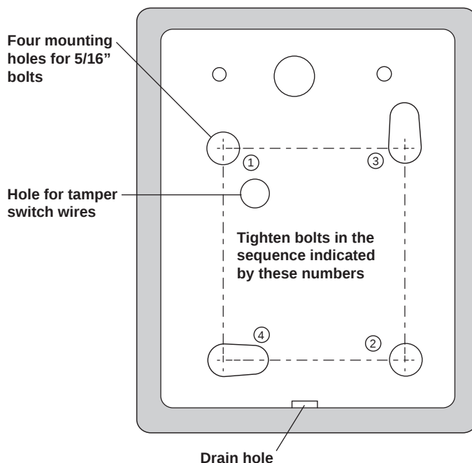
Figure 1. Mounting holes
