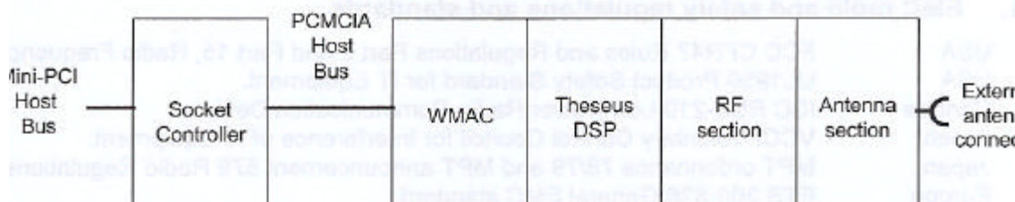
Figure 1. Functional diagram of the mini-PCI card.
