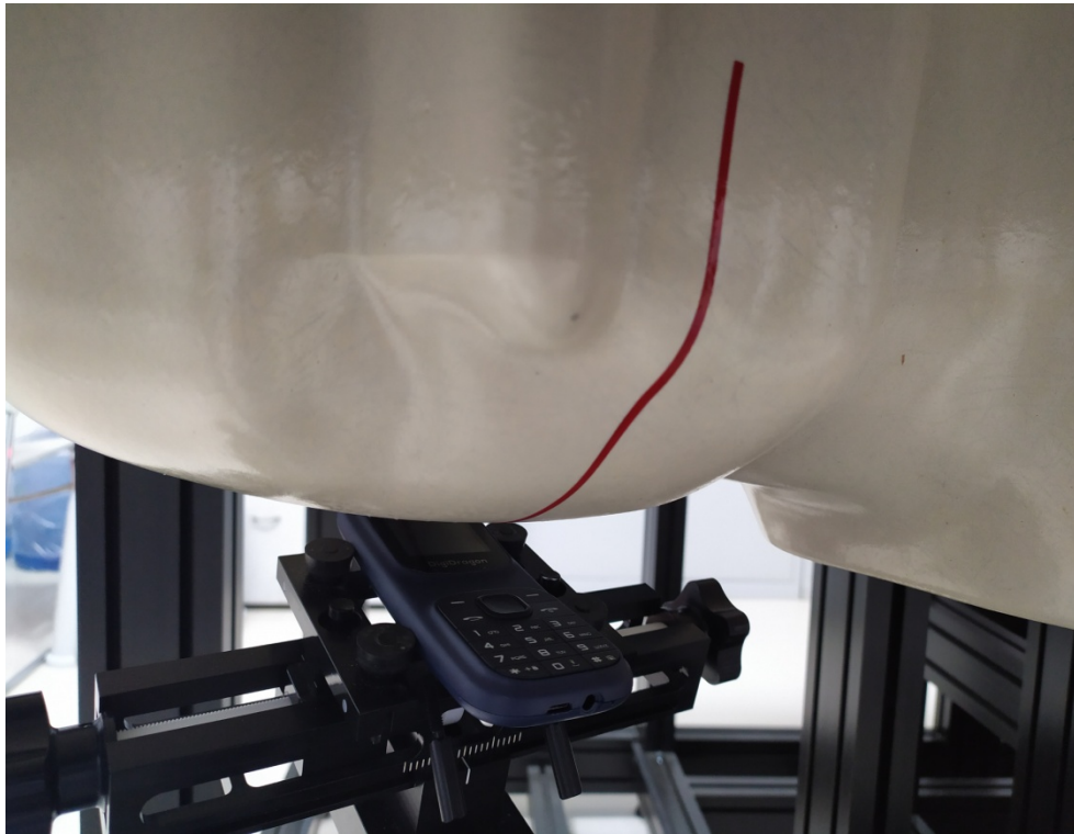
Head Right Tilt Setup Photo
