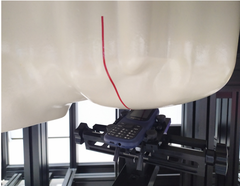
Head Left Tilt Setup Photo
