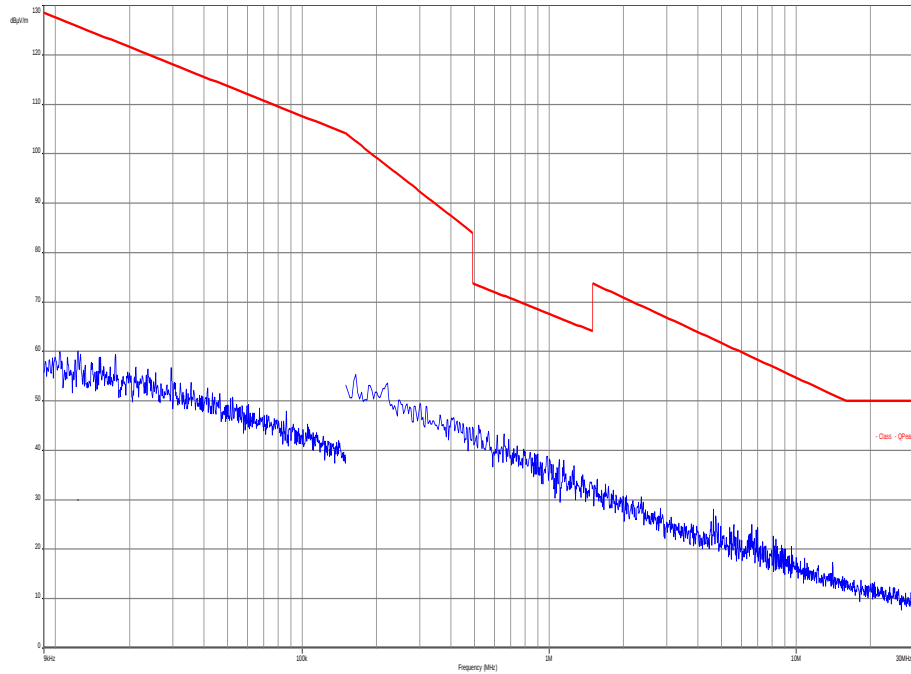
Plot 1: Channel 18900 (Traffic mode up to 30 MHz)
