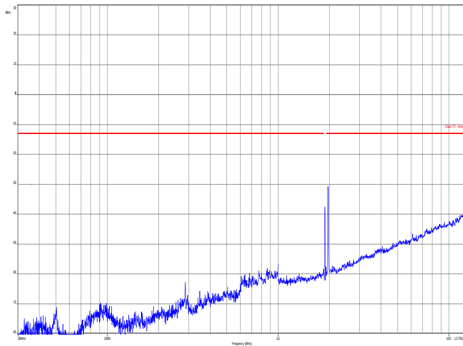
Plot 6: Channel 18900 (30 MHz – 12.75 GHz)
