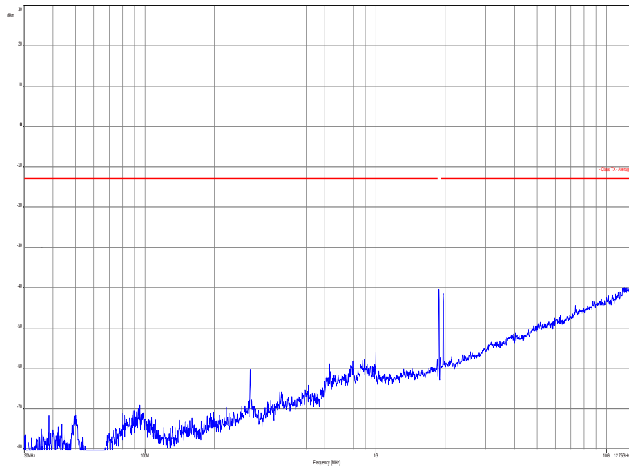
Plot 2: Channel 18900 (30 MHz – 12.75 GHz)
