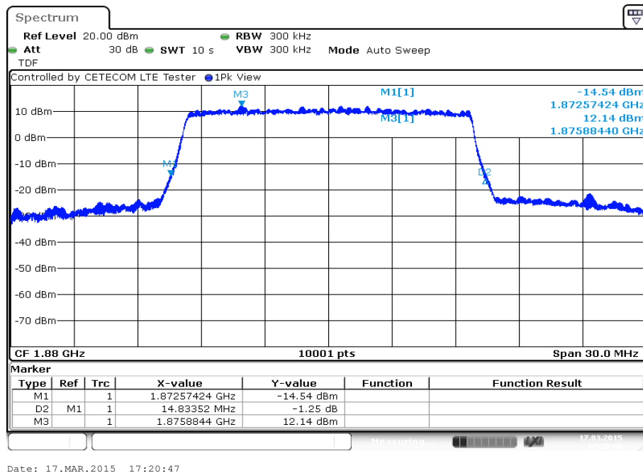
Plot 10: 15 MHz (-26 dBc BW)
