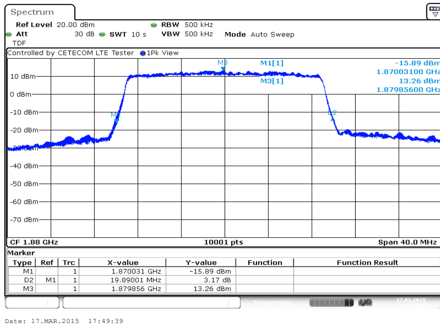
Plot 12: 20 MHz (-26 dBc BW)
