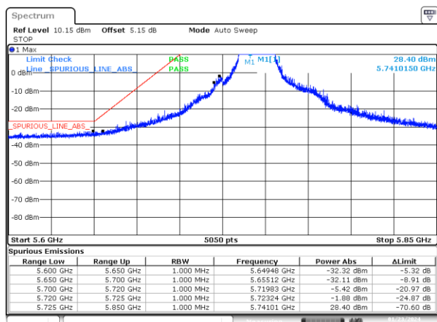
BE-NR-LOW, MIMO-A, 802.11ax20-MCS0, Ch149
