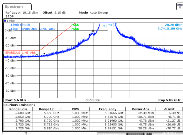
BE-NR-LOW, SISO-B, 802.11ax20-MCS0, Ch149
