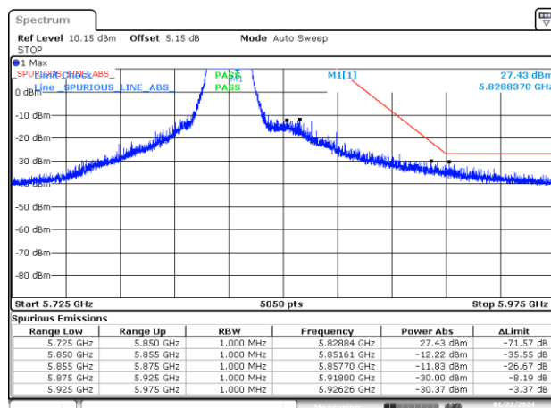
BE-NR-HIGH, MIMO-B, 802.11ax20-MCS0, Ch165
