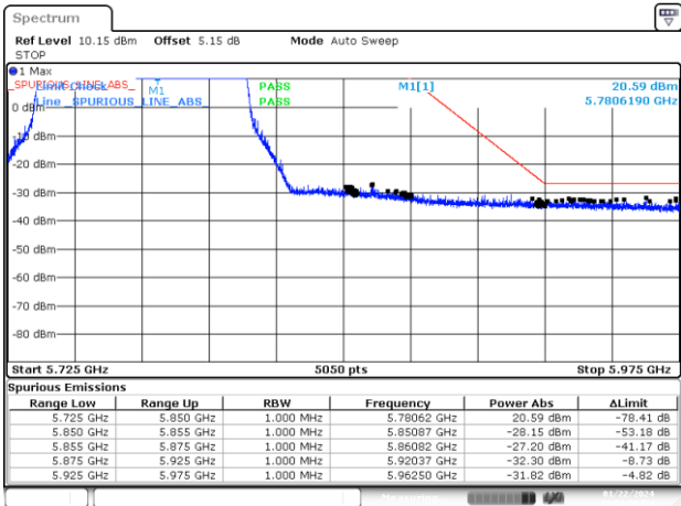
BE-NR-HIGH, MIMO-B, 802.11ax80-MCS0, Ch155
