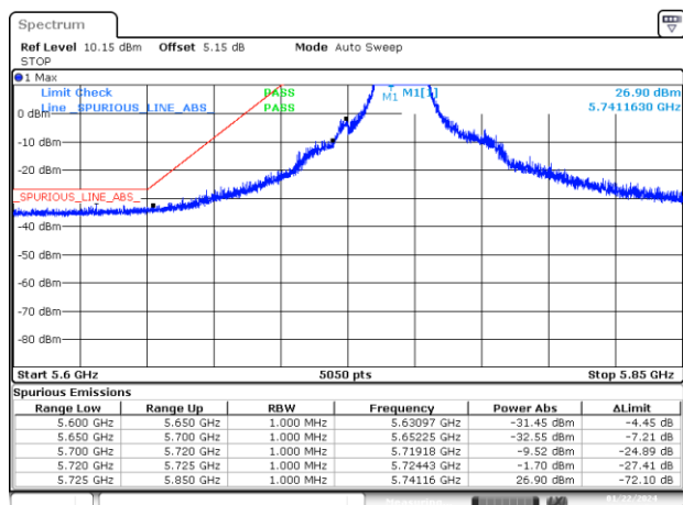
BE-NR-LOW, SISO-B, 802.11n20-HT0, Ch149
