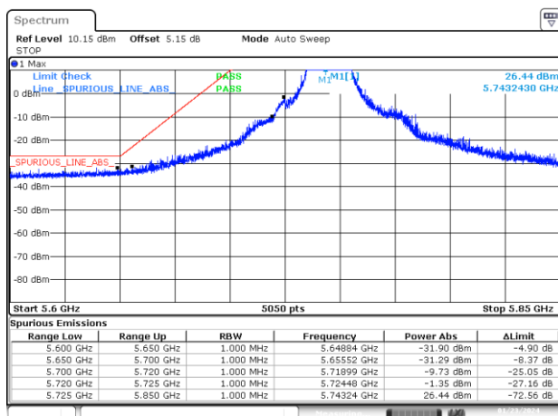
BE-NR-LOW, MIMO-A, 802.11n20-HT0, Ch149
