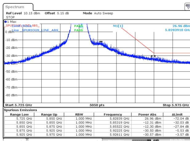
BE-NR-HIGH, MIMO-A, 802.11ax20-MCS0, Ch165
