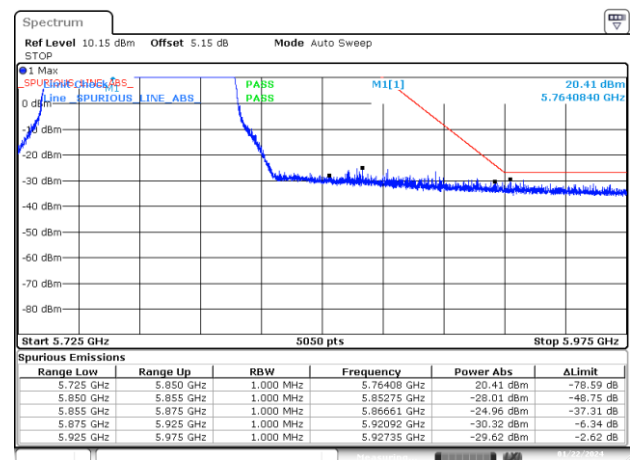
BE-NR-HIGH, SISO-B, 802.11ax80-MCS0, Ch155
