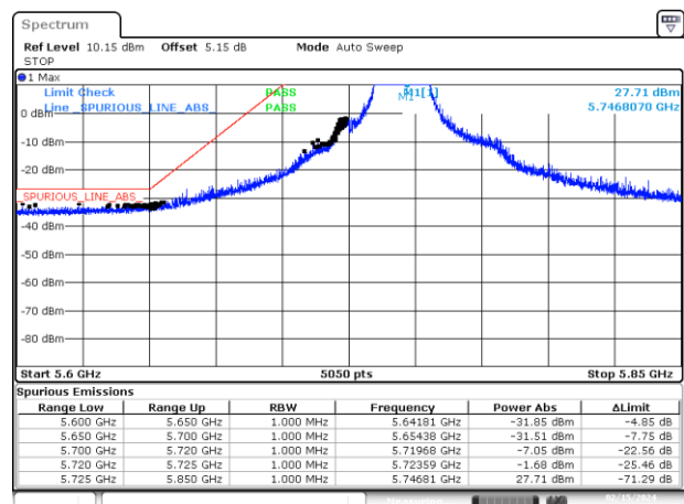
BE-NR-LOW, MIMO-B, 802.11ax20-MCS0, Ch149
