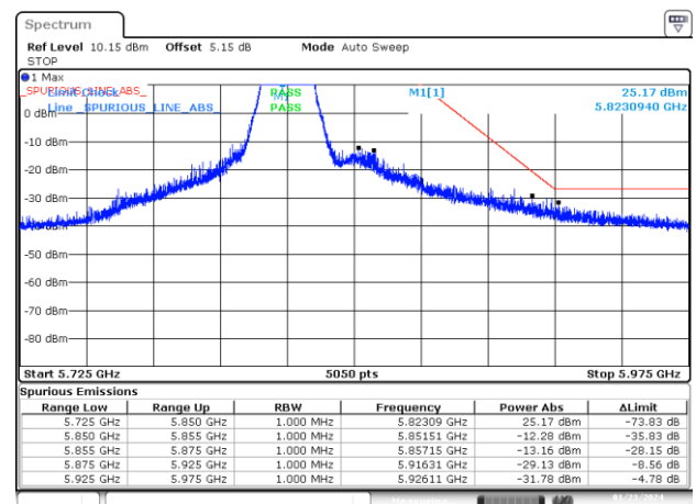
BE-NR-HIGH, MIMO-A, 802.11n20-HT0, Ch165
