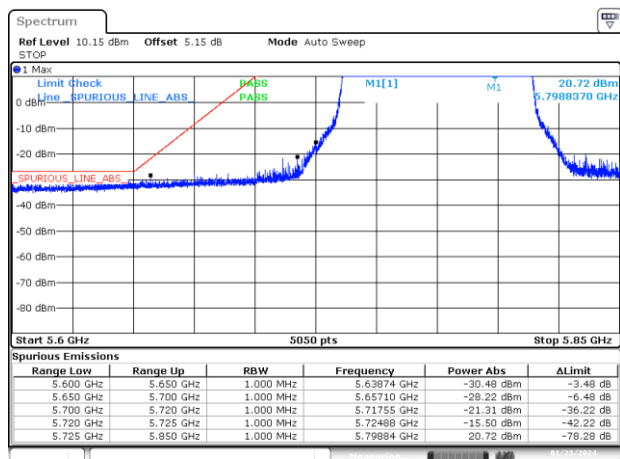
BE-NR-LOW, SISO-A, 802.11ax80-MCS0, Ch155
