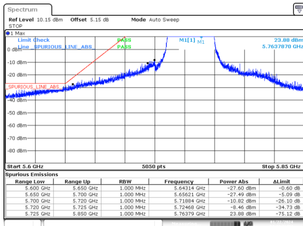
BE-NR-LOW, SISO-B, 802.11ax40-MCS0, Ch151
