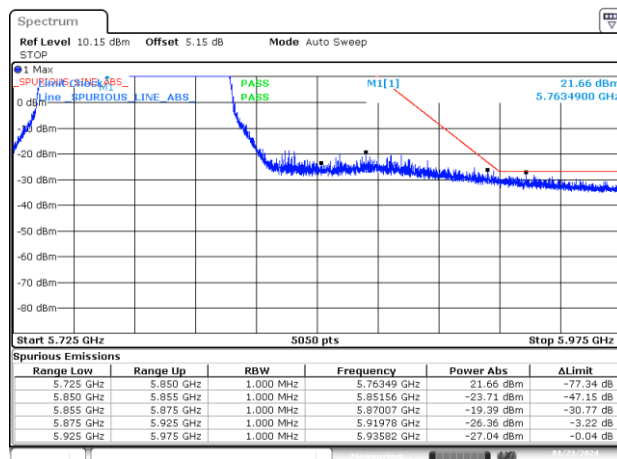
BE-NR-HIGH, SISO-A, 802.11ax80-MCS0, Ch155
