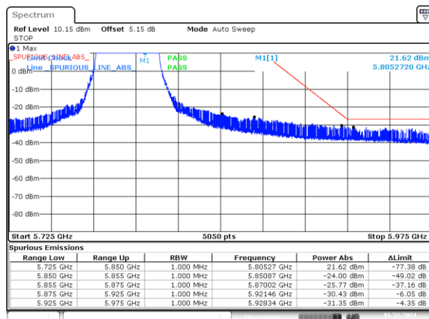
BE-NR-HIGH, MIMO-B, 802.11n40-HT0, Ch159
