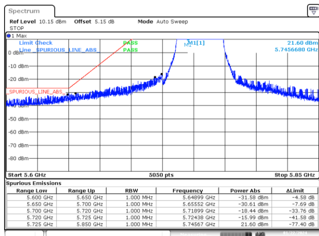
BE-NR-LOW, MIMO-B, 802.11n40-HT0, Ch151
