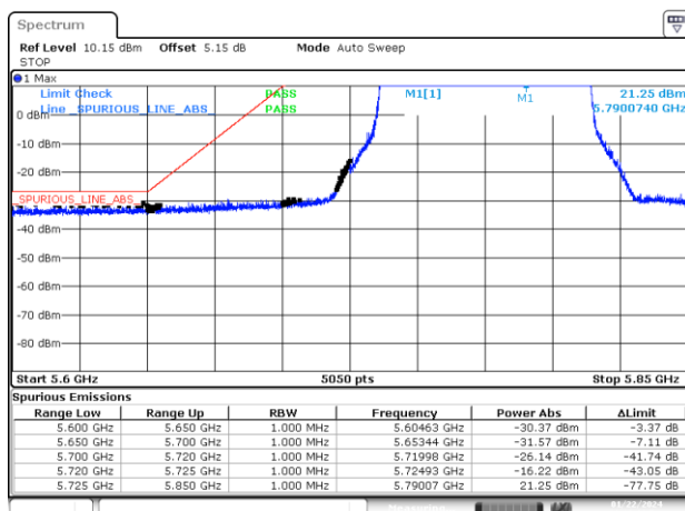
BE-NR-LOW, SISO-B, 802.11ax80-MCS0, Ch155
