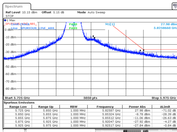
BE-NR-HIGH, SISO-B, 802.11ax20-MCS0, Ch165
