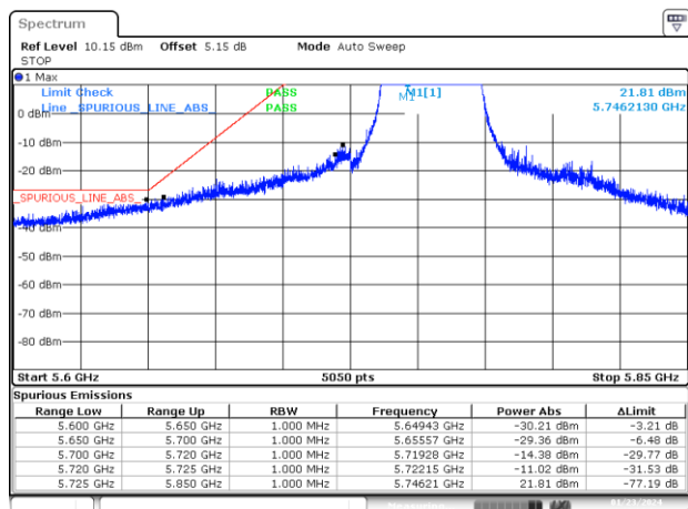
BE-NR-LOW, MIMO-A, 802.11n40-HT0, Ch151
