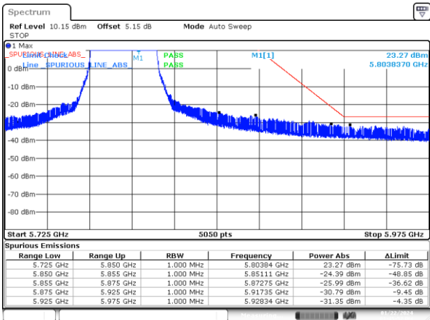
BE-NR-HIGH, MIMO-B, 802.11ax40-MCS0, Ch159
