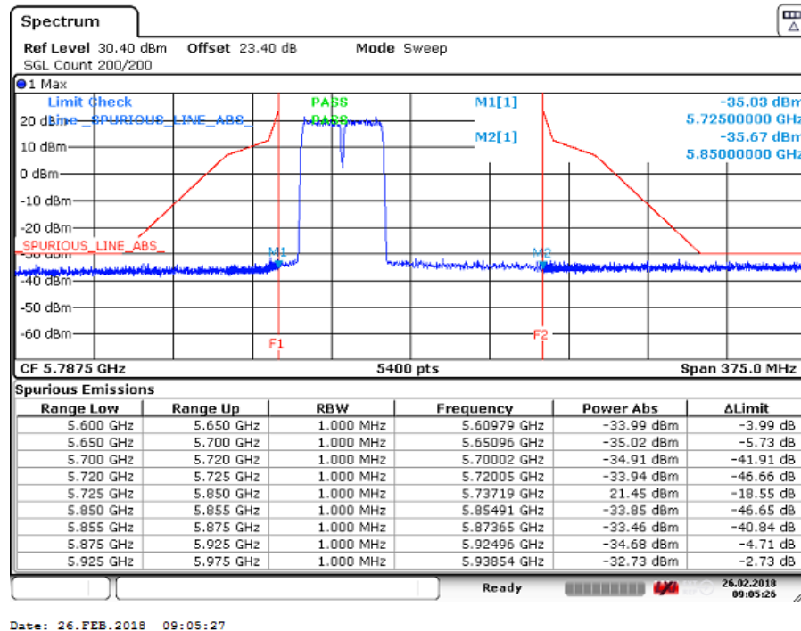
Figure 328 Spurious Emissions (Lower Band Edge) – QPSK (5745.0/ 5765.0 MHz) (2 X 20MHz Channel BW)
