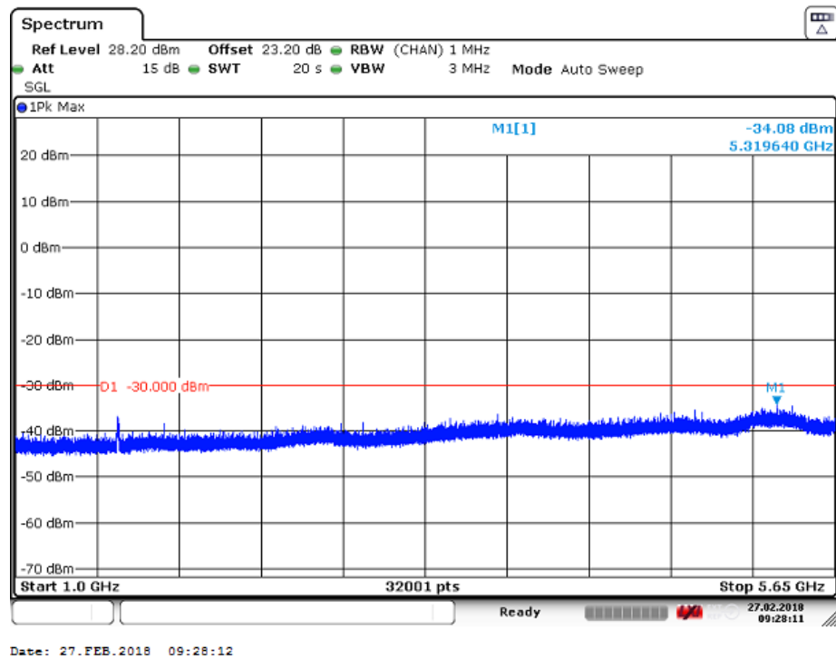
Figure 316 Spurious Emissions (1 GHz – 5.65 GHz) – QPSK (5785.0 MHz) (20MHz Channel BW)
