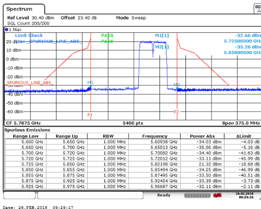
Figure 335 Spurious Emissions (Upper Band Edge) – 256QAM (5805.0/ 5825.0 MHz) (2 X 20MHz Channel BW)
