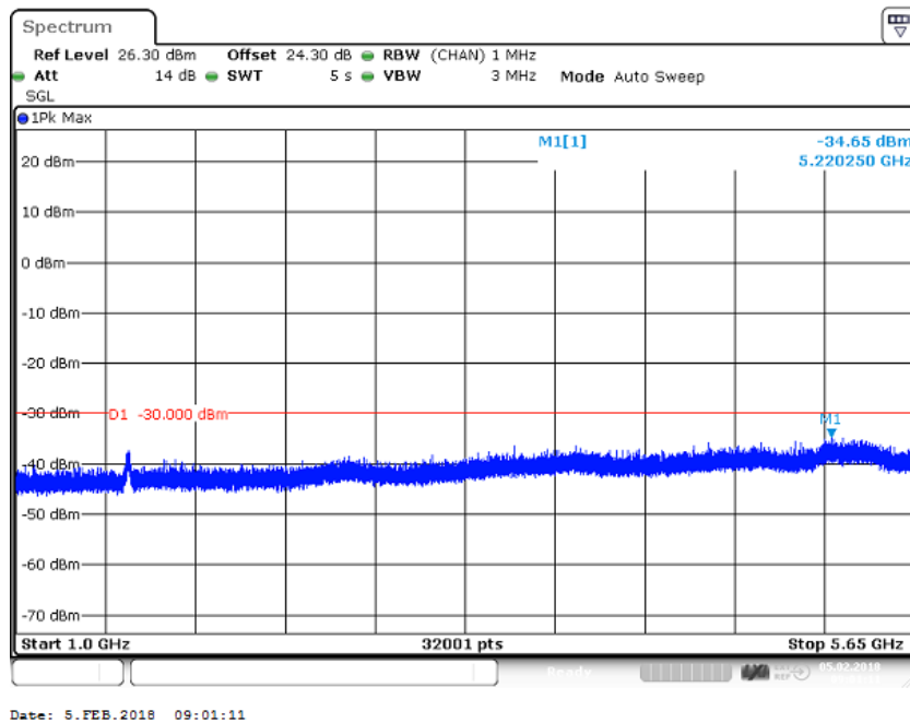
Figure 364 Spurious Emissions (1 GHz – 5.65 GHz) – QPSK (5765.0/ 5787.0/ 5805.0 MHz) (3 X 20MHz Channel BW)
