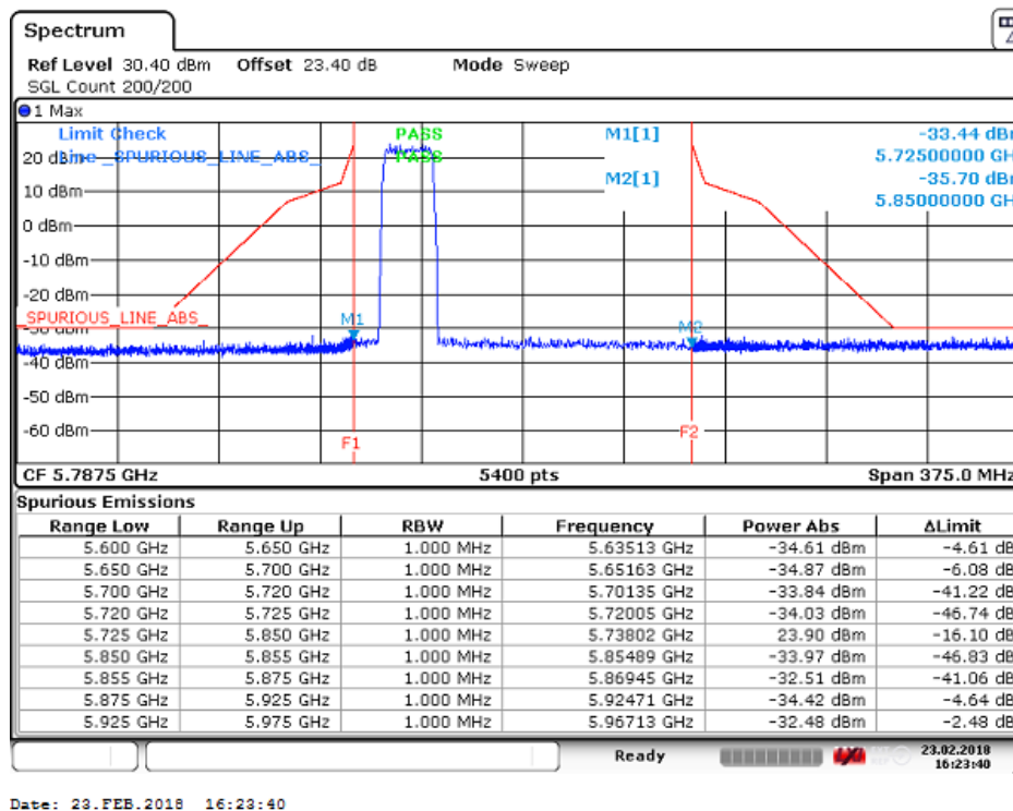
Figure 307 Spurious Emissions (Lower Band Edge) – 256QAM (5745.0 MHz) (20MHz Channel BW)
