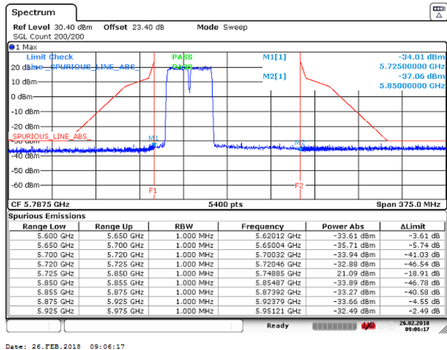
Figure 329 Spurious Emissions (Lower Band Edge) – 64QAM (5745.0/ 5765.0 MHz) (2 X 20MHz Channel BW)
