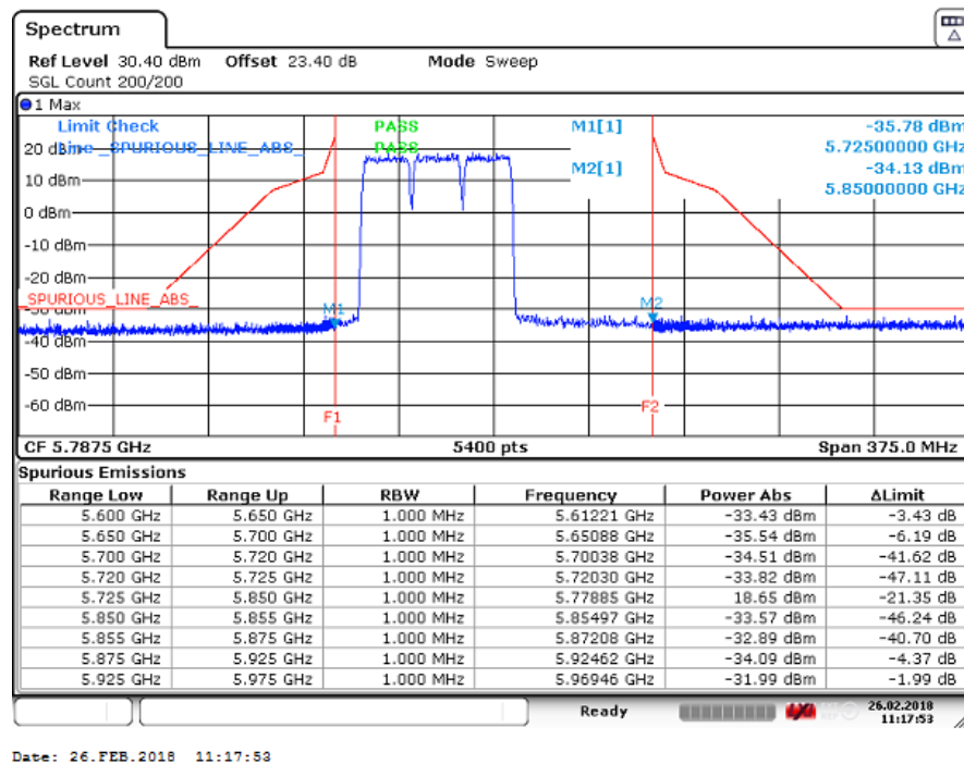
Figure 353 Spurious Emissions (Lower Band Edge) – 64QAM (5745.0/ 5765.0/ 5785.0 MHz) (3 X 20MHz Channel BW)
