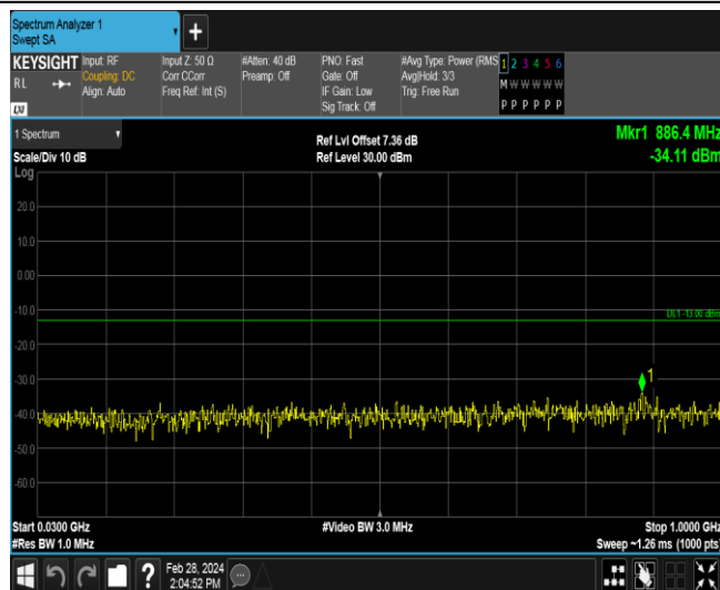
Band2-10MHz-16QAM-18650-1RB#0-Range1:30~1000MHz
