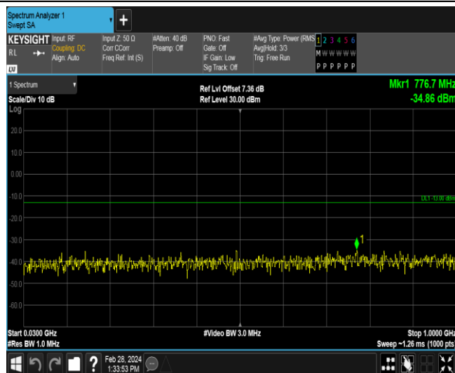
Band2-3MHz-QPSK-18615-1RB#0-Range1:30~1000MHz
