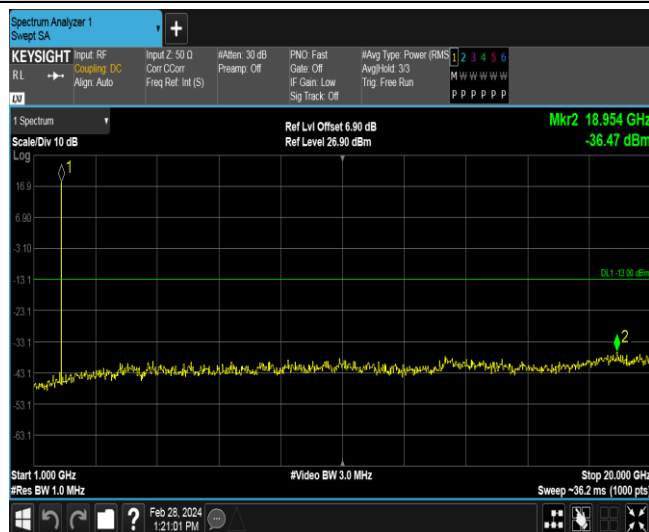
Band2-1.4MHz-16QAM-18607-1RB#0-Range2:1000~20000MHz
