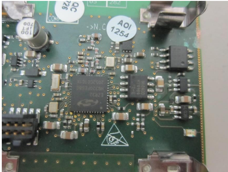
Photograph No.4 Component side of the RF PCB
