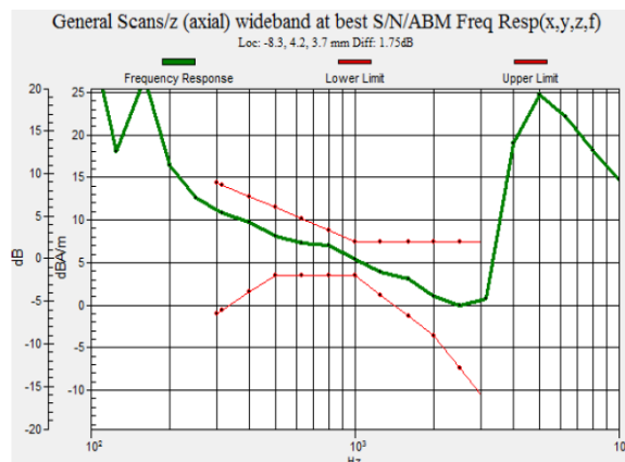
Fig 7.2 GSM1900 Ch661
