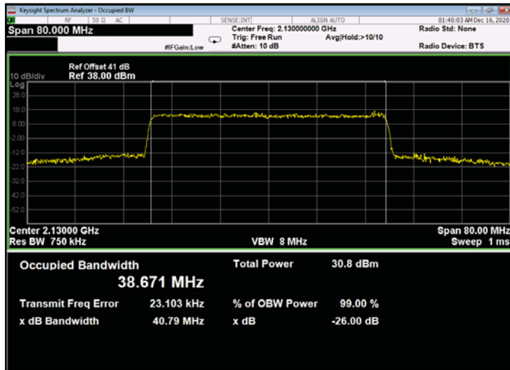
Figure 711: 256QAM 40MHz B.W.; 2130.0MHz, 15kHz - Output
