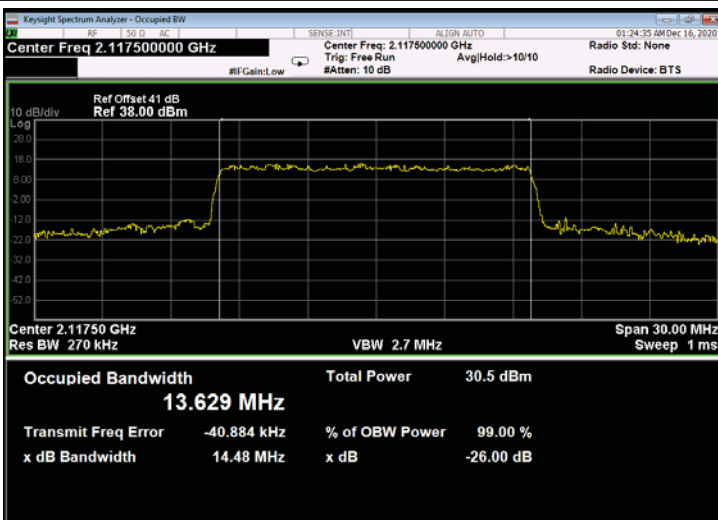
Figure 685: 256QAM 15MHz B.W.; 2117.5MHz, 30kHz - Output
