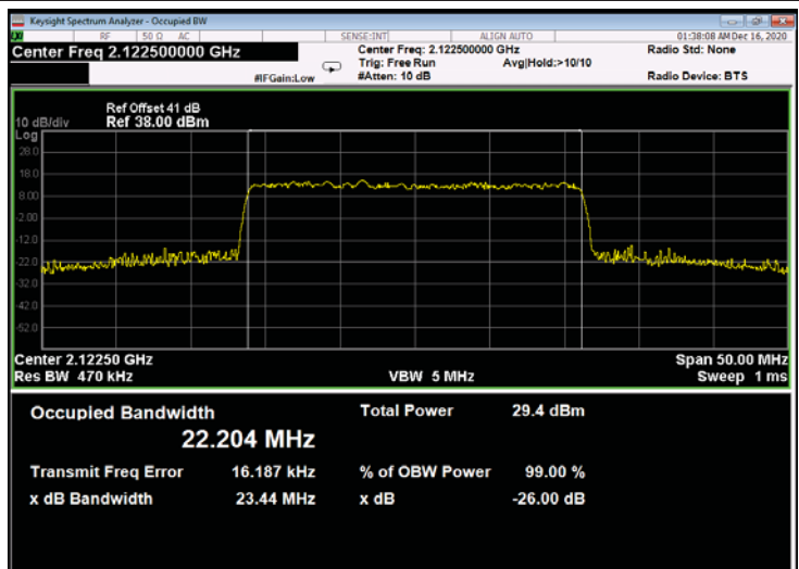
Figure 704: 256QAM 25MHz B.W.; 2122.5MHz, 60kHz - Output
