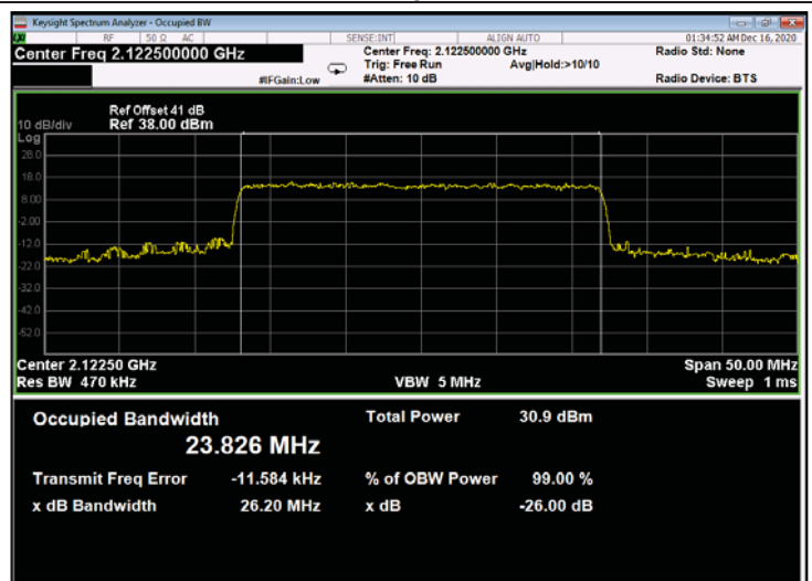
Figure 702: 256QAM 25MHz B.W.; 2122.5MHz, 15kHz - Output
