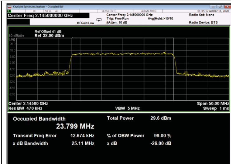
Figure 705: 256QAM 25MHz B.W.; 2145.0MHz, 15kHz - Output
