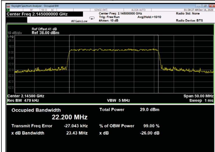
Figure 707: 256QAM 25MHz B.W.; 2145.0MHz, 60kHz - Output
