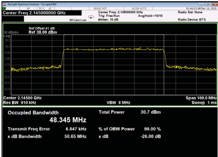
Figure 723: 256QAM 50MHz B.W.; 2145.0MHz, 15kHz - Output
