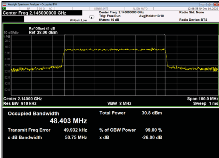
Figure 657: 64QAM 50MHz B.W.; 2145MHz, 15kHz - Output
