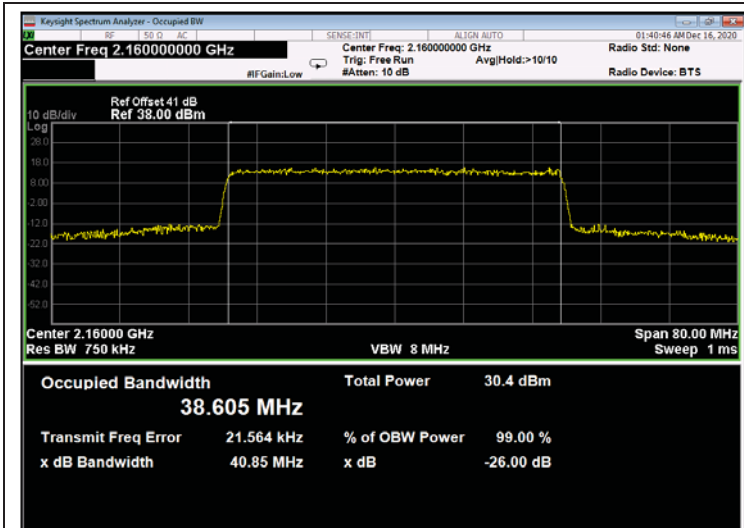
Figure 717: 256QAM 40MHz B.W.; 2160.0MHz, 15kHz - Output
