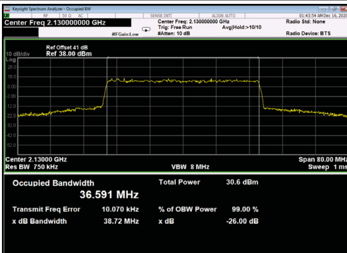
Figure 713: 256QAM 40MHz B.W.; 2130.0MHz, 60kHz - Output
