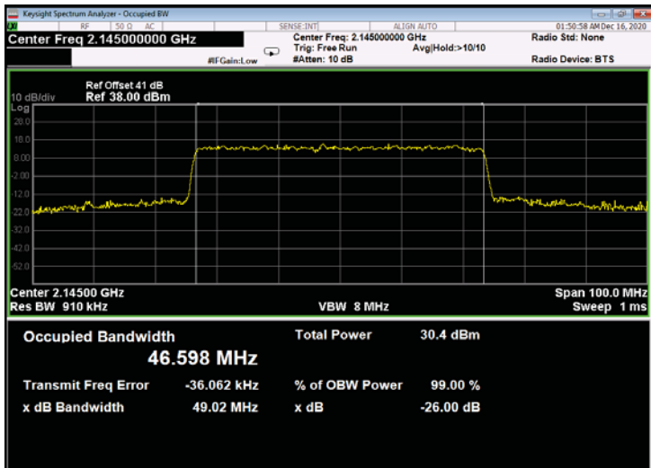
Figure 725: 256QAM 50MHz B.W.; 2145.0MHz, 60kHz - Output
