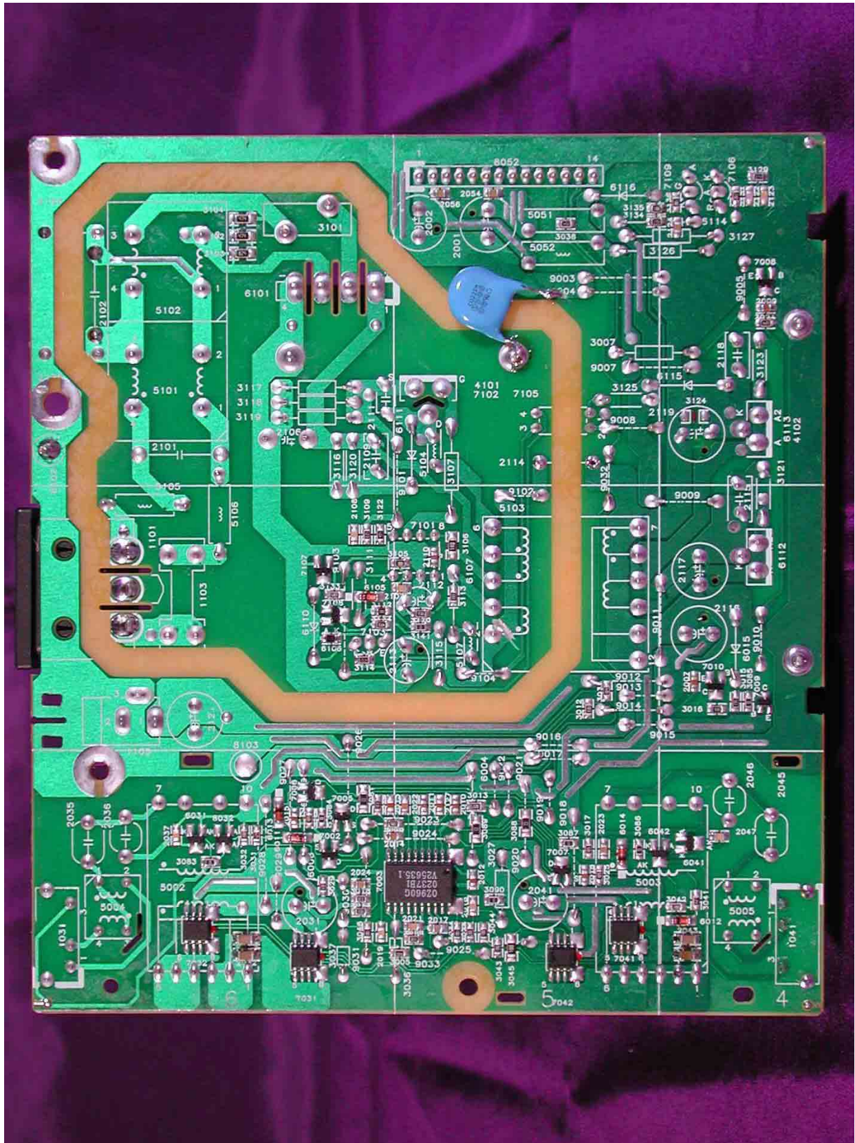
PCB Layout (QDI Panel)
