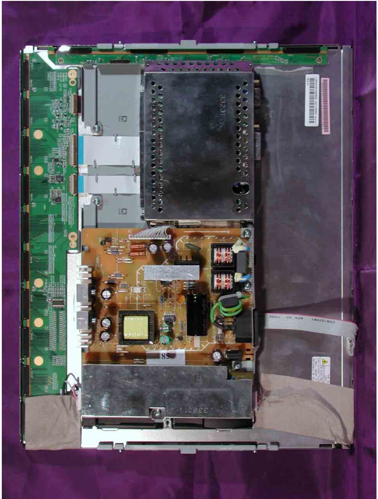
Assembly w/o Back Cover (QDI Panel)
