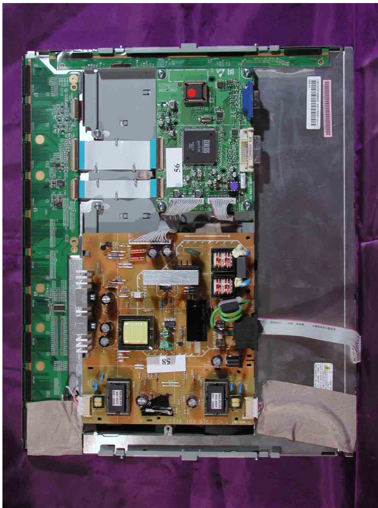
Assembly w/o Shielding Cover (QDI Panel)
