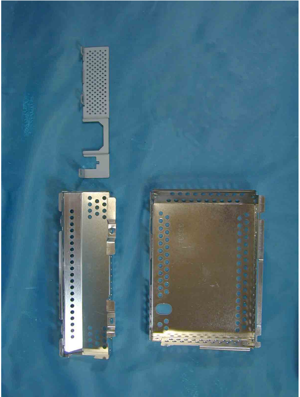
Shielding Cover (AU Panel)
