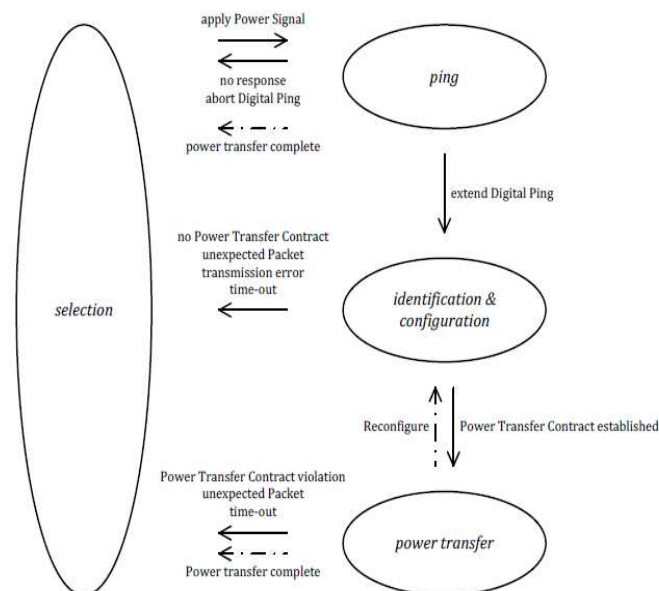
Fig.3 : Functional overview
