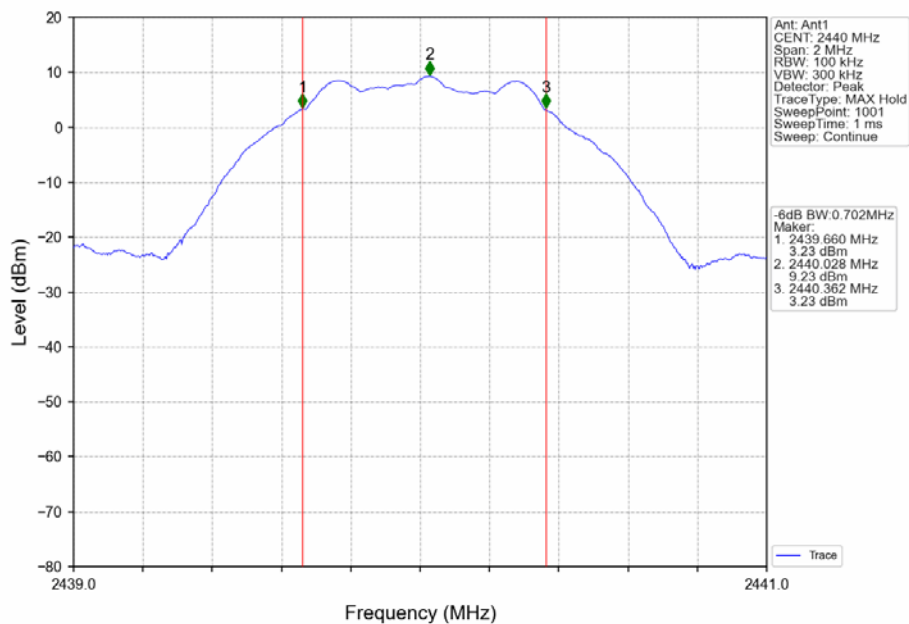
1M_MCH_2440MHz_Ant1_NTNV
