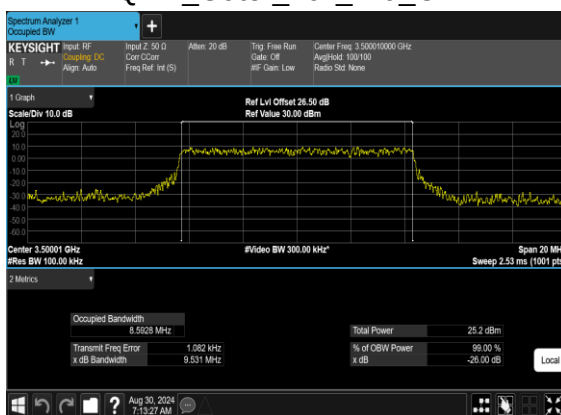
N77(10M)_CP-OFDM_256 QAM_Outer_Full_Mid_CH
