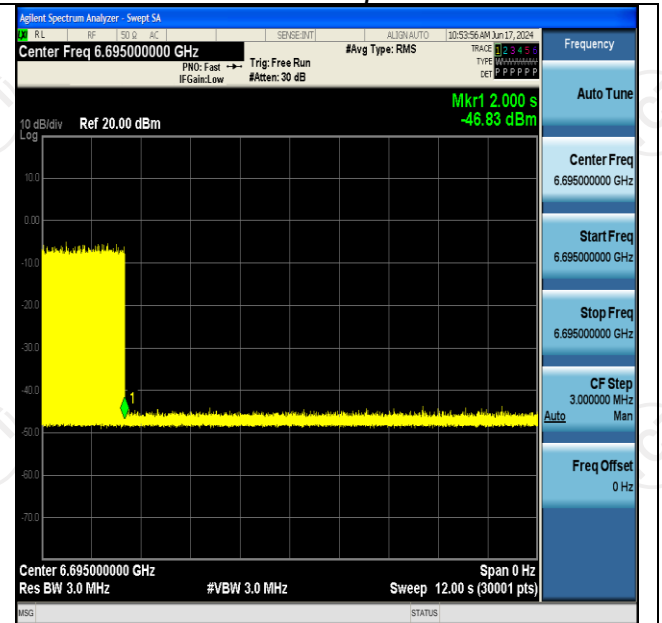
11AX20SISO-Ant2-6695-Center-6695-OFF-PASS
