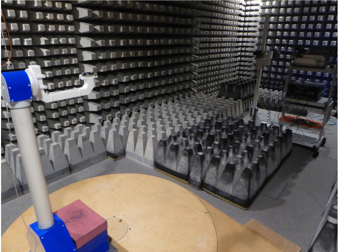
Test setup fully anechoic chamber 12 – 18 GHz
