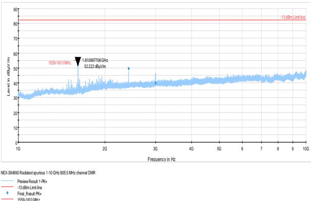
Figure 8.3-24: Radiated spurious above 1GHz 805.5 MHz DMR
