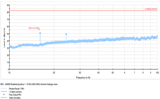
Figure 8.3-20: Radiated spurious above 1GHz 805.5 MHz analogue voice
