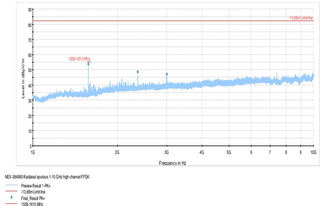
Figure 8.3-21 Radiated spurious above 1GHz high channel 787.9875 MHz FFSK
