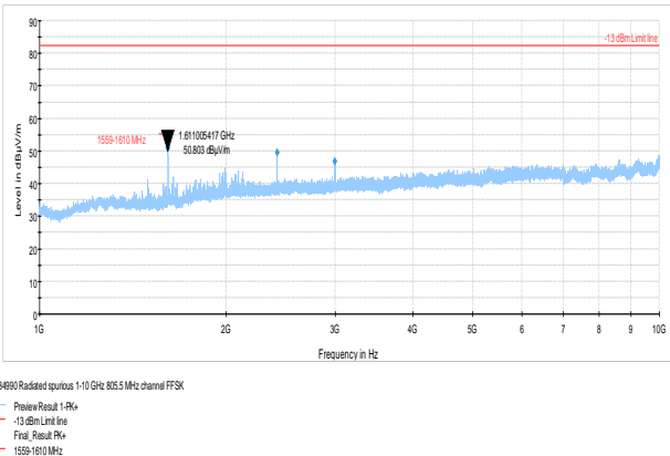
Figure 8.3-22: Radiated spurious above 1GHz 805.5 MHz FFSK
