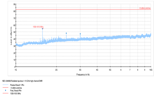
Figure 8.3-23 Radiated spurious above 1GHz high channel 787.9875 MHz DMR
