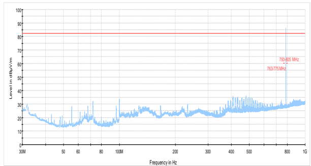
Figure 8.3-7: Radiated spurious below 1GHz high channel 787.9875 MHz analogue voice
