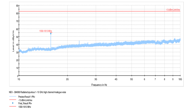
Figure 8.3-19: Radiated spurious above 1GHz high channel 787.9875 MHz analogue voice
