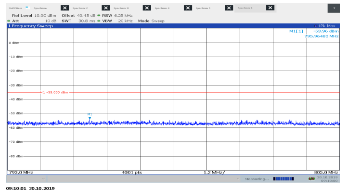
Figure 8.2-2: Spurious emissions within 793-805 MHz protection band for high channel 787.9875 MHz analogue FM
