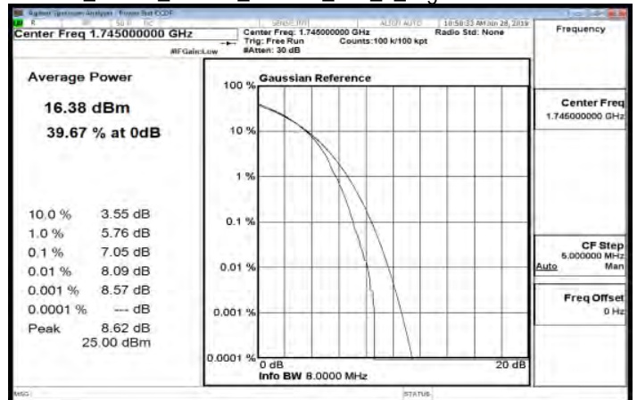
LTE_Band4_20MHz_16QAM_100_0_HighCH20300-1745
