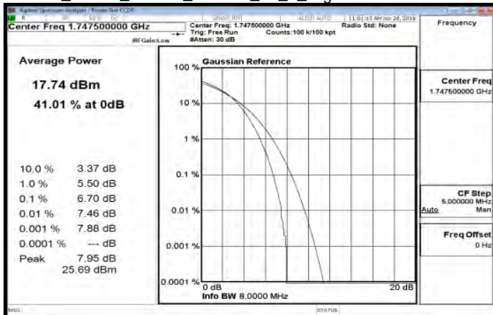
LTE_Band4_15MHz_16QAM_75_0_HighCH20325-1747.5
