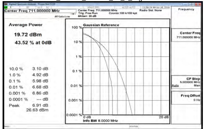
LTE_Band12_10MHz_16QAM_50_0_HighCH23130-711
