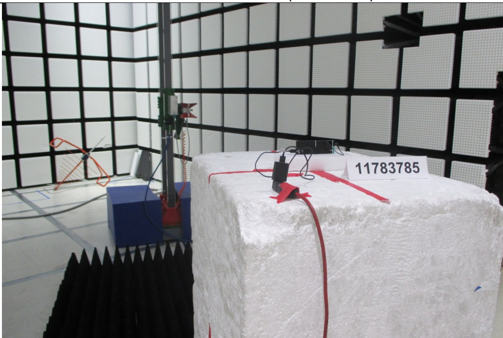
RADIATED BACK PHOTO (ABOVE 1 GHz)
