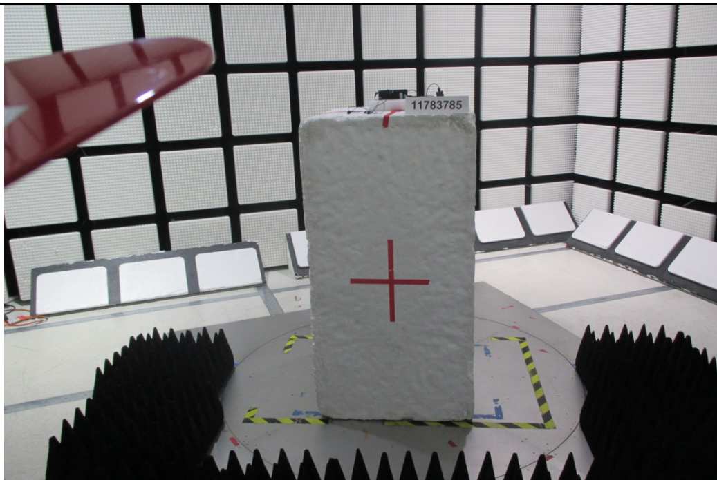
RADIATED FRONT PHOTO (ABOVE 1 GHz)
