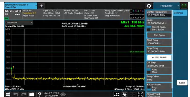
Band2-9262-4-0.15~30MHz-PASS
