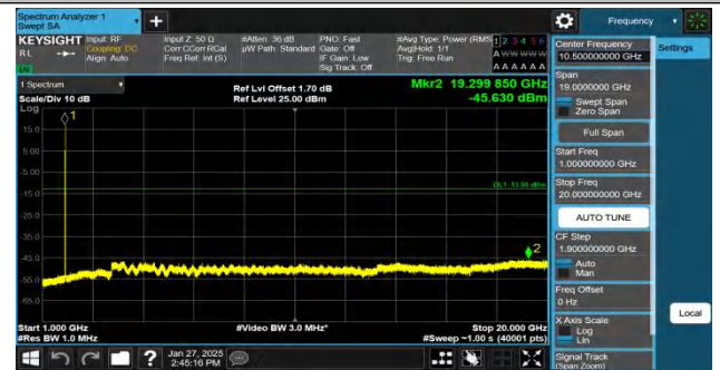
Band2-9262-3-1000~20000MHz-PASS
