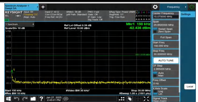
Band2-9262-3-0.15~30MHz-PASS
