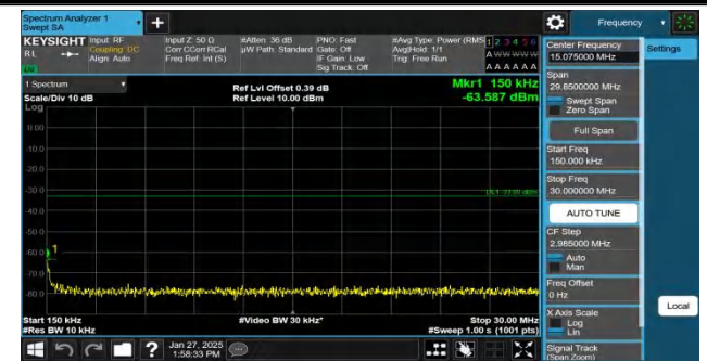
Band2-9538-0.15~30MHz-PASS
