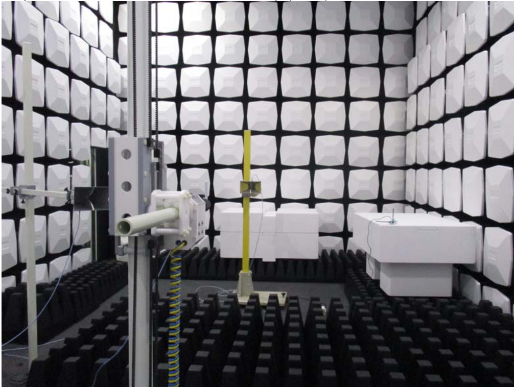
Description : Radiated Emission Test Setup (Horn)
