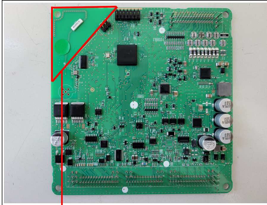
Receive Antenna
