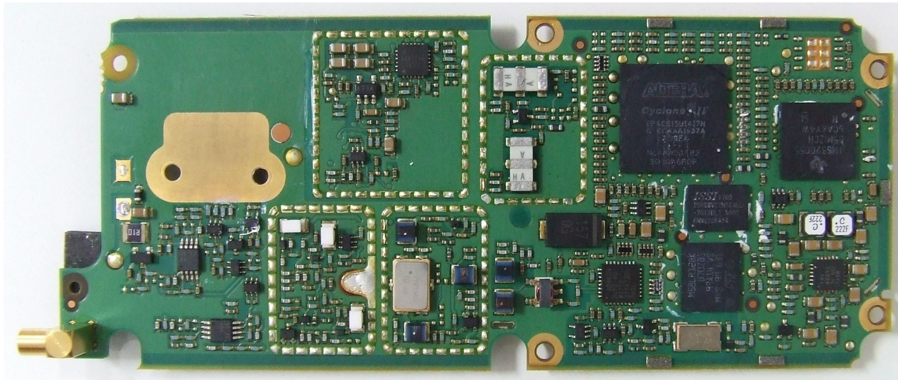
Photograph 05: Rx-Tx PCB - bottom (without shields)
