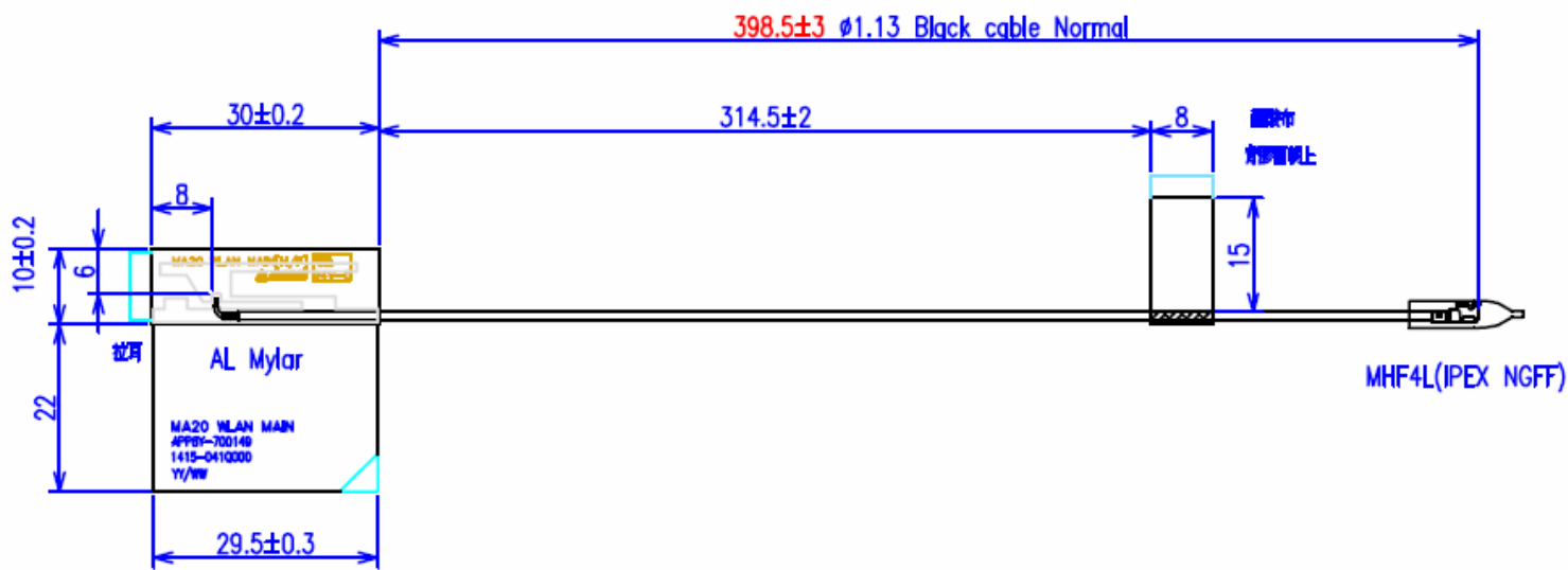
Tx1 Antenna Dimensioned Drawing:
