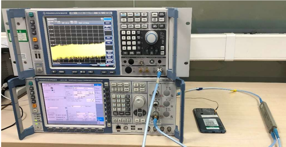
RF Conducted Test
