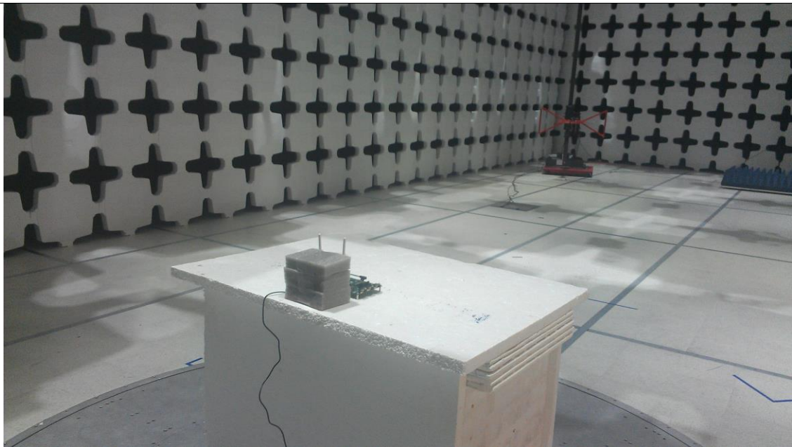
Radiated Emission Test Setup (below 1GHz) with Sleeve antenna: Sansei – Rear View
