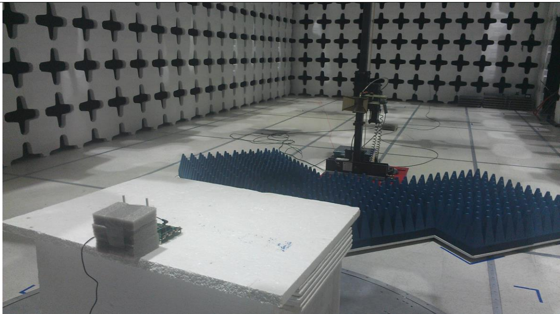
Radiated Emission Test Setup (above 1GHz) with Sleeve antenna: Sansei – Rear View
