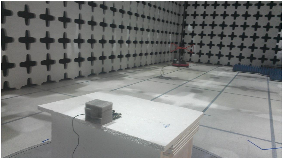
Radiated Emission Test Setup (below 1GHz) with Embedded antenna: Ethertronics – Rear View
