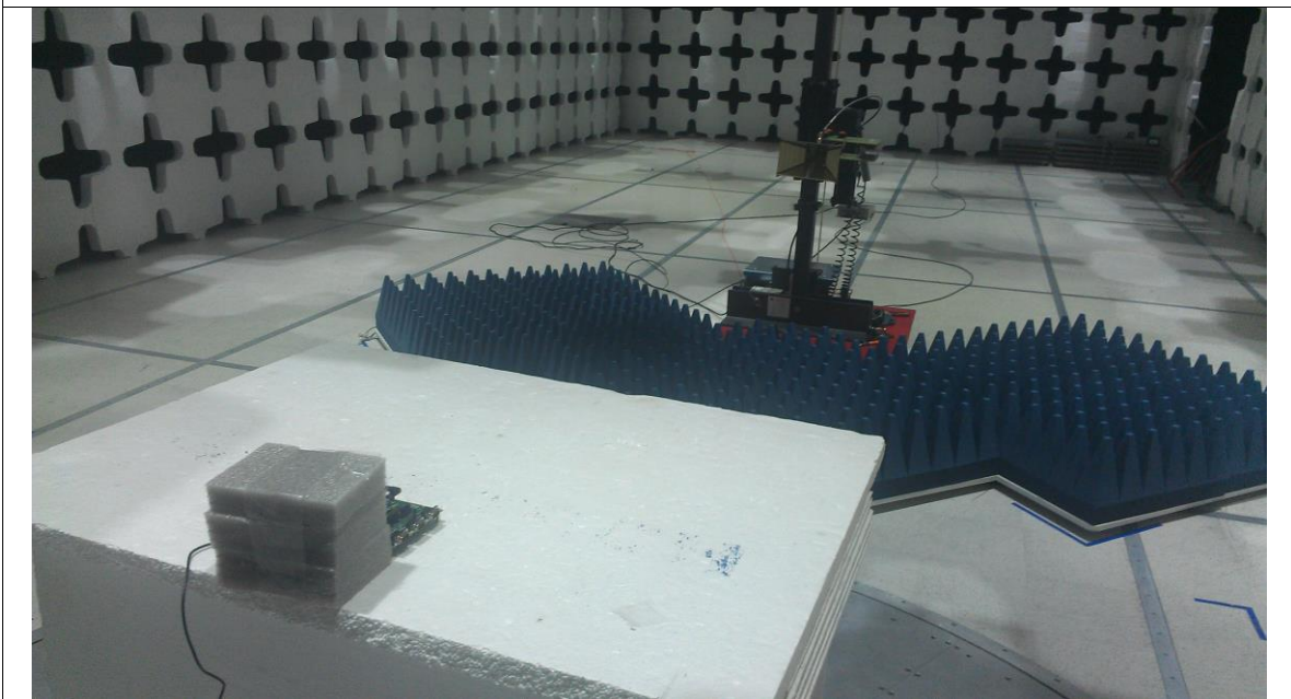
Radiated Emission Test Setup (above 1GHz) with Embedded antenna: Ethertronics – Rear View
