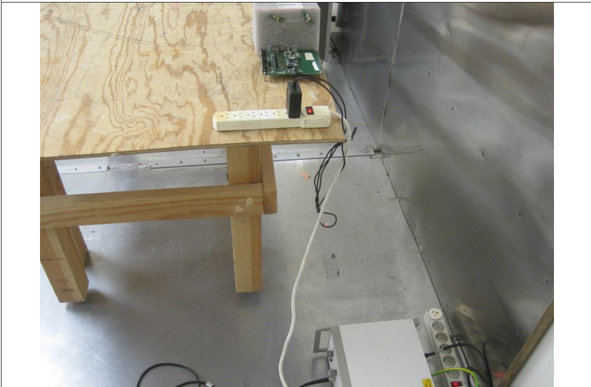
Conducted Emission Test Setup (below 1GHz) - Rear View
