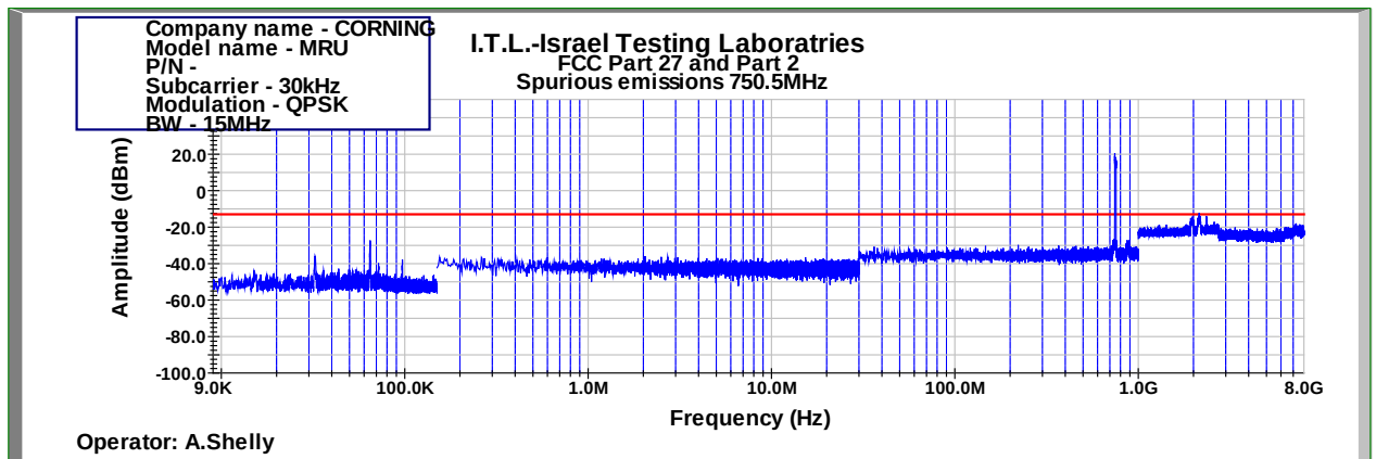
Figure 525: Spurious Emissions at Antenna Terminal QPSK 15MHz B.W.; 750.5MHz, 30kHz
