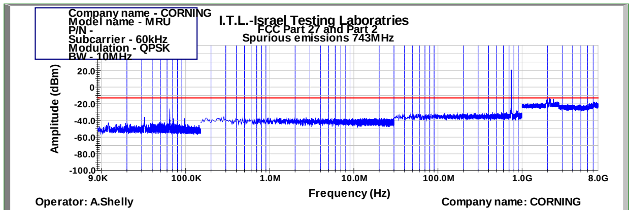
Figure 514: Spurious Emissions at Antenna Terminal QPSK 10MHz B.W.; 743.0MHz, 60kHz
