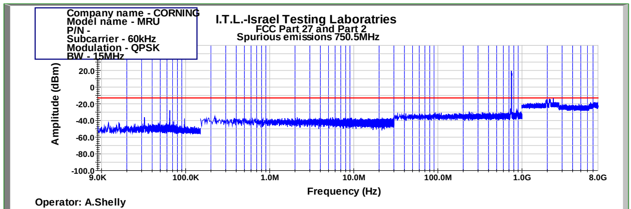
Figure 526: Spurious Emissions at Antenna Terminal QPSK 15MHz B.W.; 750.5MHz, 60kHz
