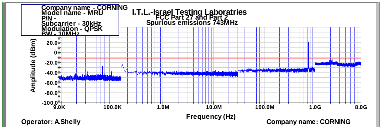
Figure 513: Spurious Emissions at Antenna Terminal QPSK 10MHz B.W.; 743.0MHz, 30kHz
