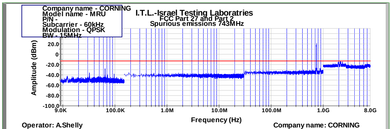
Figure 523: Spurious Emissions at Antenna Terminal QPSK 15MHz B.W.; 743.0MHz, 60kHz
