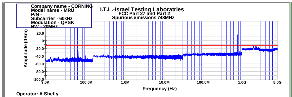
Figure 535: Spurious Emissions at Antenna Terminal QPSK 20MHz B.W.; 748.0MHz, 60kHz
