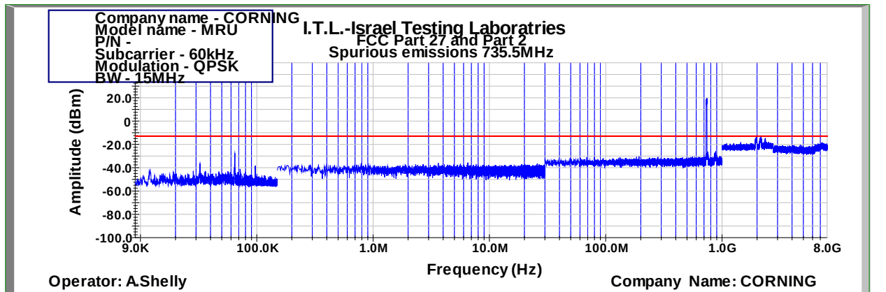
Figure 520: Spurious Emissions at Antenna Terminal QPSK 15MHz B.W.; 735.5MHz, 60kHz
