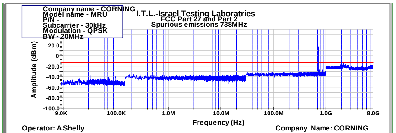
Figure 528: Spurious Emissions at Antenna Terminal QPSK 20MHz B.W.; 738.0MHz, 30kHz
