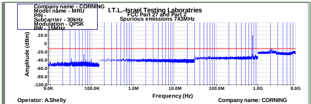
Figure 522: Spurious Emissions at Antenna Terminal QPSK 15MHz B.W.; 743.0MHz, 30kHz
