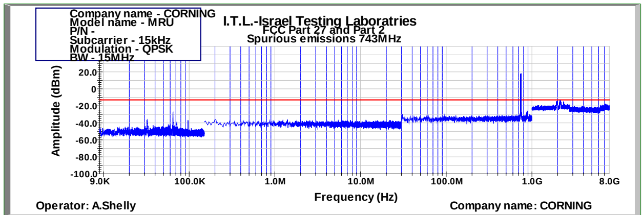
Figure 521: Spurious Emissions at Antenna Terminal QPSK 15MHz B.W.; 743.0MHz, 15kHz
