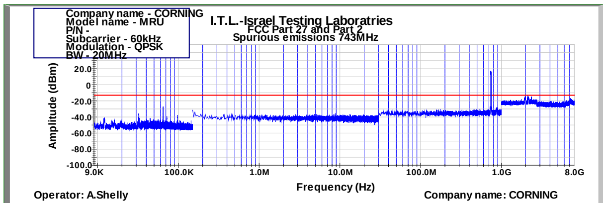
Figure 532: Spurious Emissions at Antenna Terminal QPSK 20MHz B.W.; 743.0MHz, 60kHz
