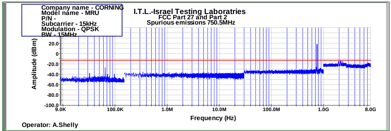
Figure 524: Spurious Emissions at Antenna Terminal QPSK 15MHz B.W.; 750.5MHz, 15kHz
