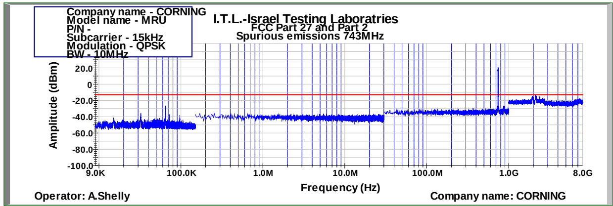
Figure 512: Spurious Emissions at Antenna Terminal QPSK 10MHz B.W.; 743.0MHz, 15kHz
