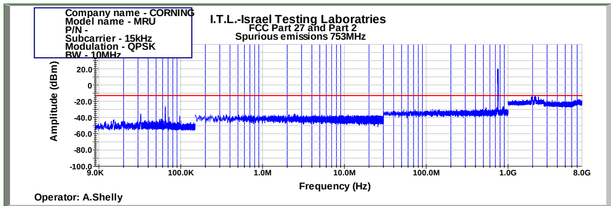
Figure 515: Spurious Emissions at Antenna Terminal QPSK 10MHz B.W.; 753.0MHz, 15kHz
