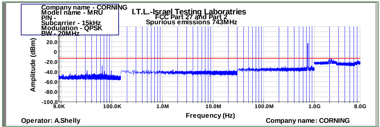
Figure 530: Spurious Emissions at Antenna Terminal QPSK 20MHz B.W.; 743.0MHz, 15kHz
