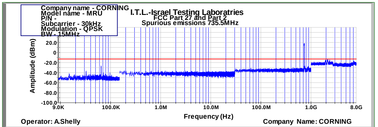
Figure 519: Spurious Emissions at Antenna Terminal QPSK 15MHz B.W.; 735.5MHz, 30kHz
