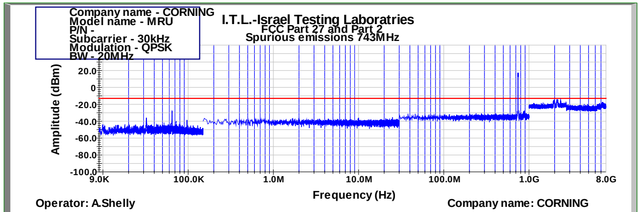
Figure 531: Spurious Emissions at Antenna Terminal QPSK 20MHz B.W.; 743.0MHz, 30kHz
