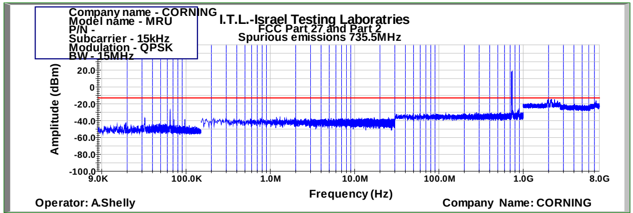
Figure 518: Spurious Emissions at Antenna Terminal QPSK 15MHz B.W.; 735.5MHz, 15kHz
