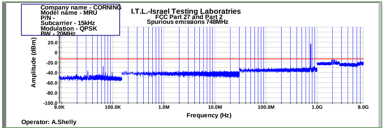
Figure 533: Spurious Emissions at Antenna Terminal QPSK 20MHz B.W.; 748.0MHz, 15kHz
