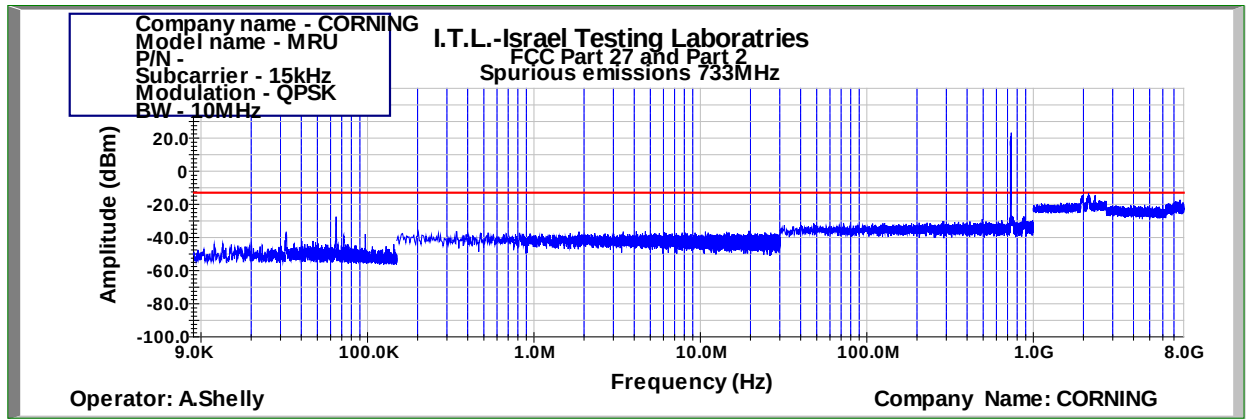
Figure 509: Spurious Emissions at Antenna Terminal QPSK 10MHz B.W.; 733.0MHz, 15kHz
