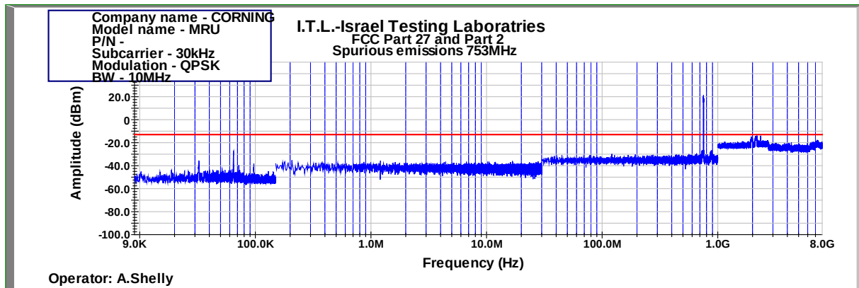
Figure 516: Spurious Emissions at Antenna Terminal QPSK 10MHz B.W.; 753.0MHz, 30kHz
