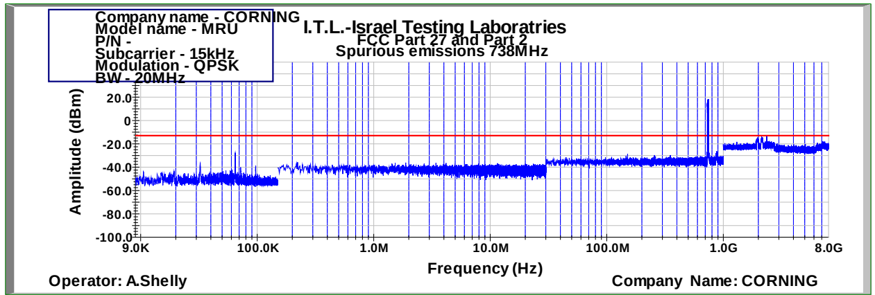
Figure 527: Spurious Emissions at Antenna Terminal QPSK 20MHz B.W.; 738.0MHz, 15kHz
