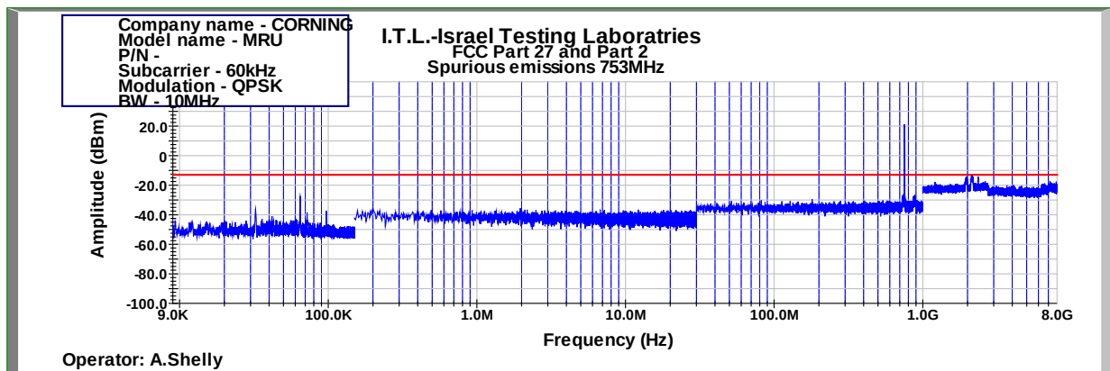
Figure 517: Spurious Emissions at Antenna Terminal QPSK 10MHz B.W.; 753.0MHz, 60kHz
