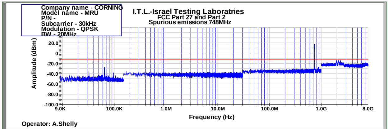
Figure 534: Spurious Emissions at Antenna Terminal QPSK 20MHz B.W.; 748.0MHz, 30kHz
