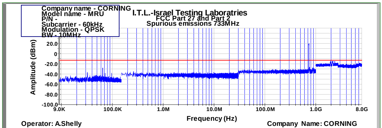
Figure 510: Spurious Emissions at Antenna Terminal QPSK 10MHz B.W.; 733.0MHz, 30kHz
