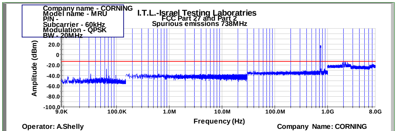
Figure 529: Spurious Emissions at Antenna Terminal QPSK 20MHz B.W.; 738.0MHz, 60kHz
