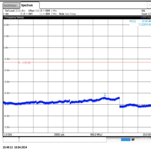
Band5-4132-2-1000~10000MHz-PASS
