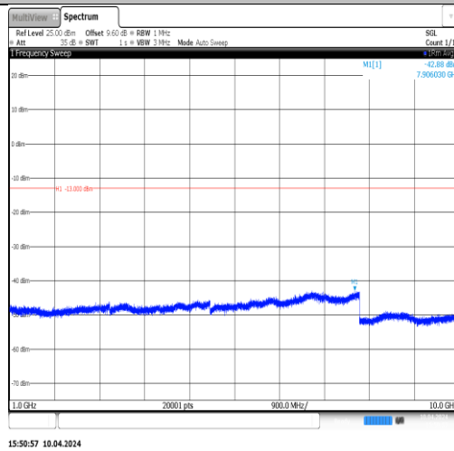
Band5-4132-3-1000~10000MHz-PASS
