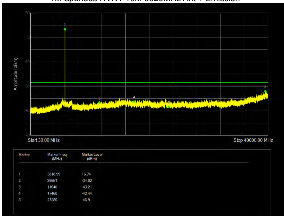
Tx. Spurious NVNT 10M 5820MHz Ant 1 Emission
