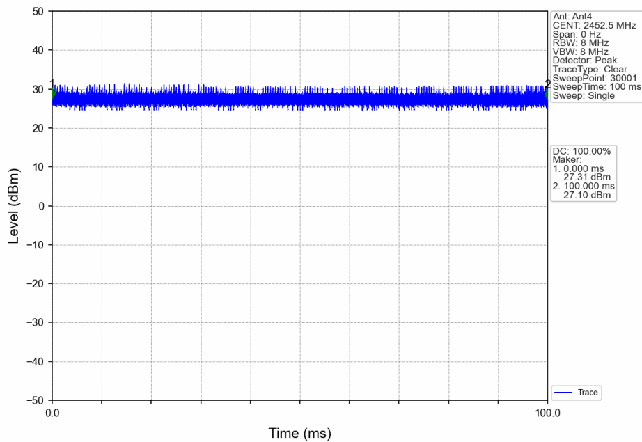
40M_HCH_2452.5MHz_Ant4_NTNV
