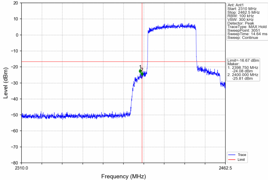
40M_LCH_2422.5MHz_Ant1_NTNV
