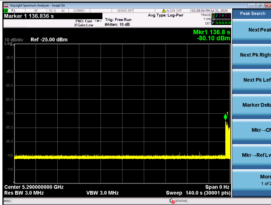
power-on cycle(5290MHz)
